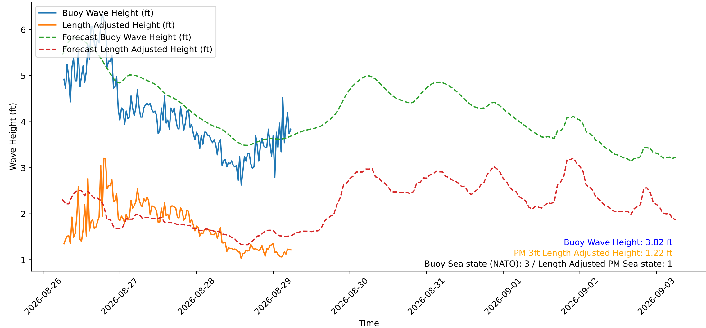
Wave Heights over Time for Green Beach at 2026-08-29 06:21:13
