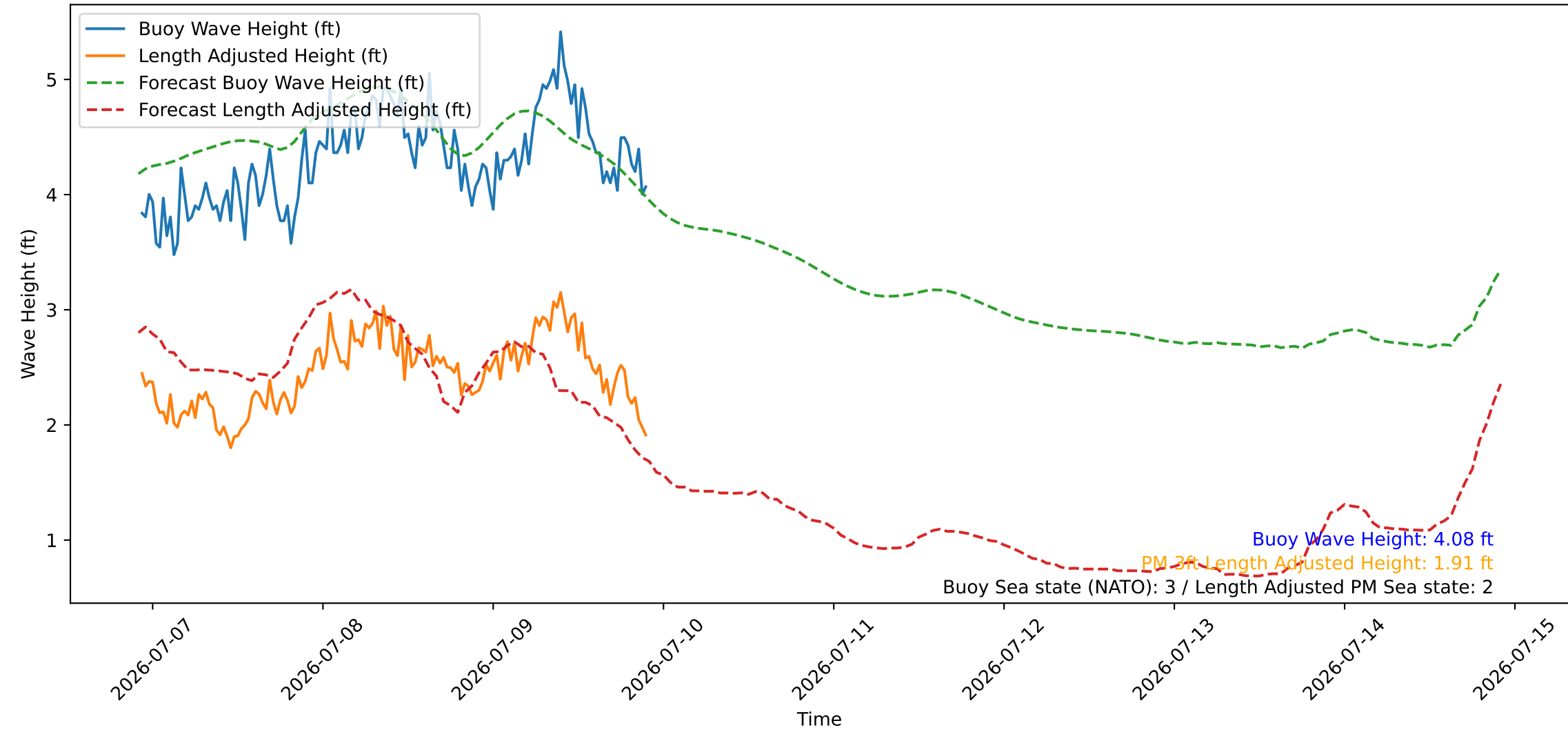
Wave Heights over Time for Oceanside Harbor at 2026-07-09 22:20:26
