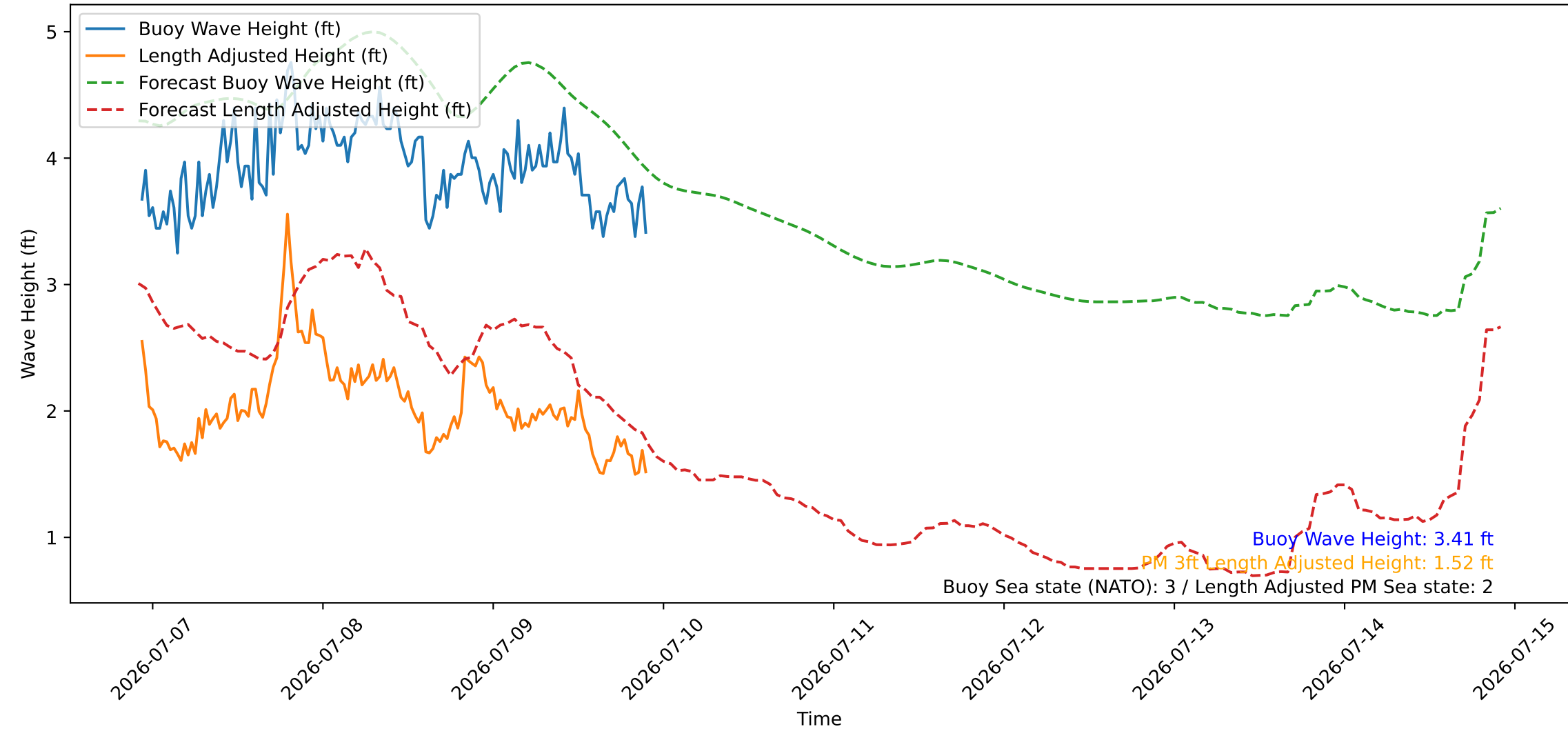
Wave Heights over Time for Green Beach at 2026-07-09 22:21:09
