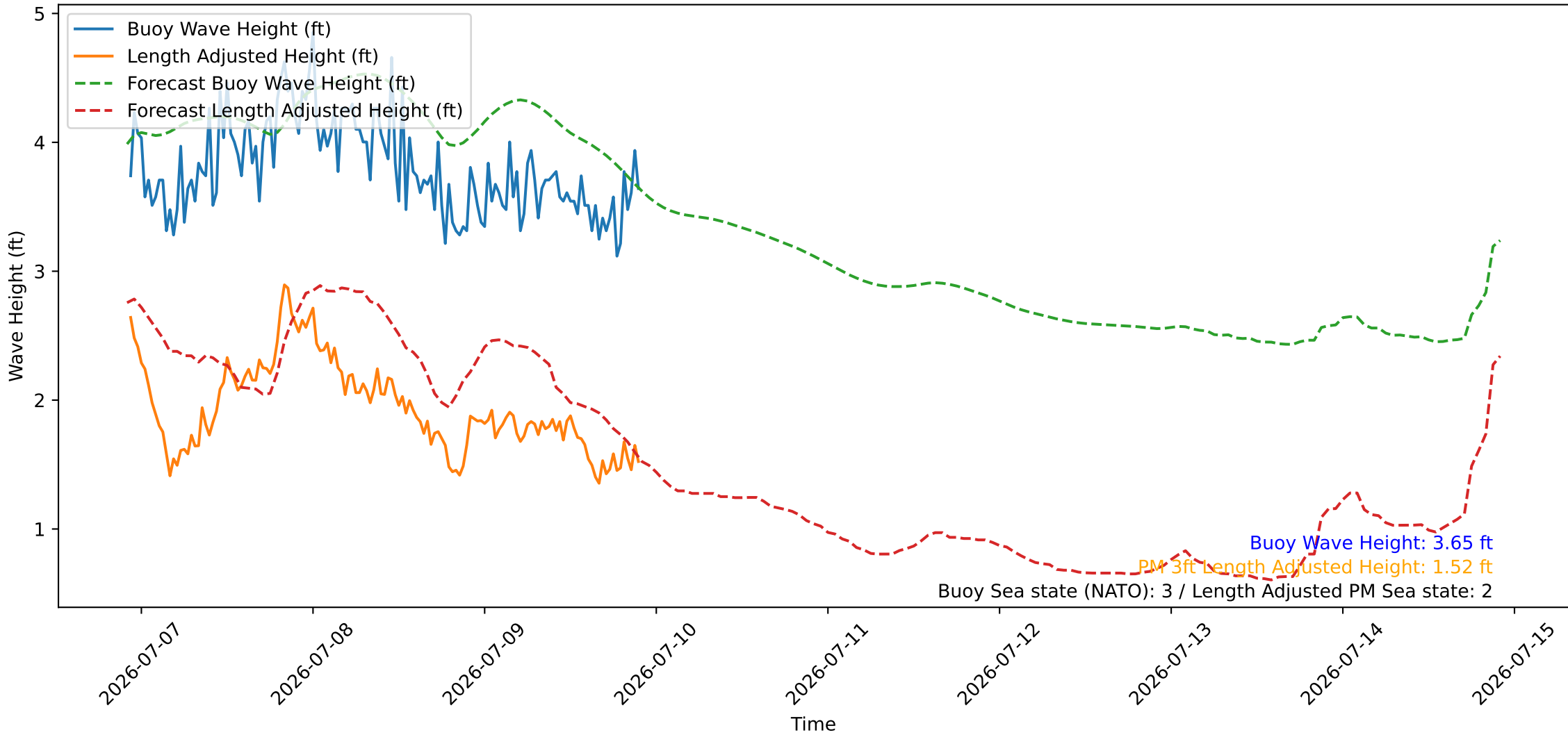
Wave Heights over Time for Red Beach at 2026-07-09 22:20:47
