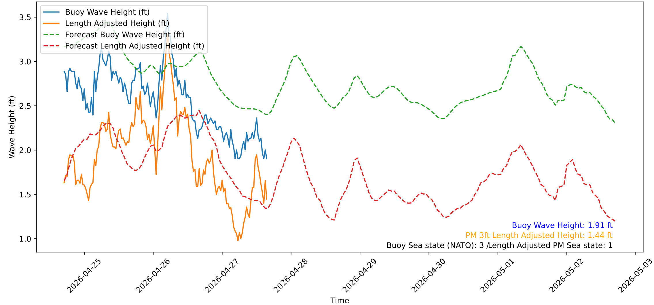
Wave Heights over Time for Red Beach at 2026-04-27 16:30:51
