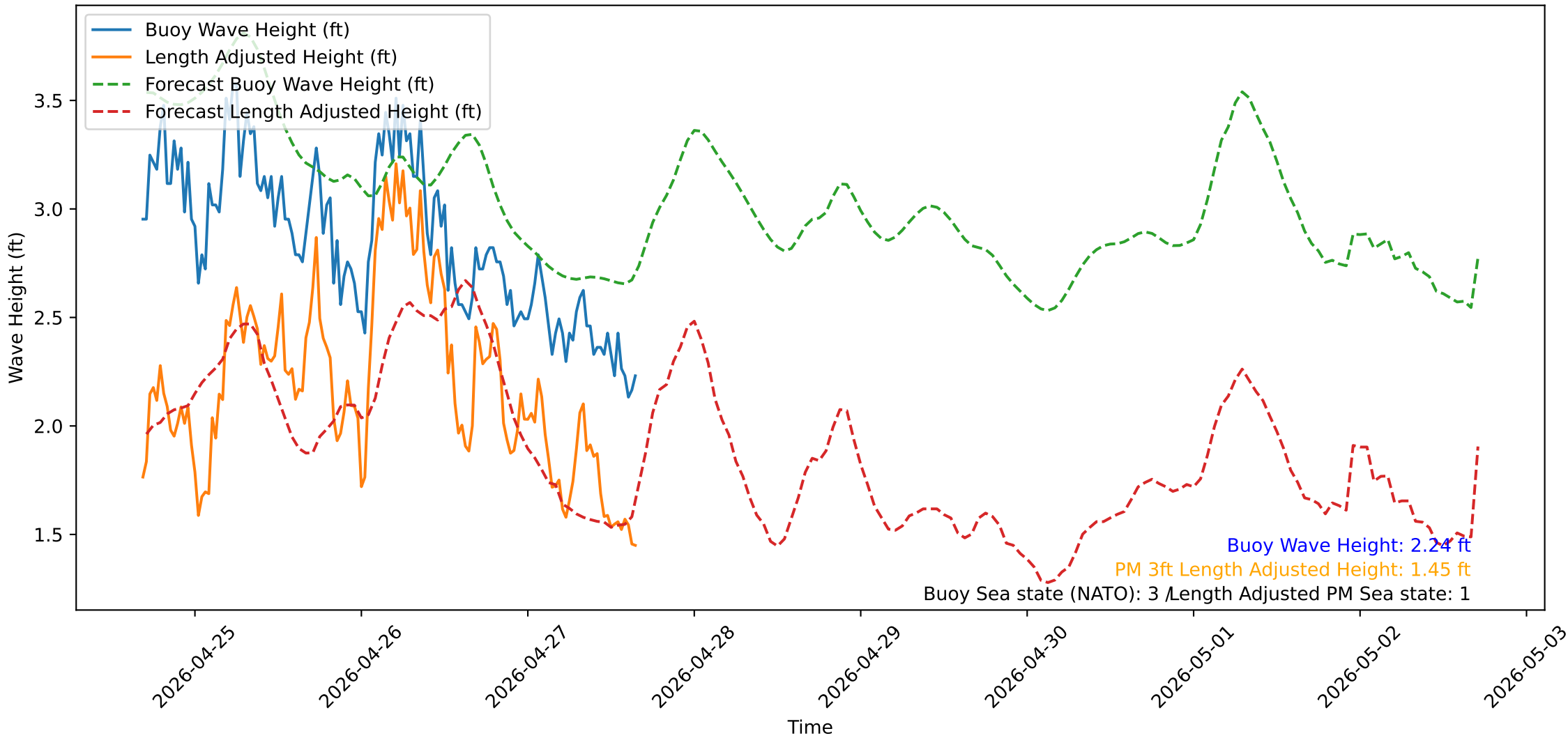
Wave Heights over Time for Green Beach at 2026-04-27 16:31:13
