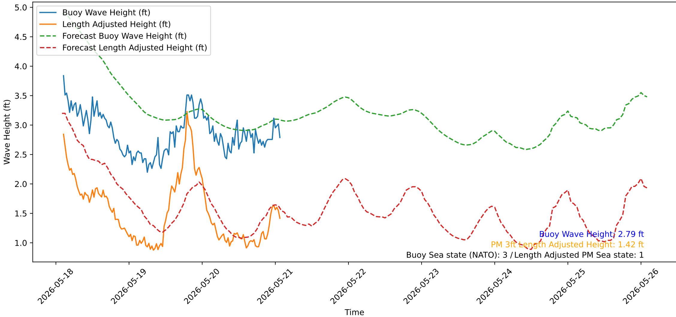
Wave Heights over Time for Oceanside Harbor at 2026-05-21 02:20:31
