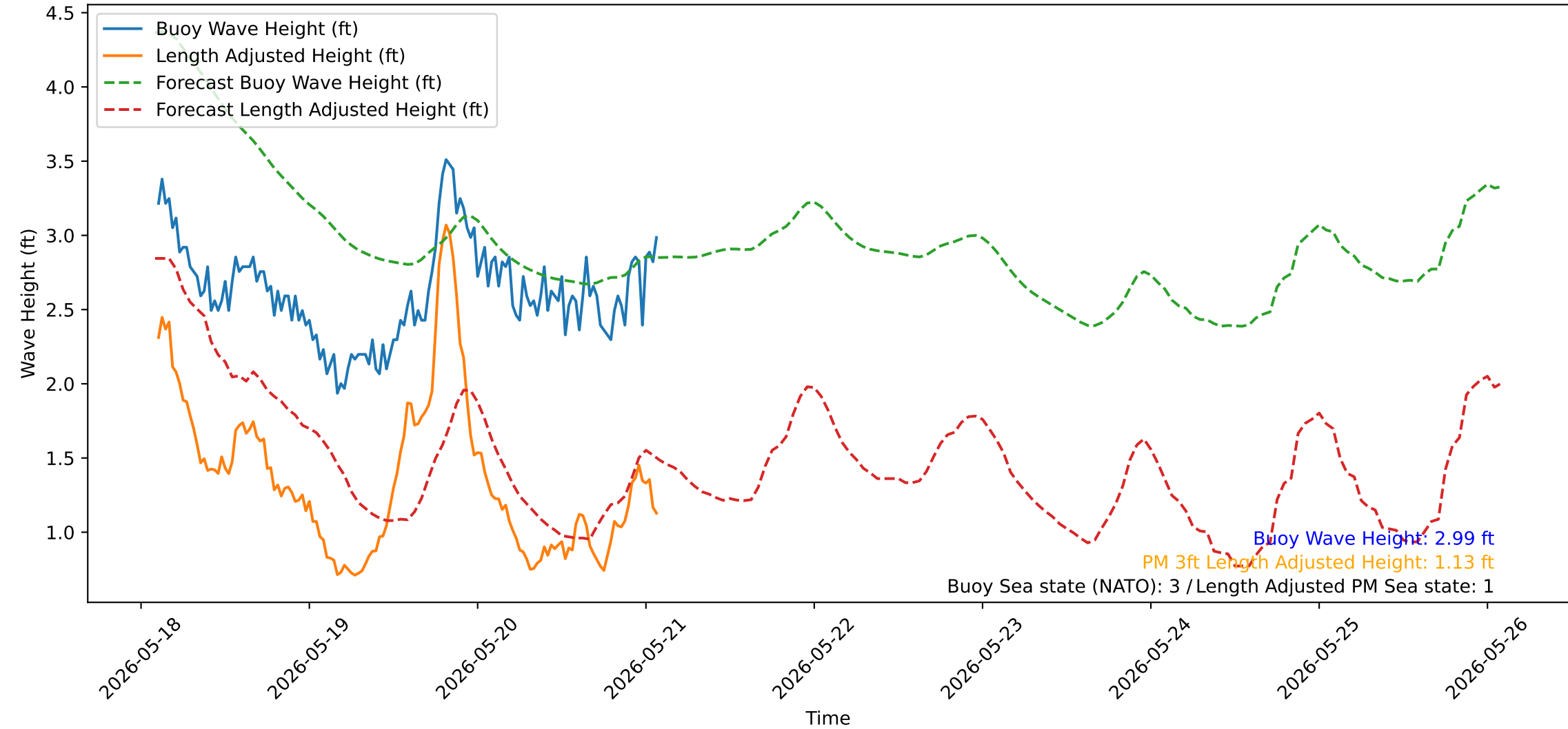
Wave Heights over Time for Red Beach at 2026-05-21 02:20:52
