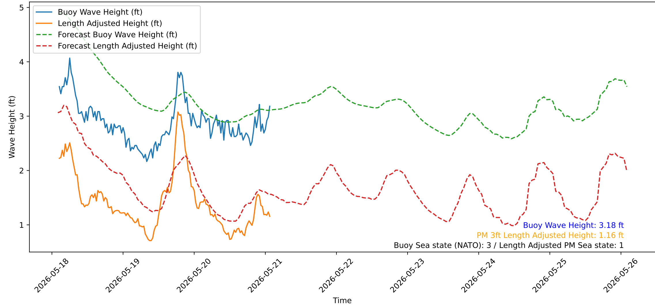
Wave Heights over Time for Green Beach at 2026-05-21 02:21:15
