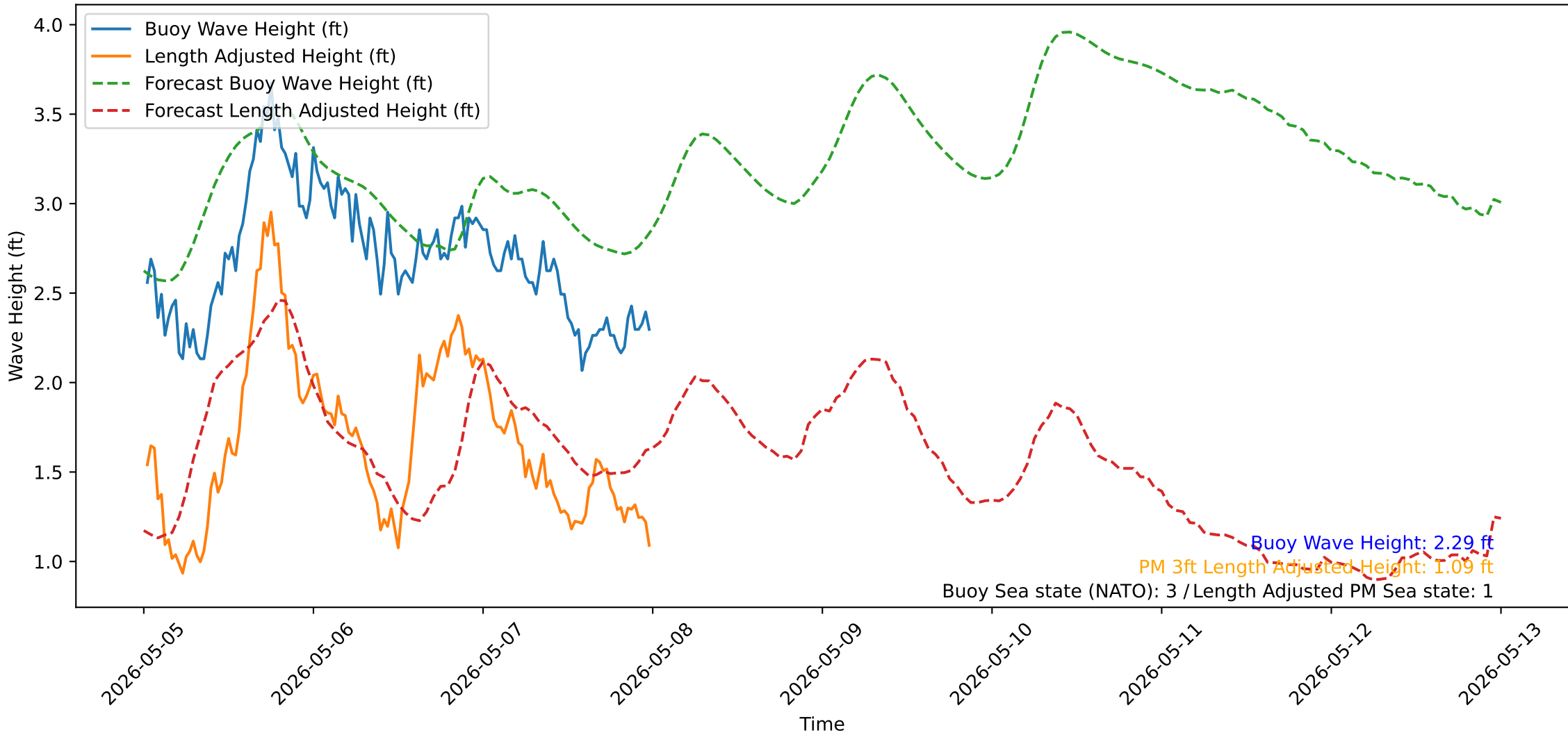
Wave Heights over Time for Green Beach at 2026-05-08 00:21:14
