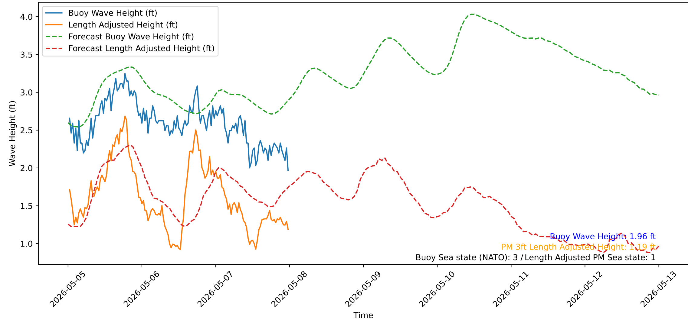
Wave Heights over Time for Oceanside Harbor at 2026-05-08 00:20:31
