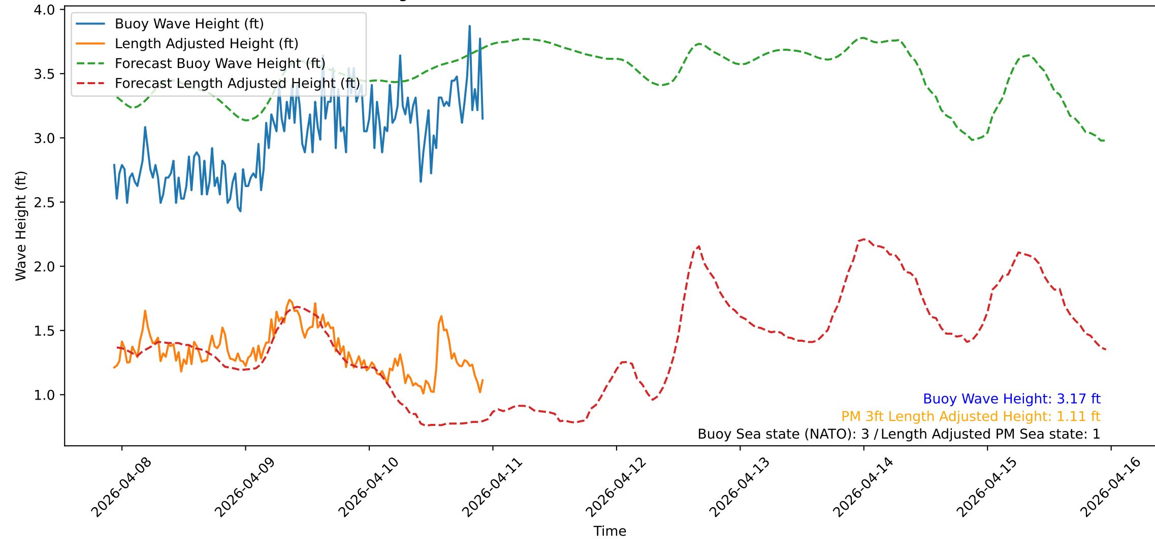
Wave Heights over Time for Oceanside Harbor at 2026-04-10 22:30:32
