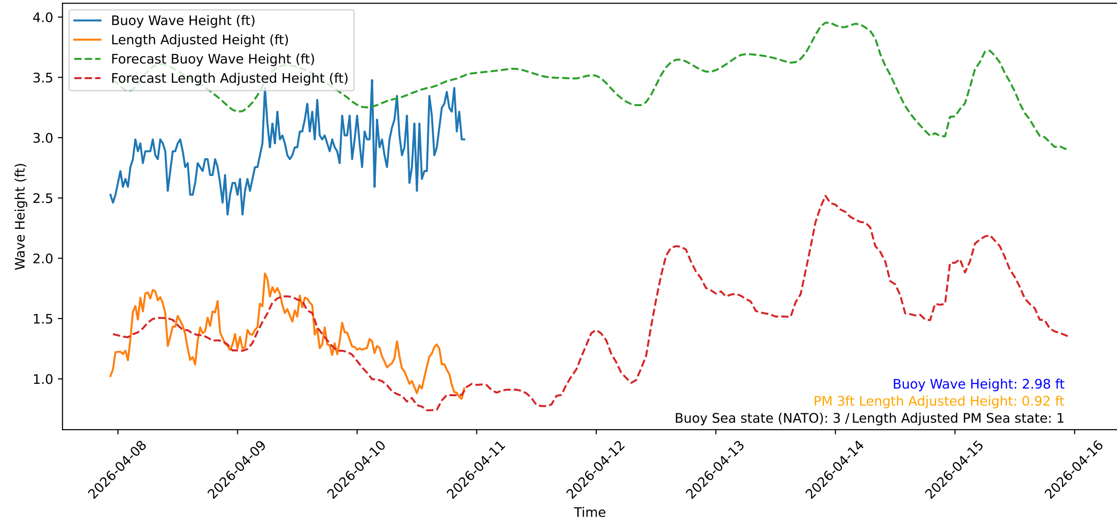
Wave Heights over Time for Green Beach at 2026-04-10 22:31:12
