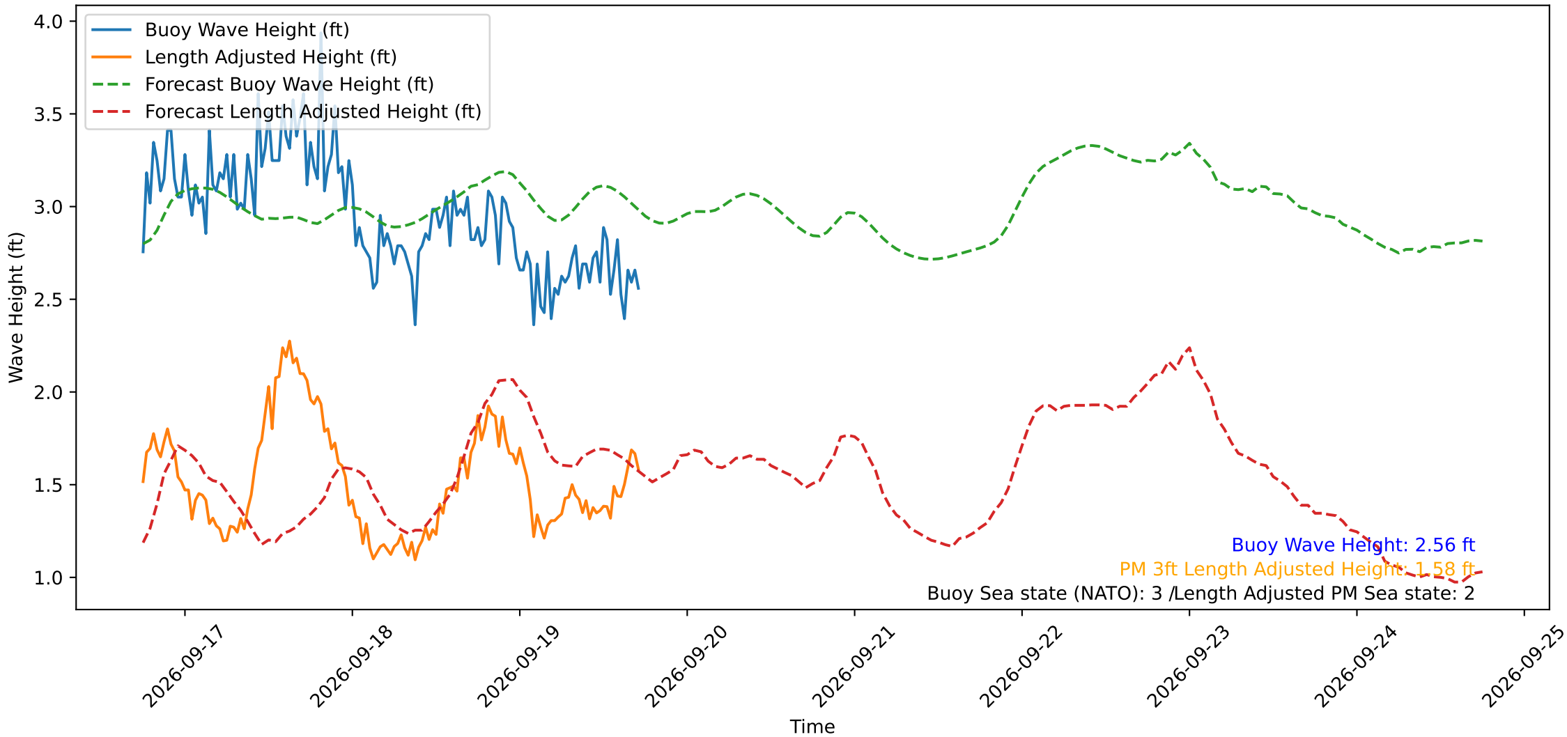
Wave Heights over Time for Oceanside Harbor at 2026-09-19 18:10:30
