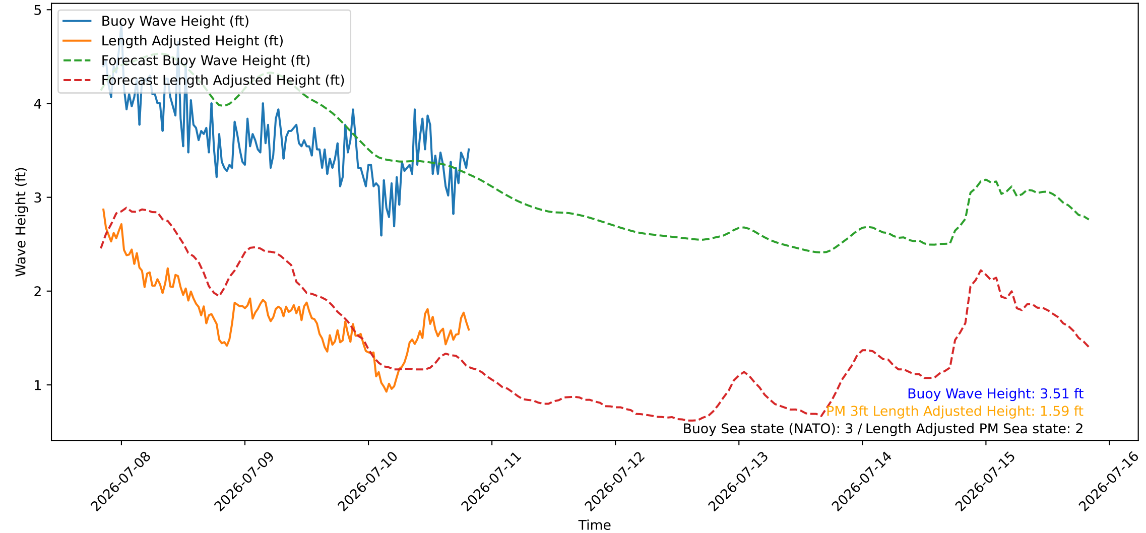
Wave Heights over Time for Red Beach at 2026-07-10 20:10:45
