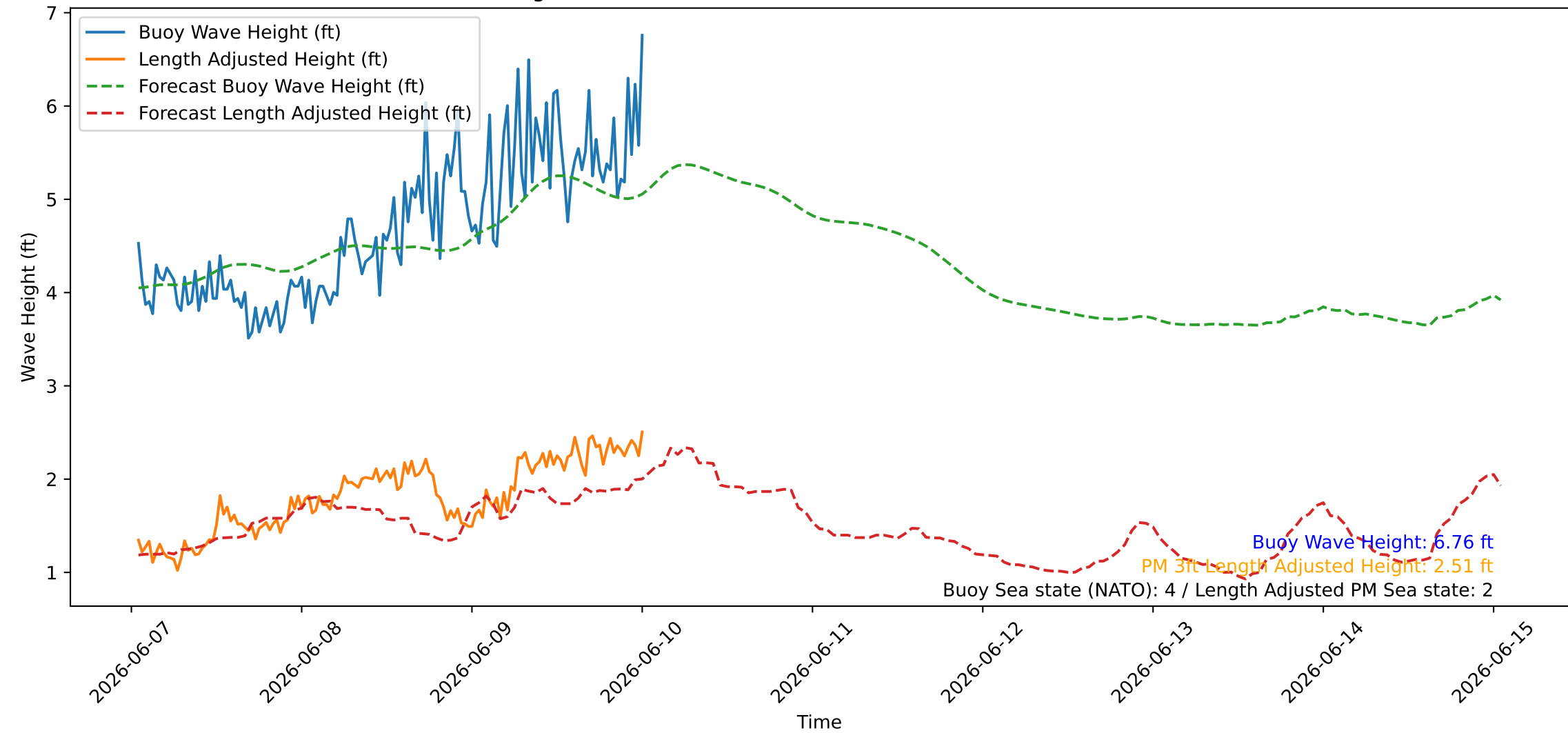
Wave Heights over Time for Oceanside Harbor at 2026-06-10 00:50:26
