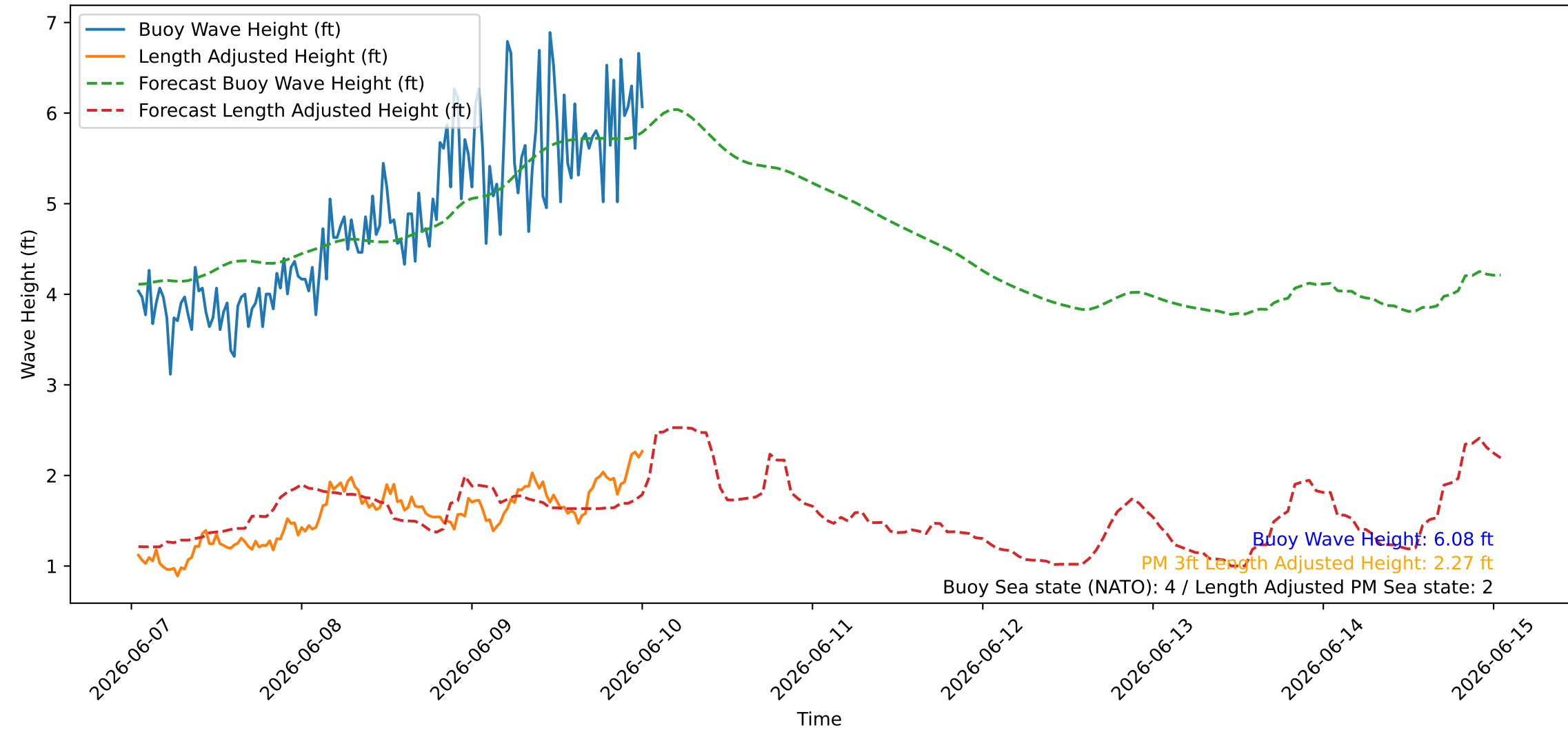
Wave Heights over Time for Green Beach at 2026-06-10 00:51:11
