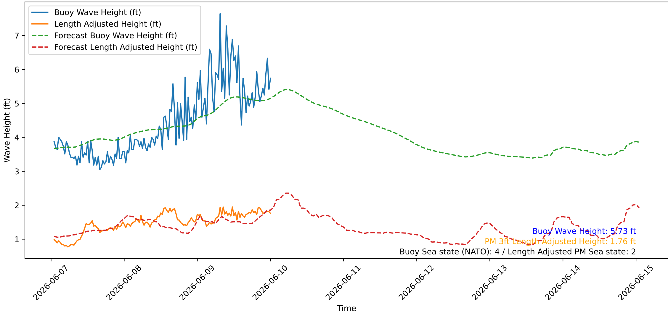
Wave Heights over Time for Red Beach at 2026-06-10 00:50:47
