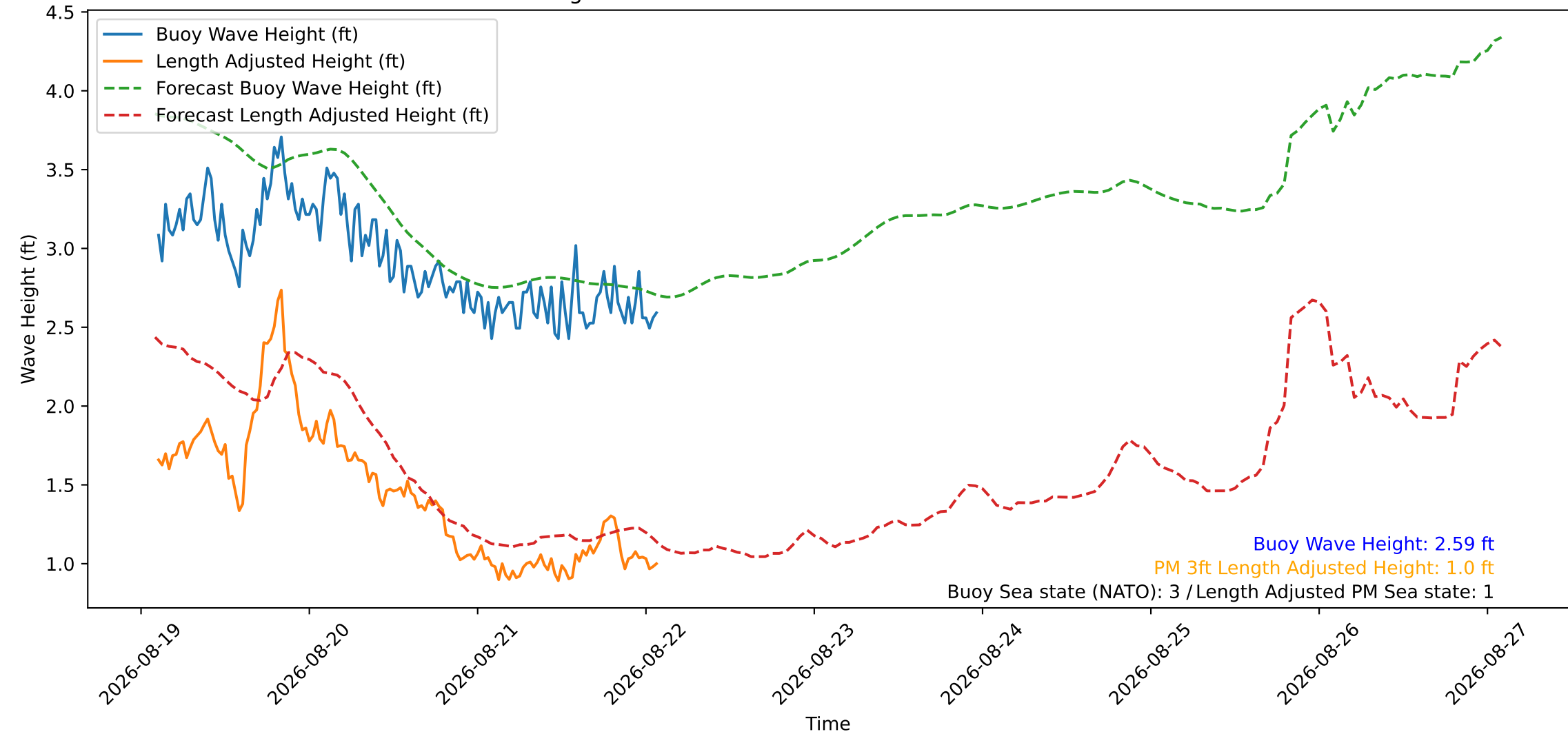
Wave Heights over Time for Green Beach at 2026-08-22 02:21:14
