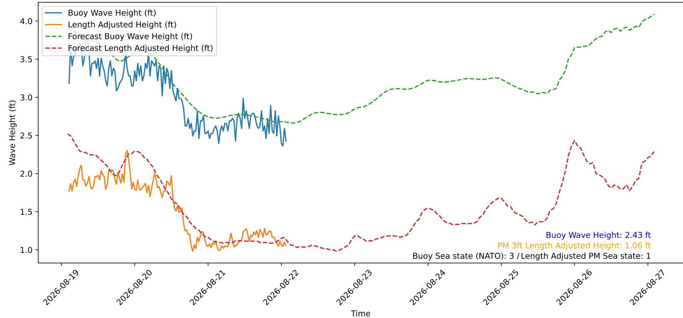
Wave Heights over Time for Oceanside Harbor at 2026-08-22 02:20:30
