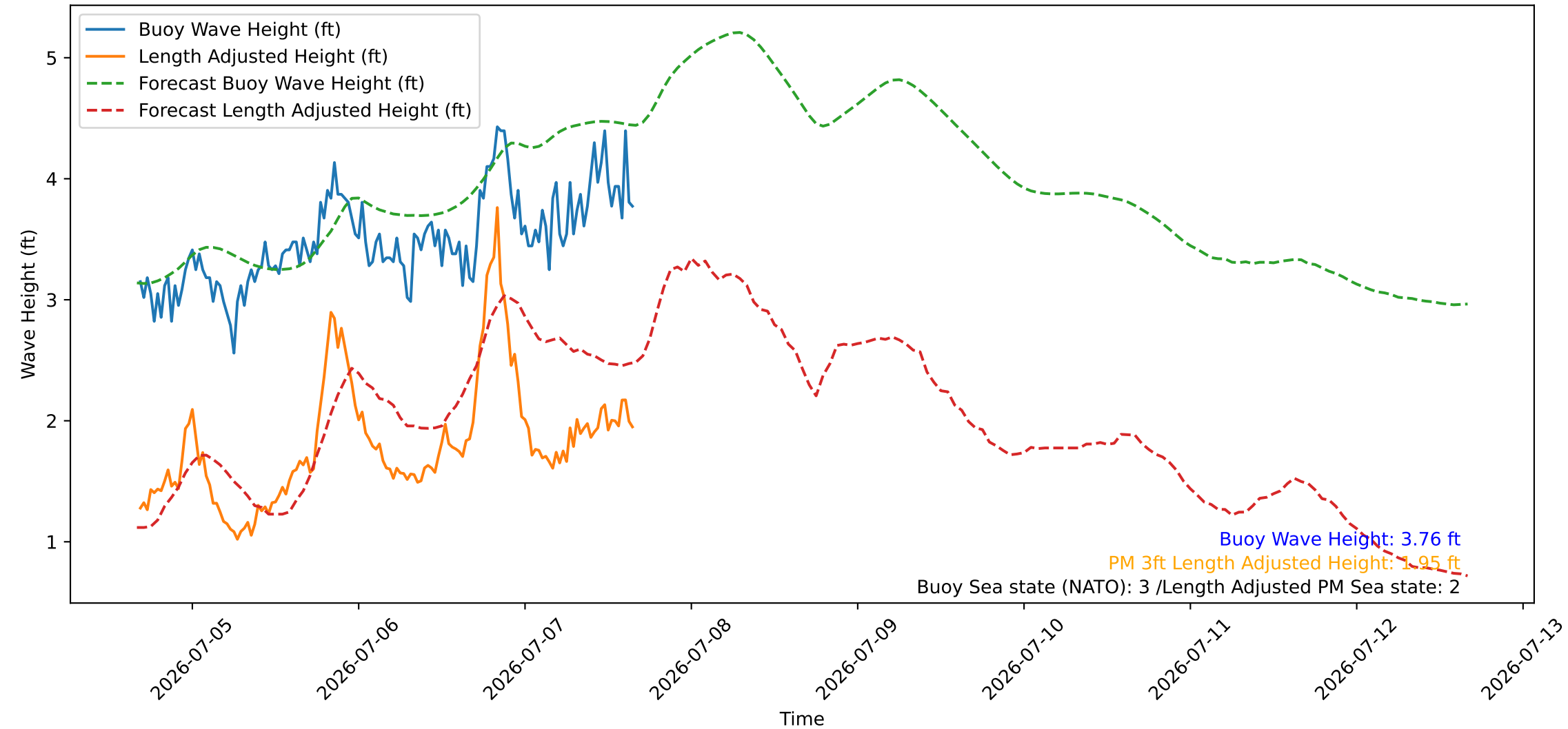
Wave Heights over Time for Green Beach at 2026-07-07 16:21:10
