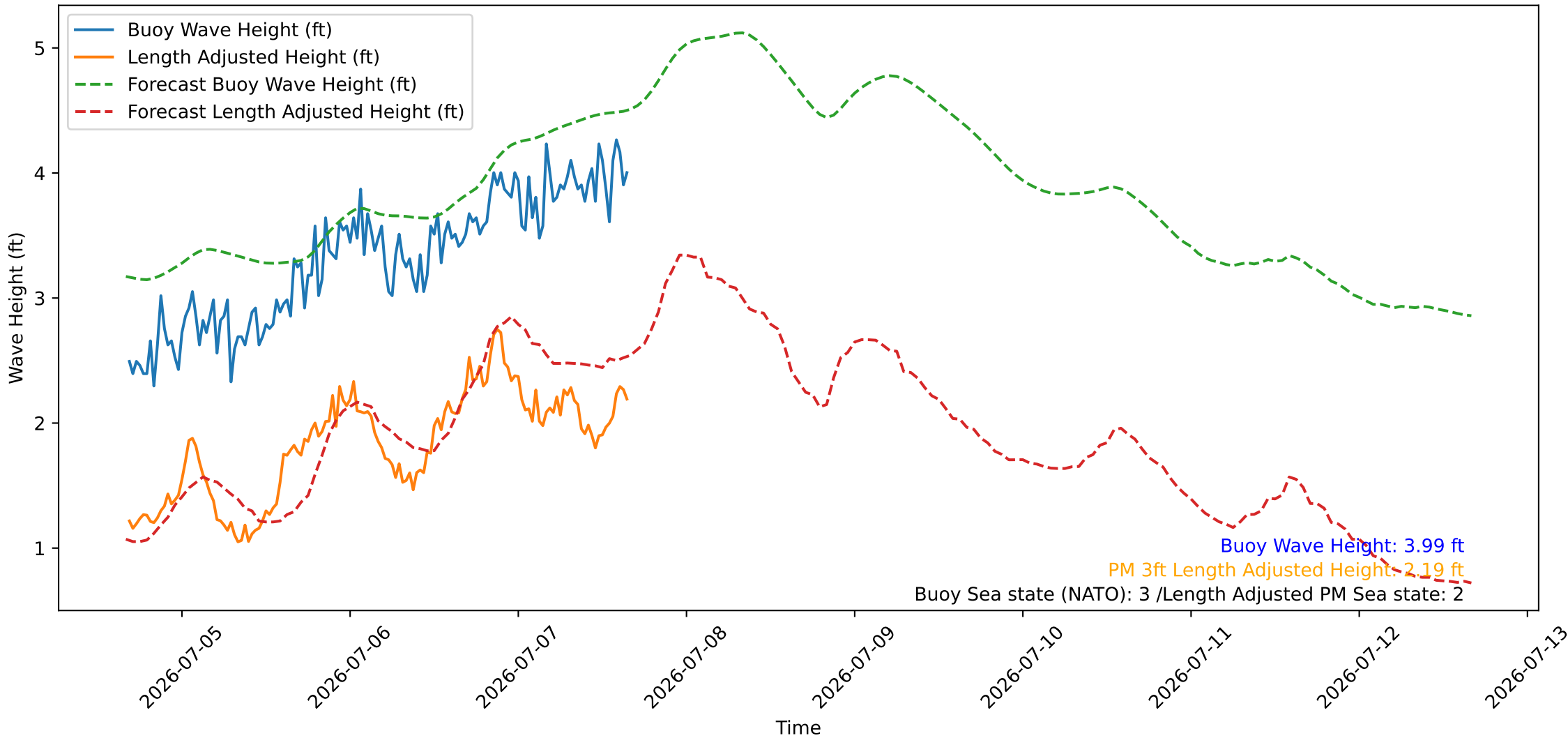
Wave Heights over Time for Oceanside Harbor at 2026-07-07 16:20:26
