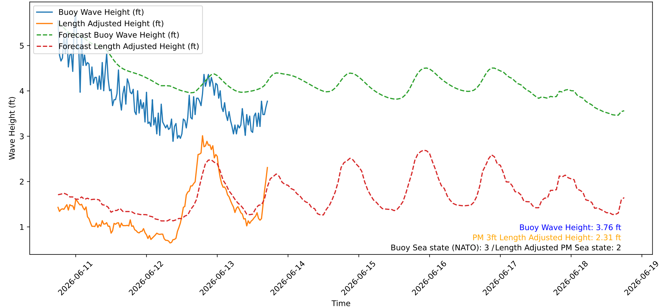
Wave Heights over Time for Green Beach at 2026-06-13 17:51:09
