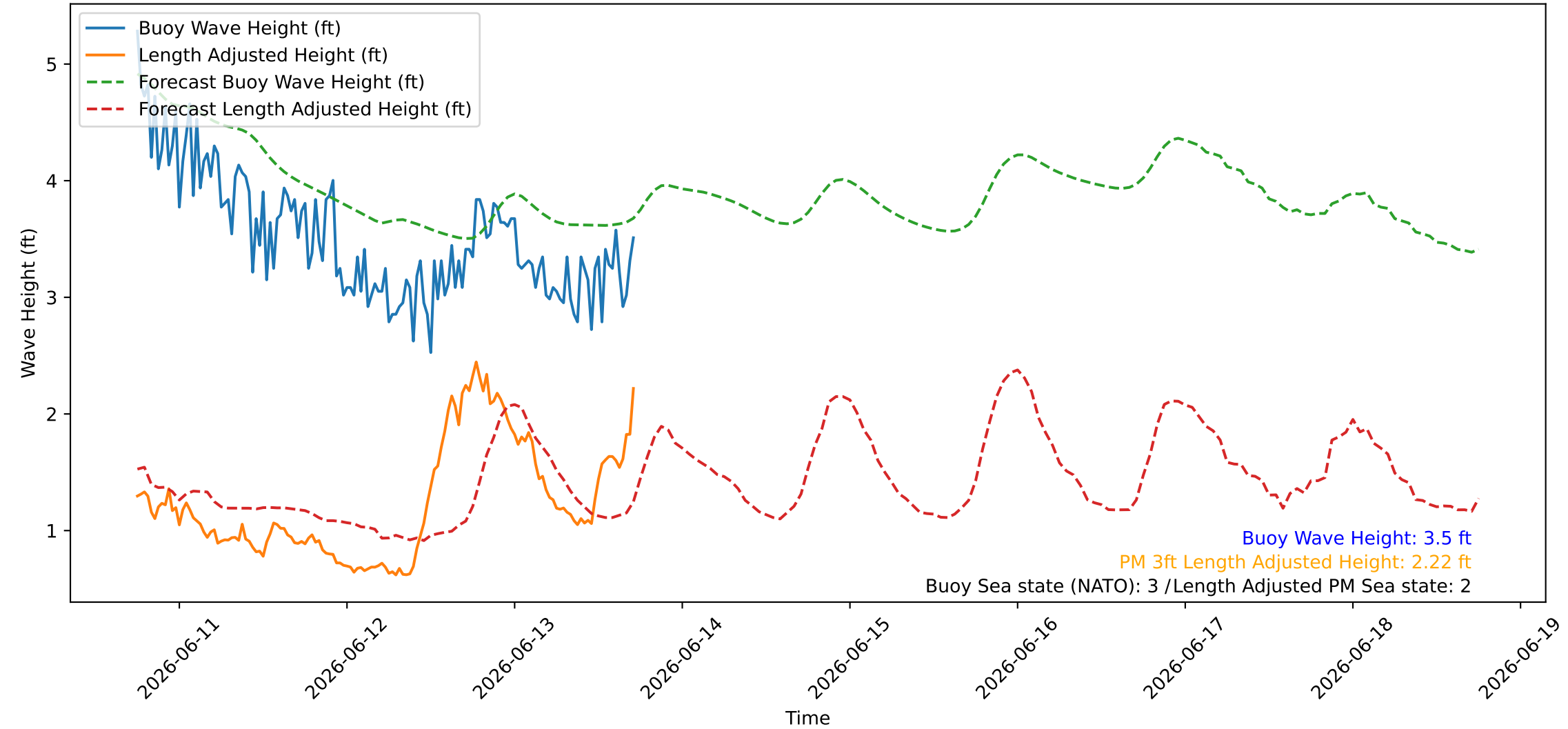
Wave Heights over Time for Red Beach at 2026-06-13 17:50:47
