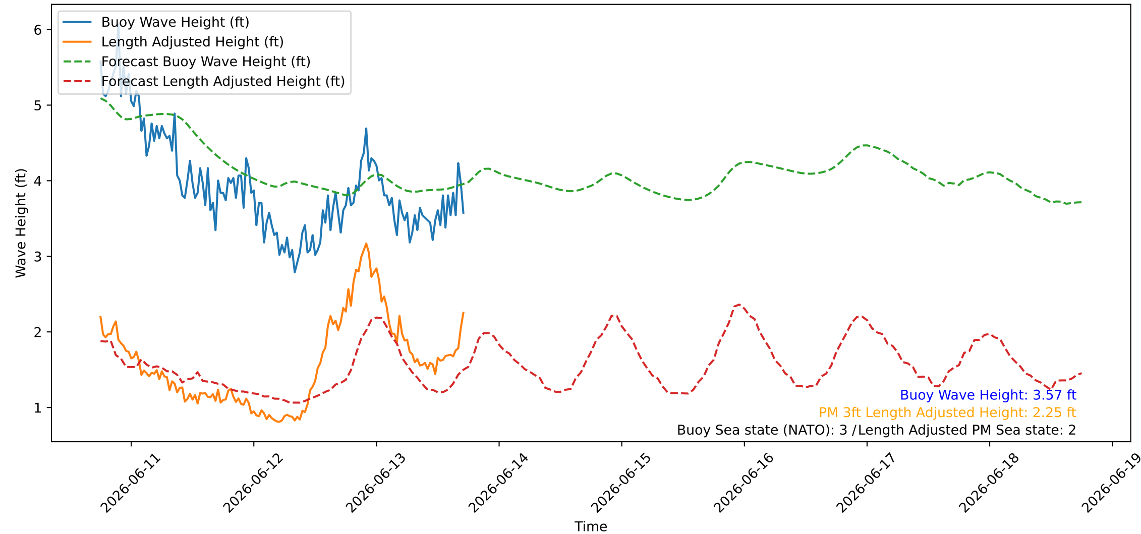
Wave Heights over Time for Oceanside Harbor at 2026-06-13 17:50:26
