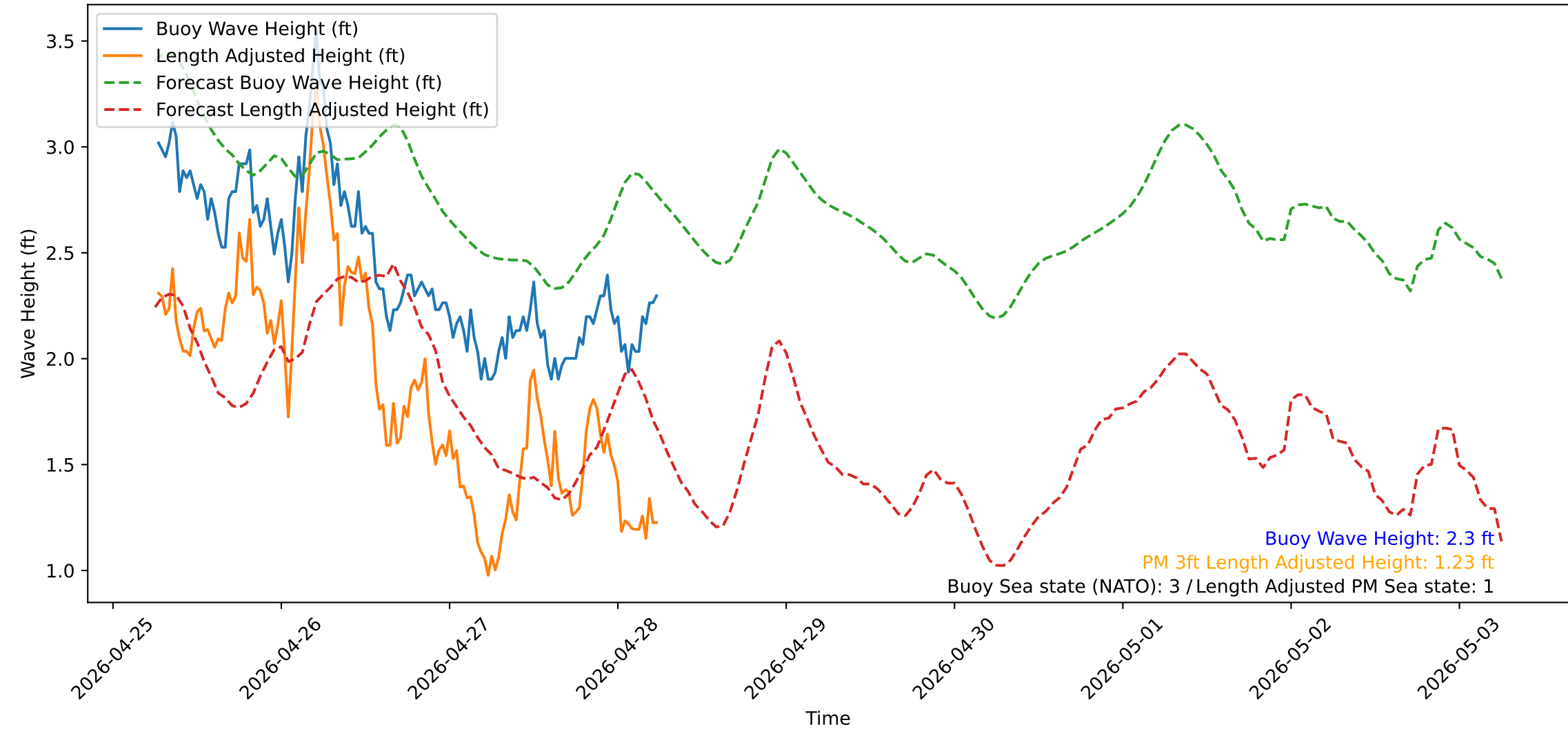
Wave Heights over Time for Red Beach at 2026-04-28 06:20:52
