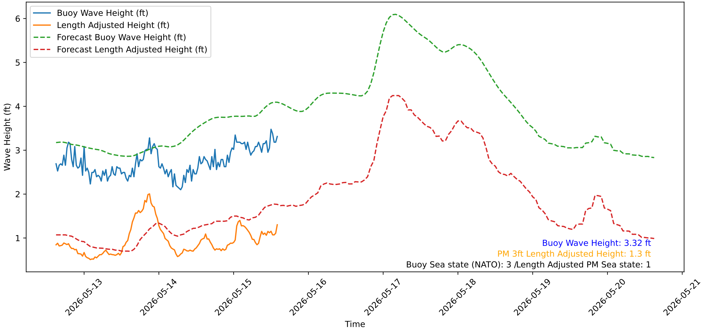
Wave Heights over Time for Green Beach at 2026-05-15 14:51:14
