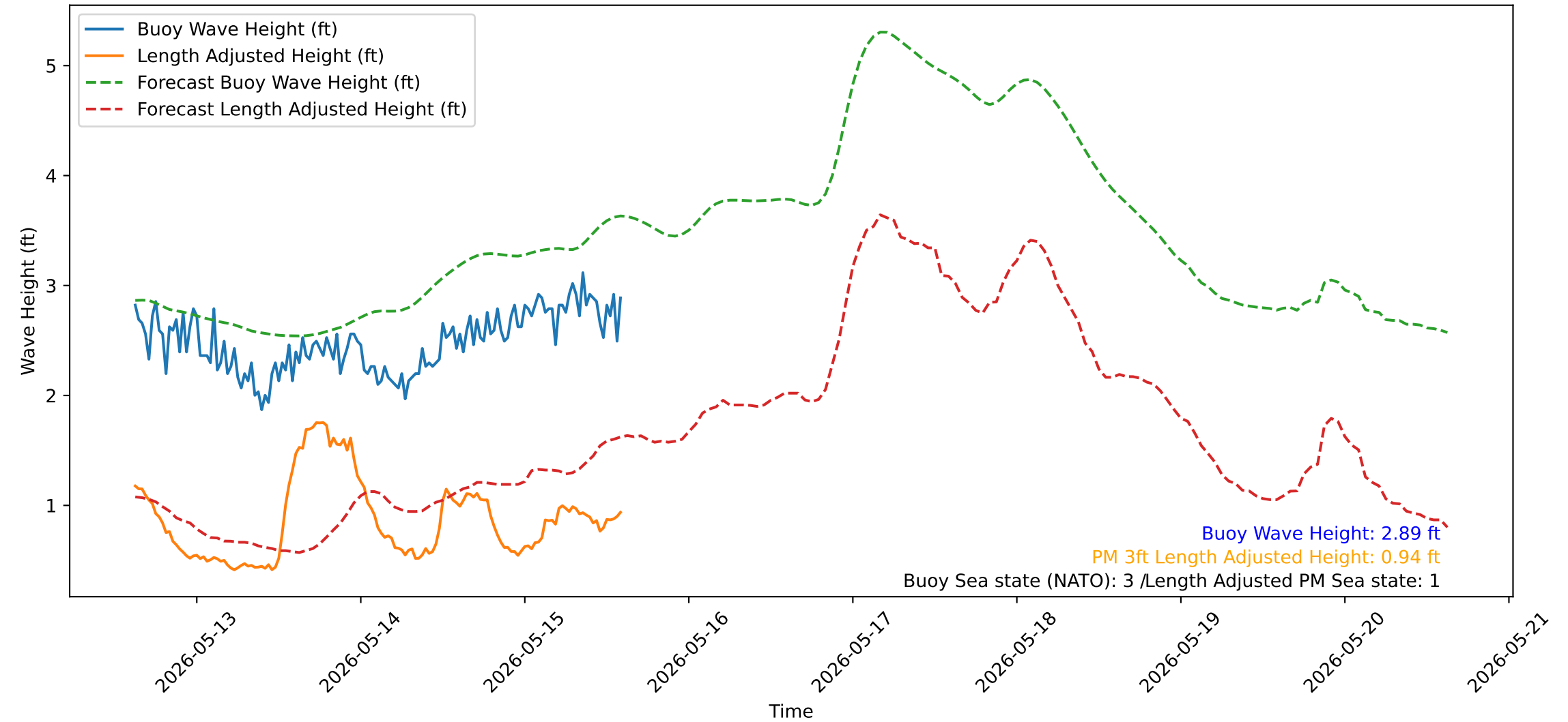
Wave Heights over Time for Red Beach at 2026-05-15 14:50:51
