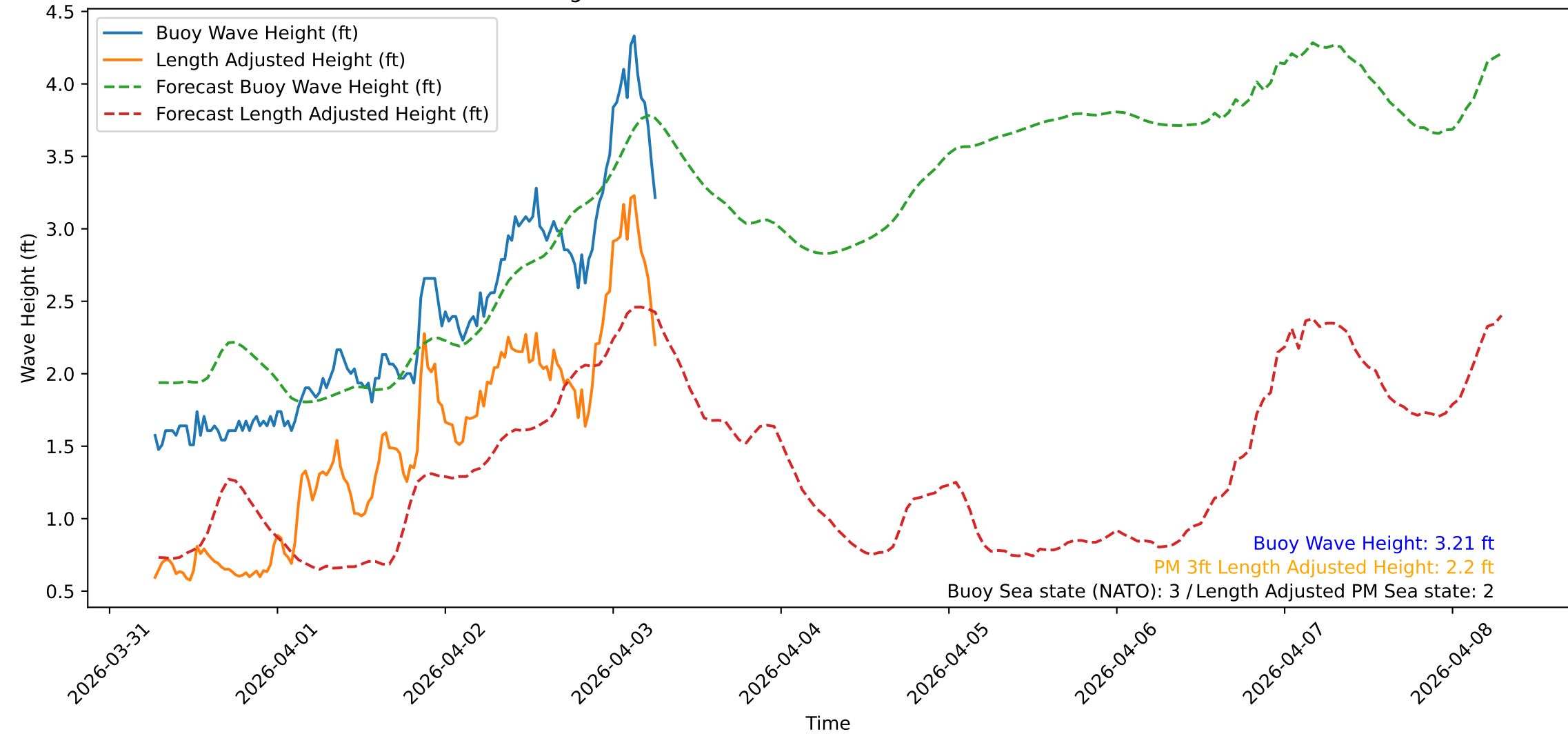
Wave Heights over Time for Green Beach at 2026-04-03 06:41:11
