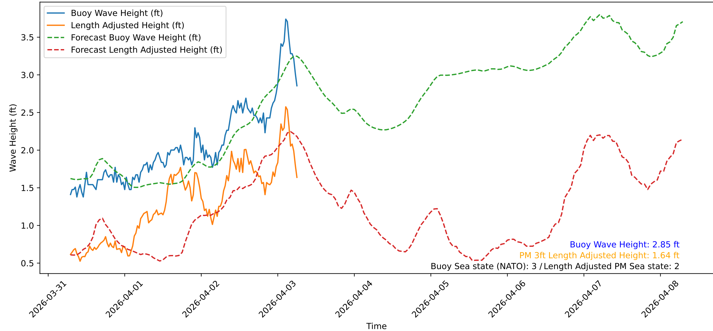
Wave Heights over Time for Red Beach at 2026-04-03 06:40:48
