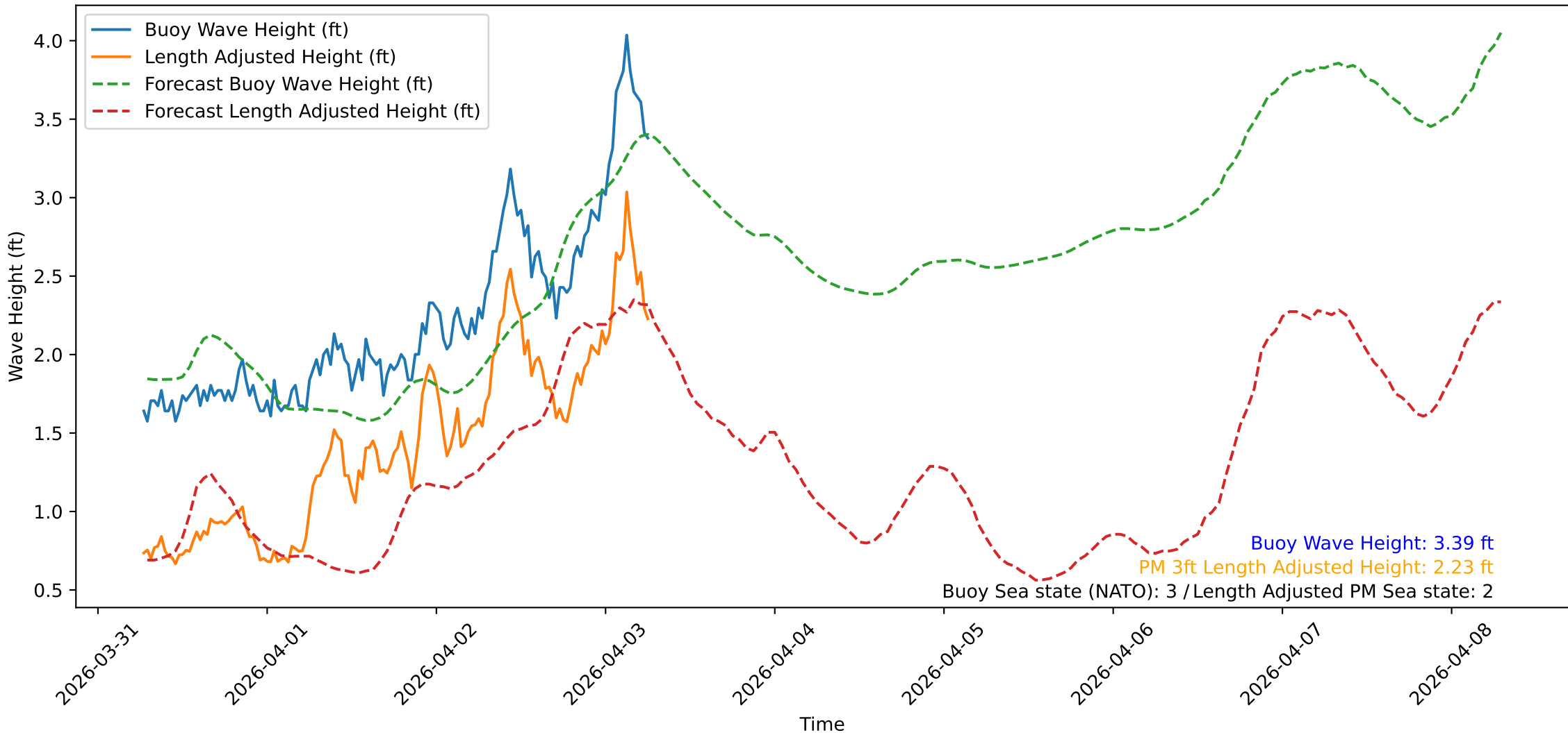
Wave Heights over Time for Oceanside Harbor at 2026-04-03 06:40:31
