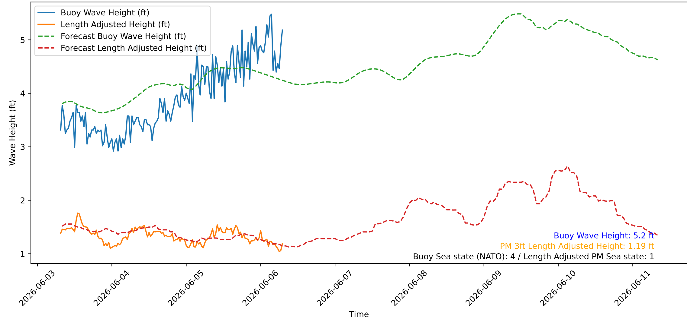
Wave Heights over Time for Oceanside Harbor at 2026-06-06 07:40:26
