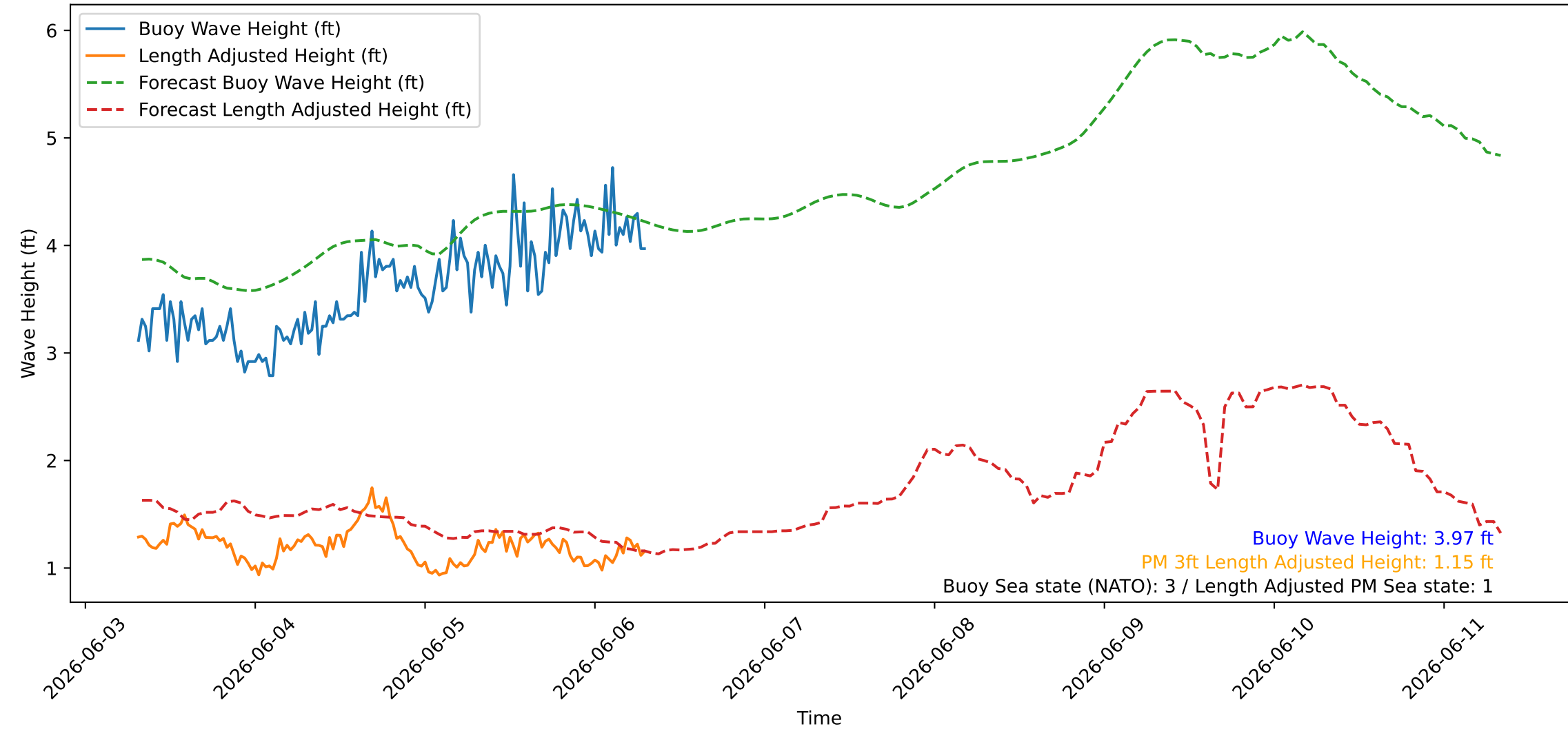
Wave Heights over Time for Green Beach at 2026-06-06 07:41:08
