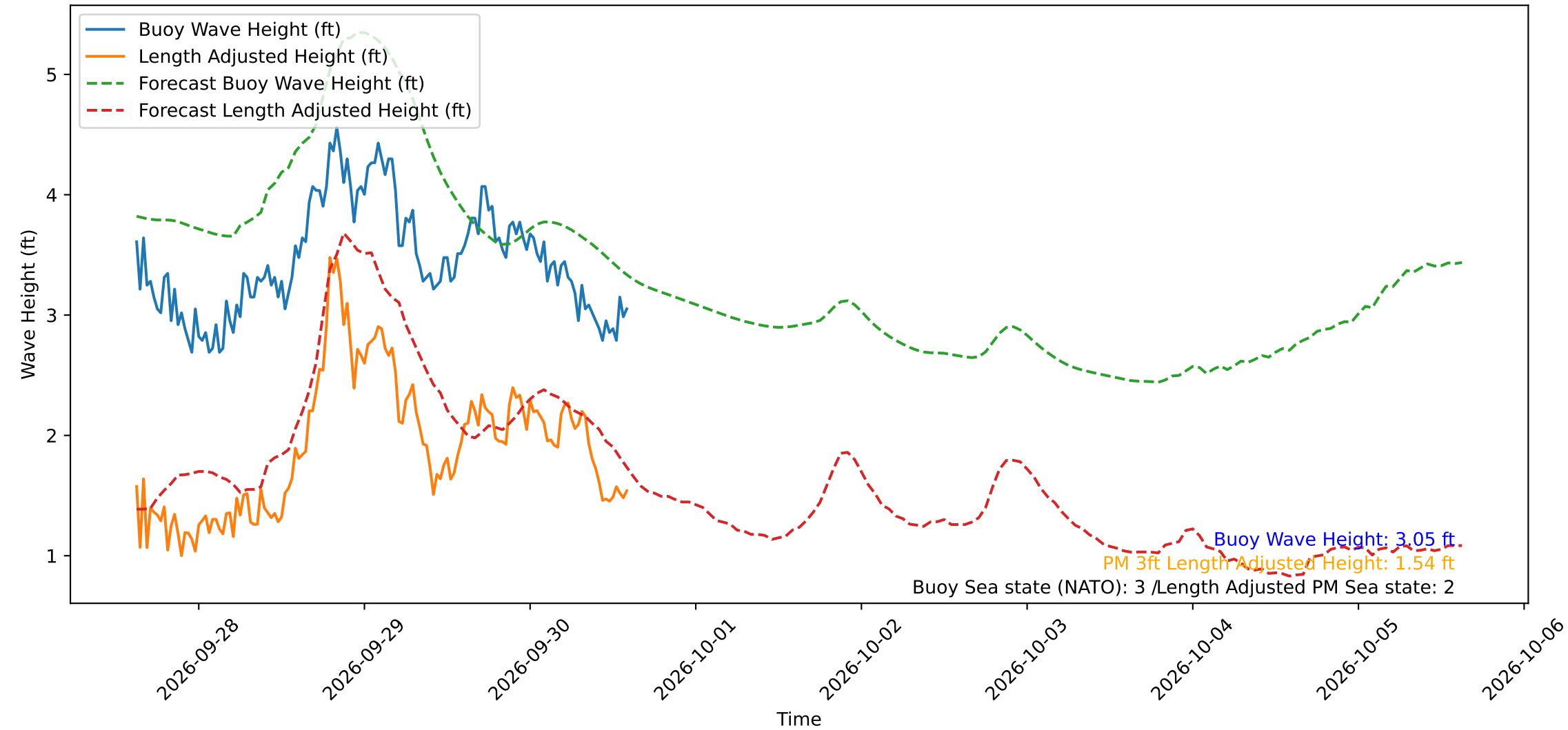
Wave Heights over Time for Green Beach at 2026-09-30 14:41:12
