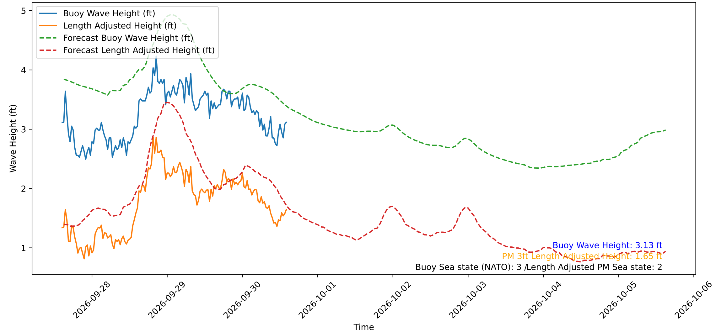
Wave Heights over Time for Oceanside Harbor at 2026-09-30 14:40:30
