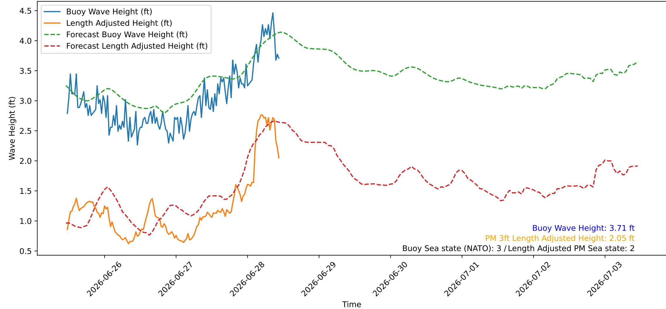
Wave Heights over Time for Red Beach at 2026-06-28 11:10:45
