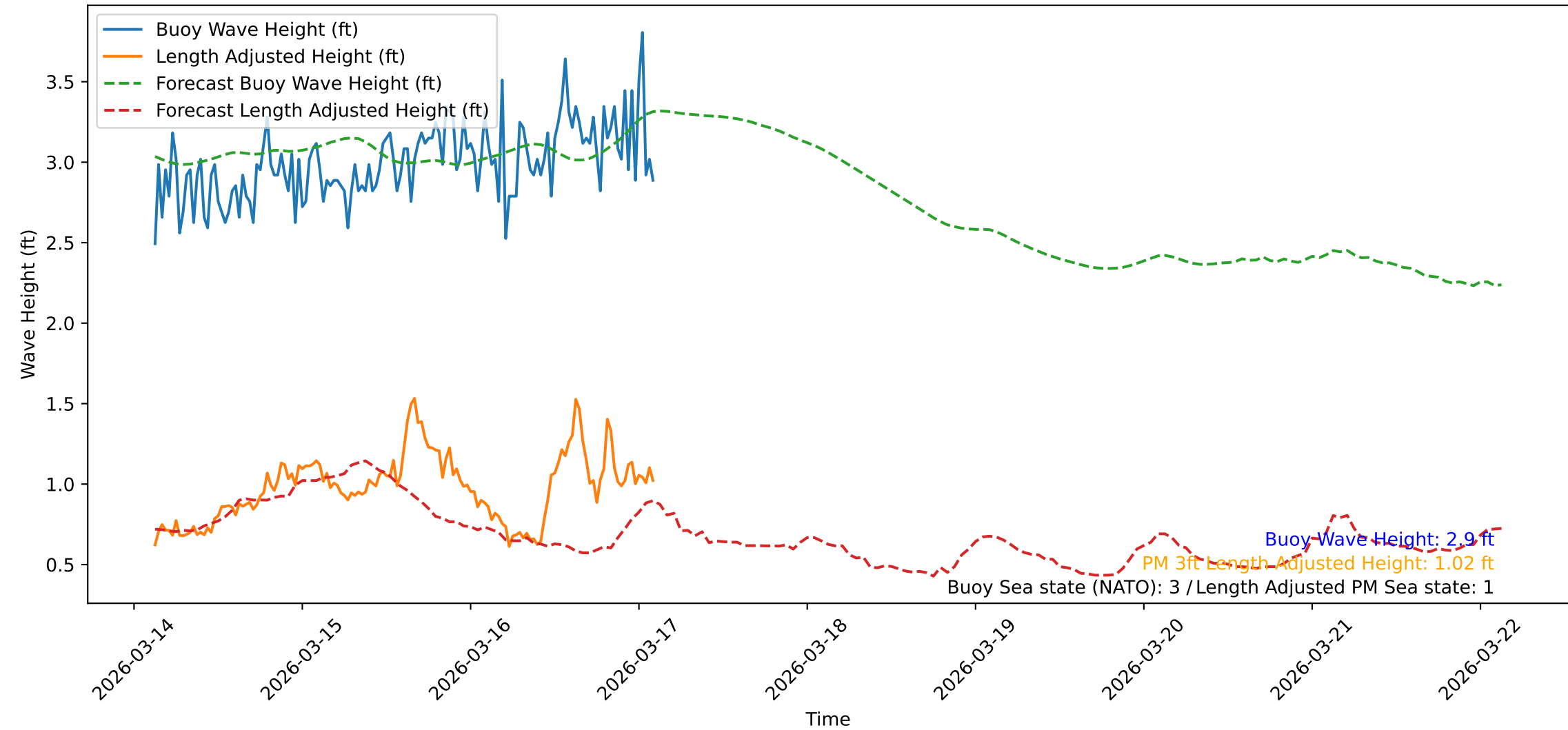
Wave Heights over Time for Red Beach at 2026-03-17 02:41:06
