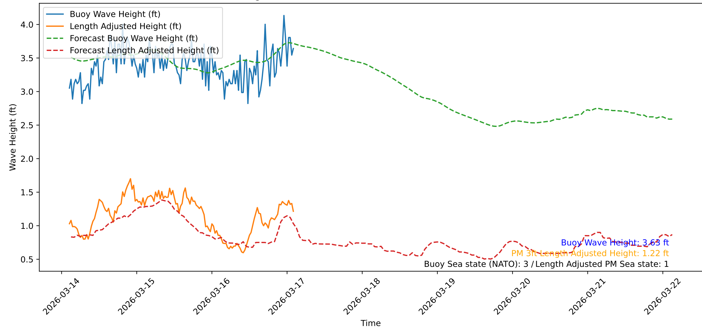
Wave Heights over Time for Green Beach at 2026-03-17 02:41:42
