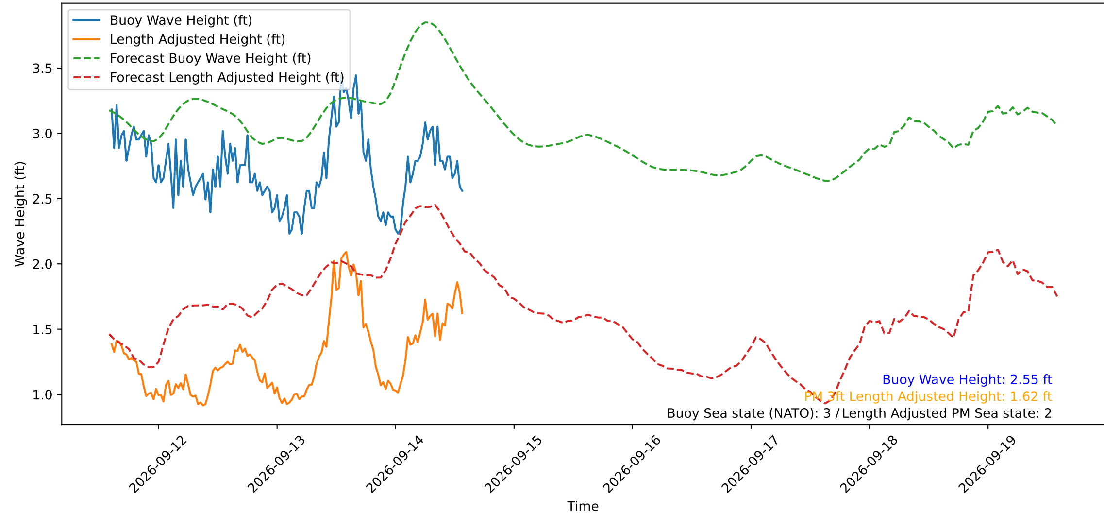
Wave Heights over Time for Red Beach at 2026-09-14 14:10:48
