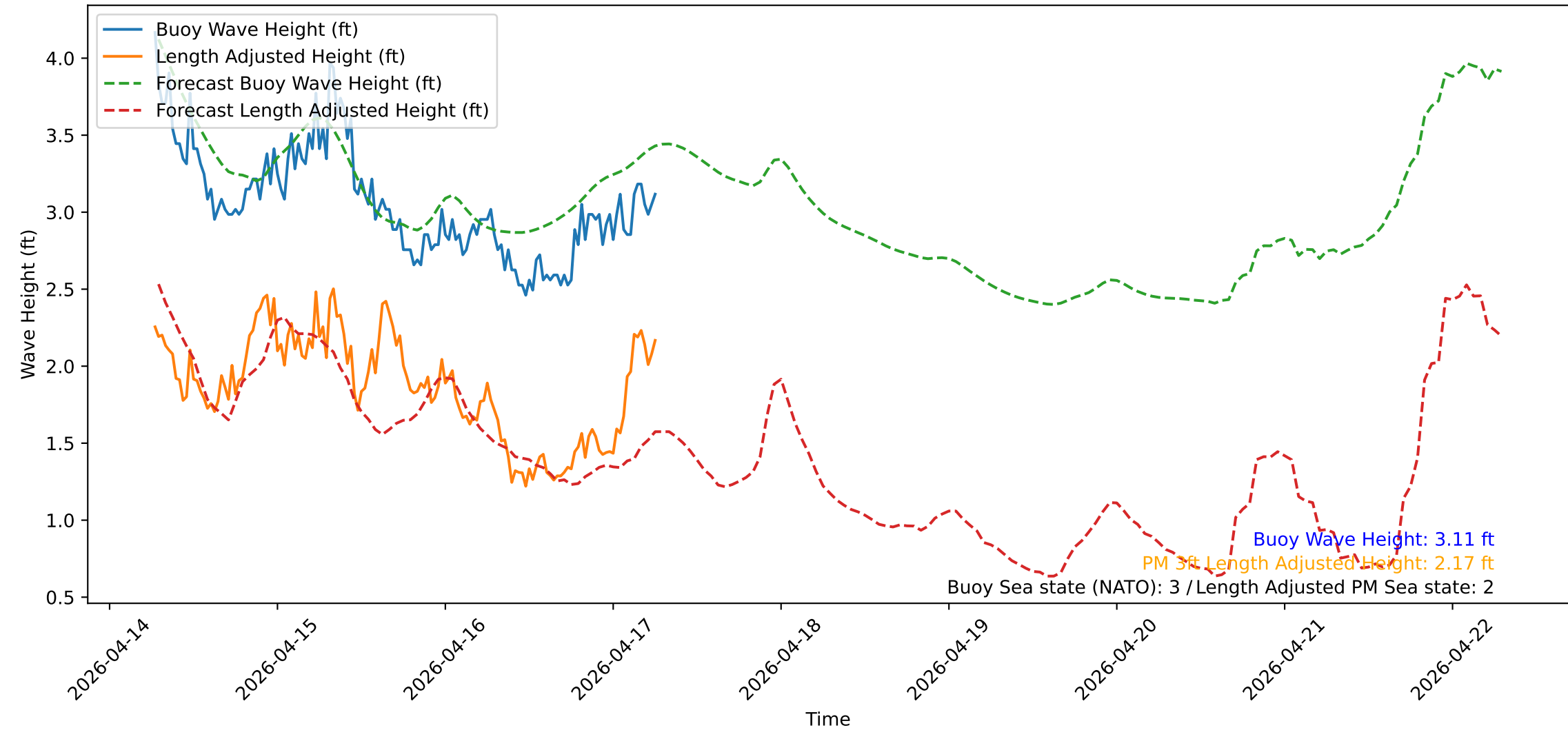
Wave Heights over Time for Green Beach at 2026-04-17 06:41:14
