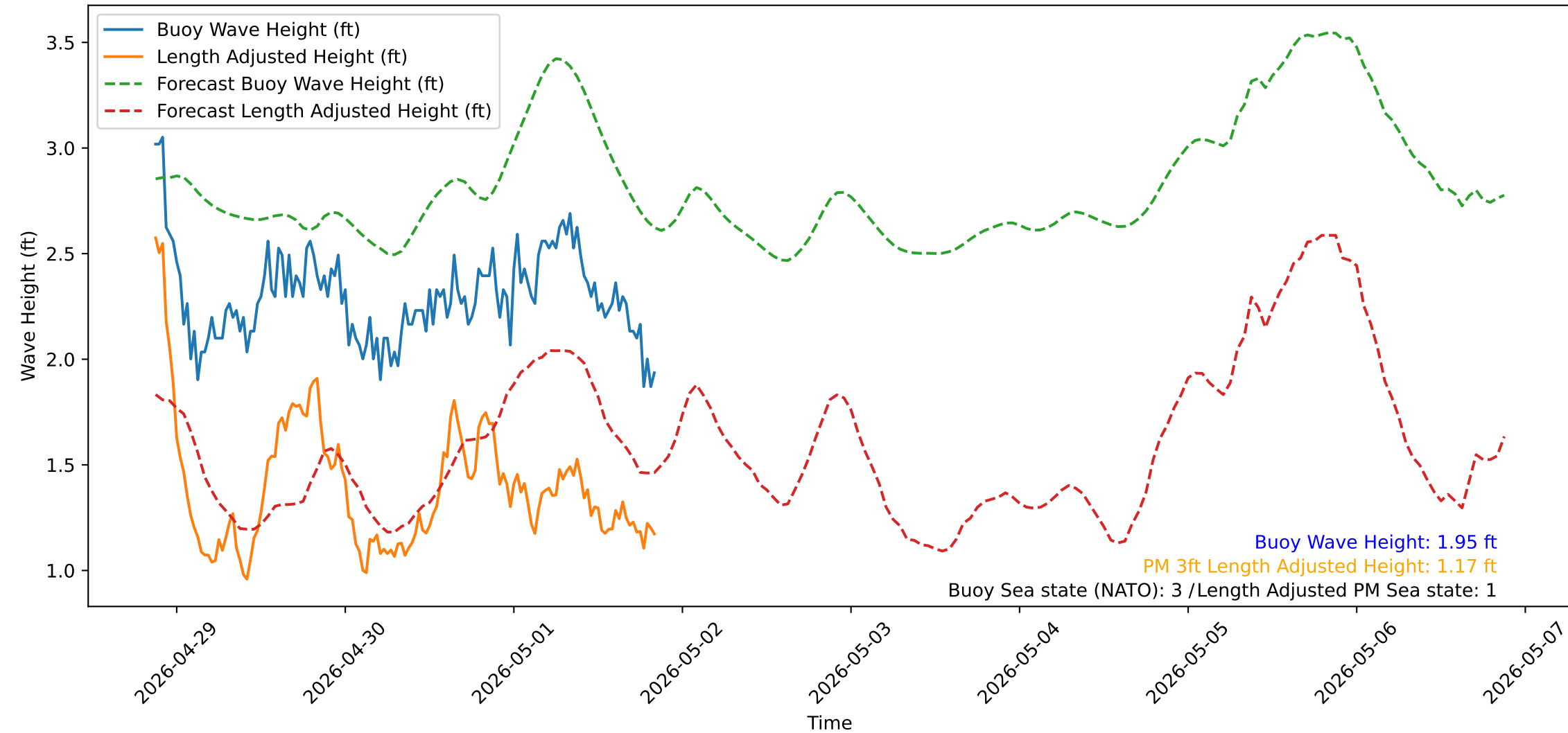
Wave Heights over Time for Oceanside Harbor at 2026-05-01 21:00:31
