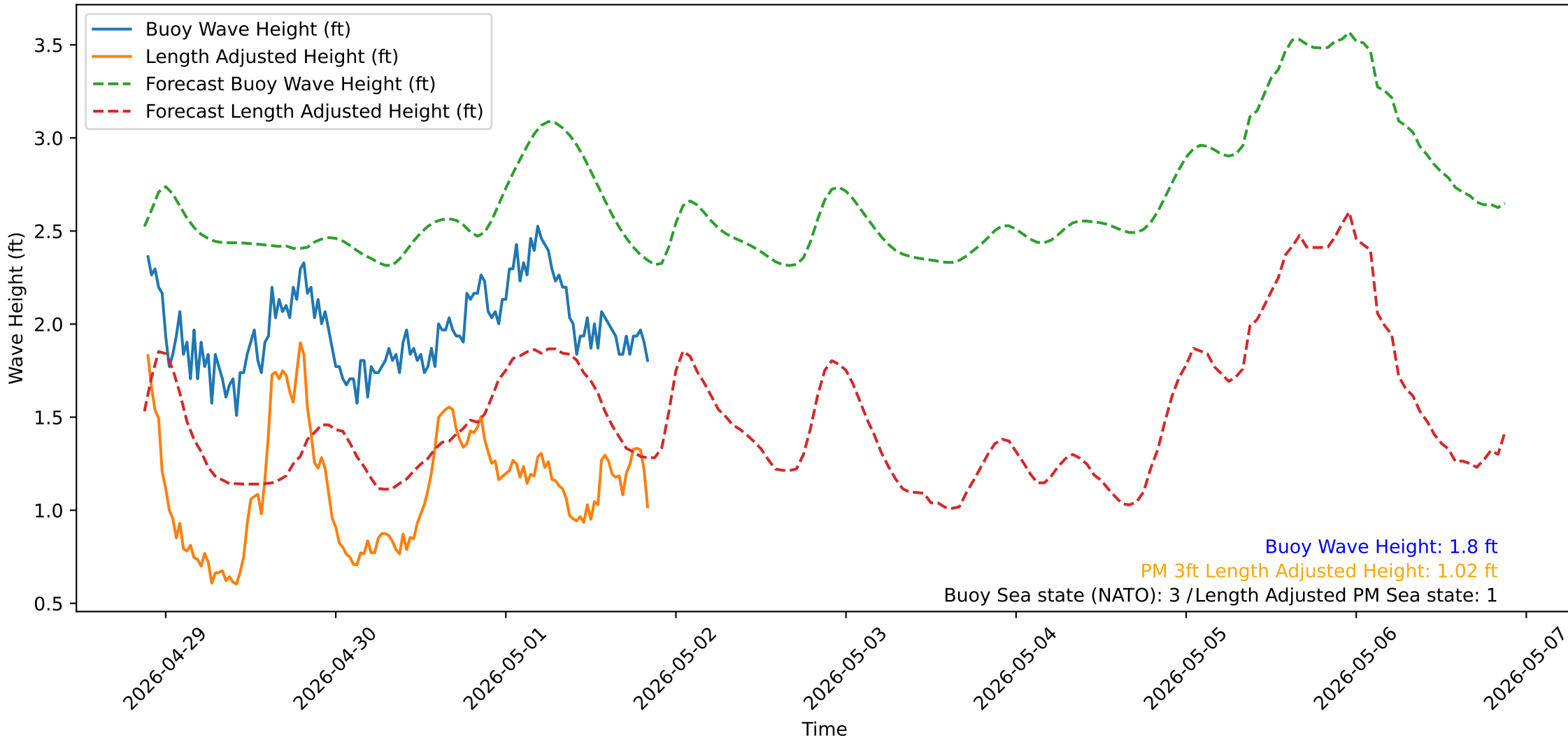
Wave Heights over Time for Red Beach at 2026-05-01 21:00:51
