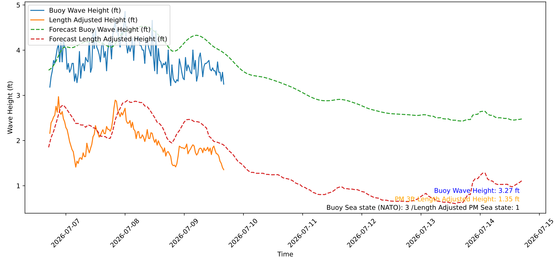
Wave Heights over Time for Red Beach at 2026-07-09 17:00:46
