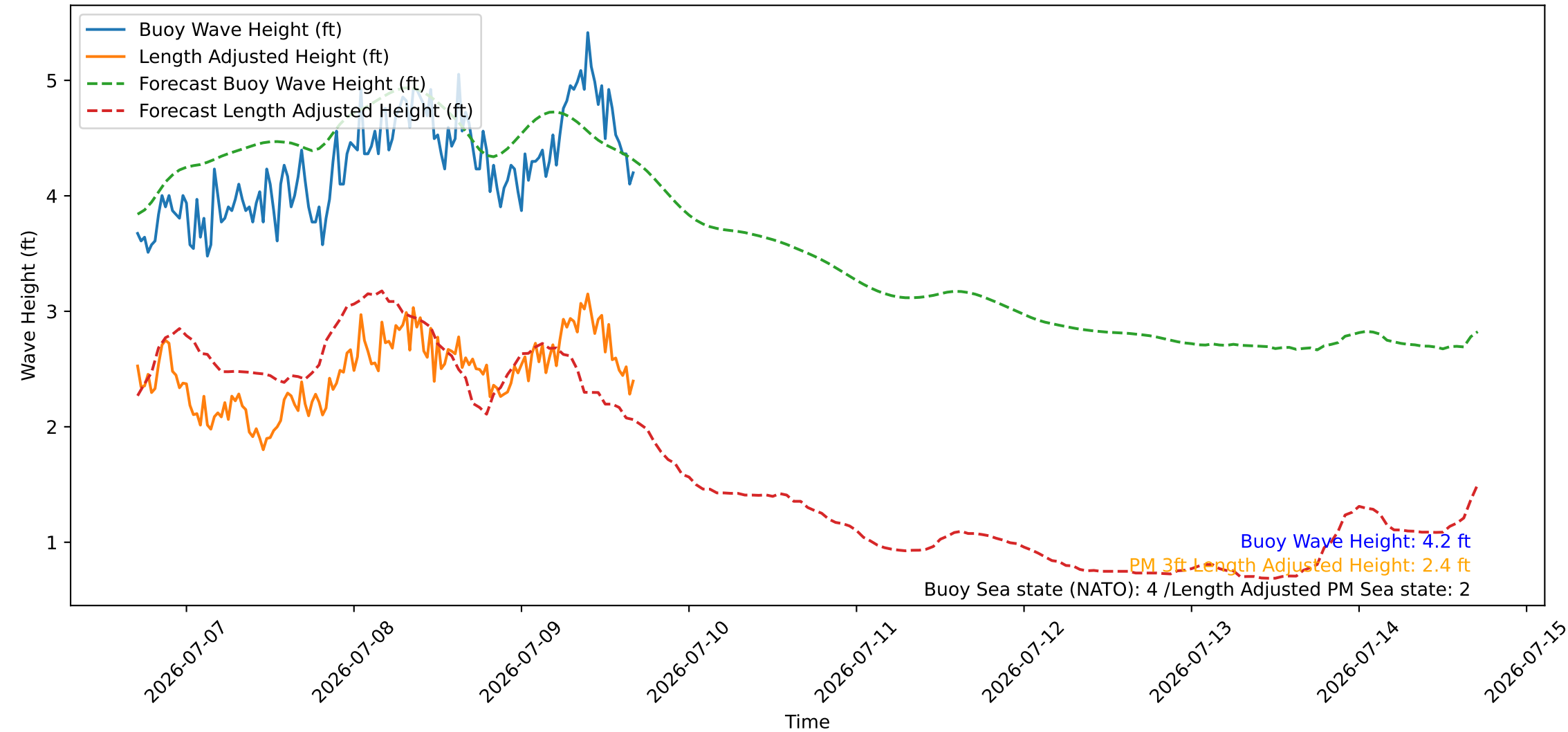
Wave Heights over Time for Oceanside Harbor at 2026-07-09 17:00:26
