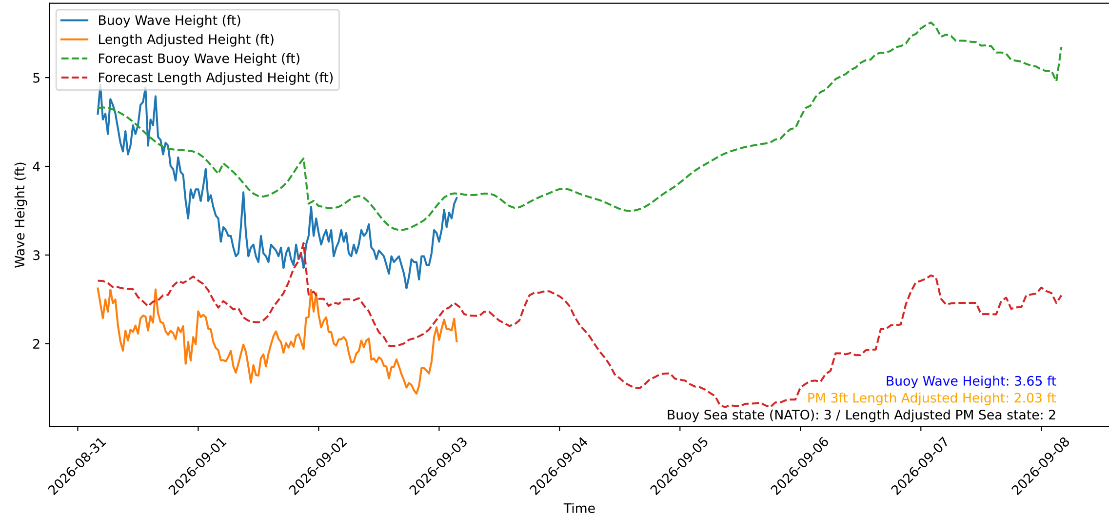
Wave Heights over Time for Oceanside Harbor at 2026-09-03 04:10:29
