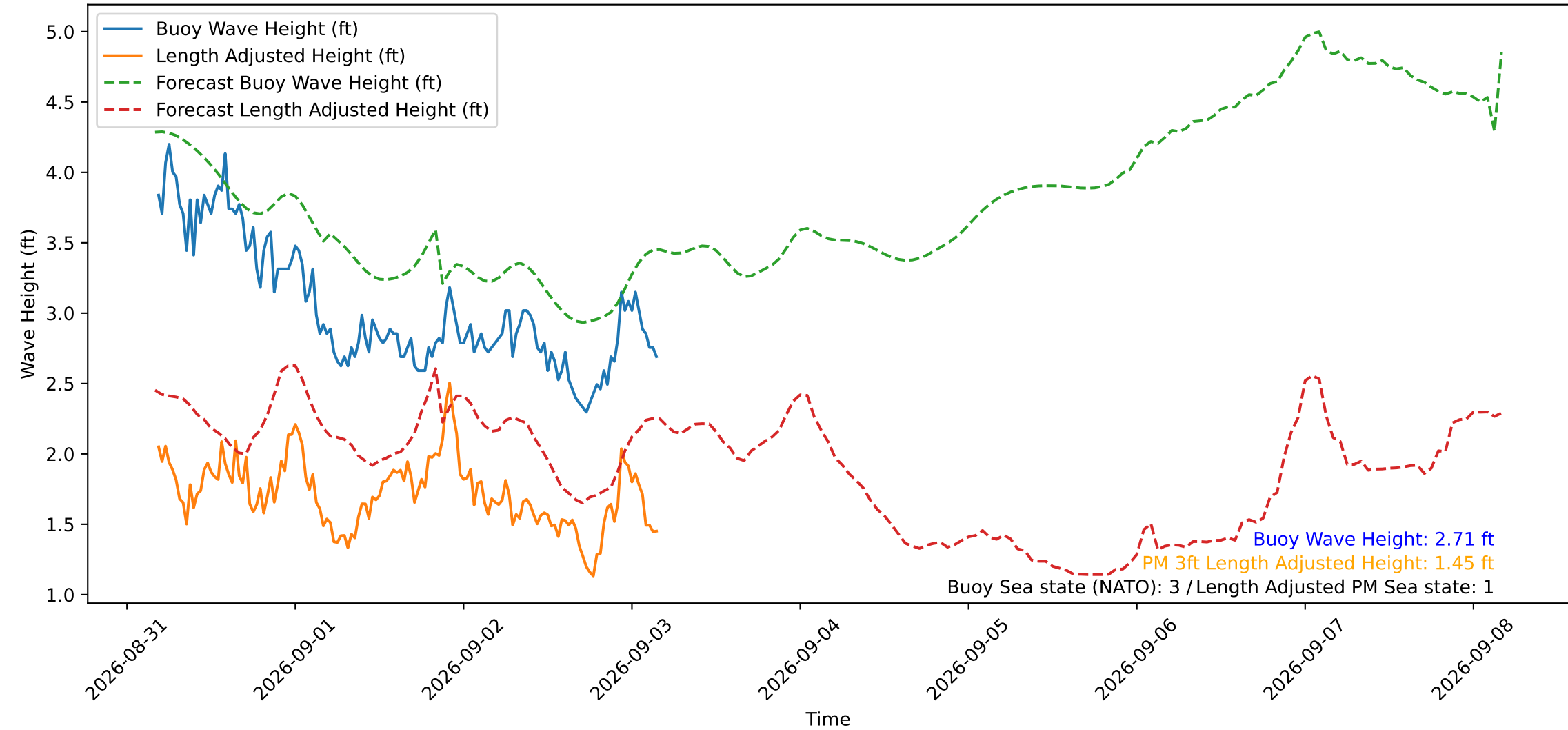
Wave Heights over Time for Red Beach at 2026-09-03 04:10:49
