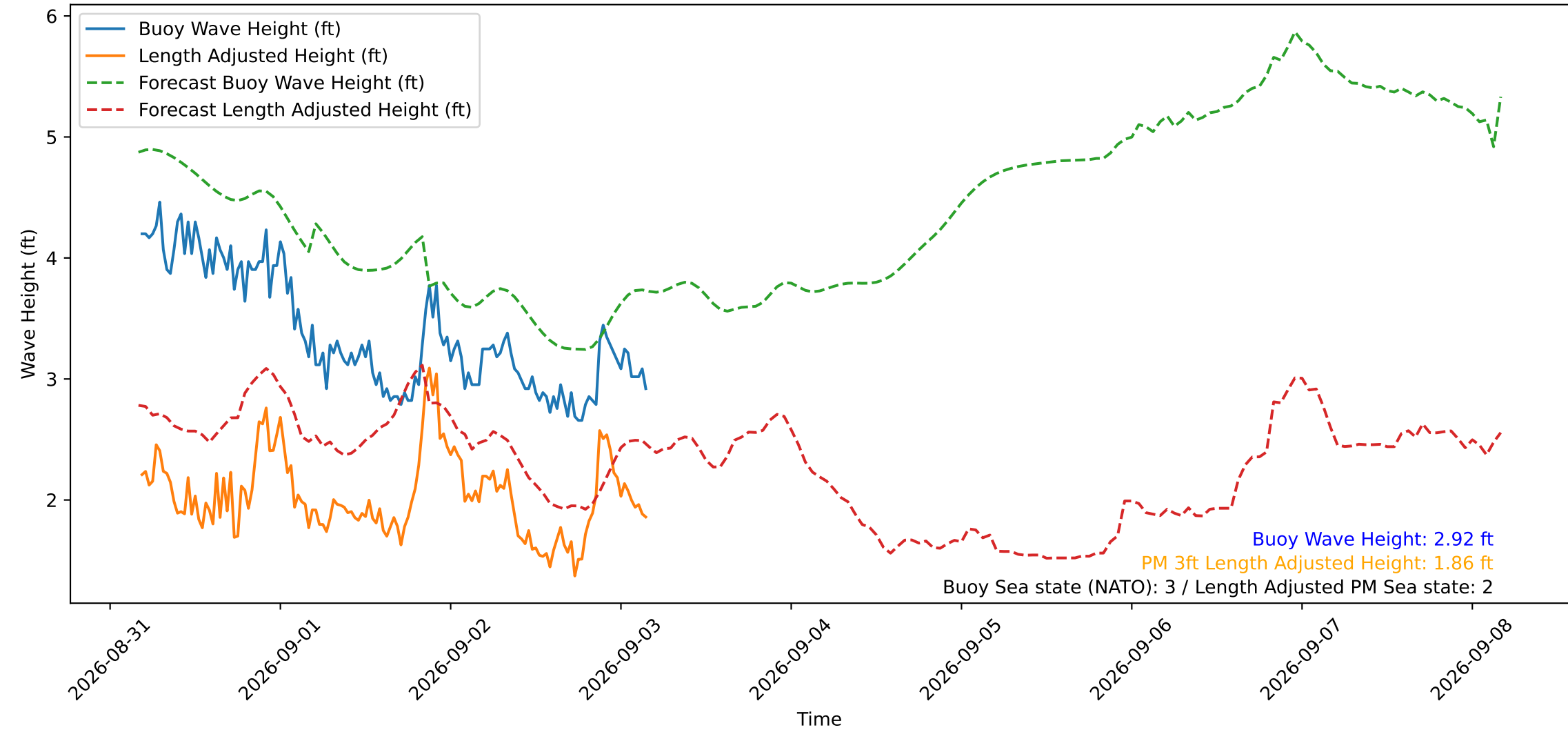
Wave Heights over Time for Green Beach at 2026-09-03 04:11:11
