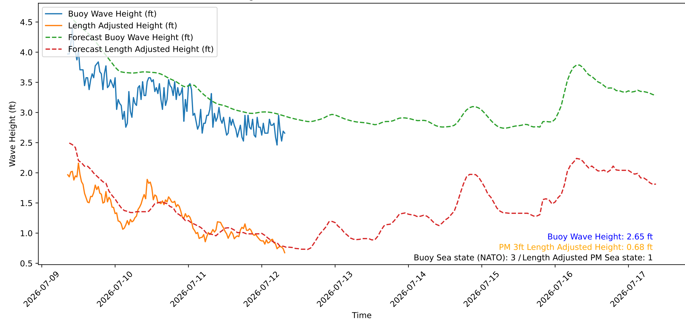
Wave Heights over Time for Green Beach at 2026-07-12 08:31:08
