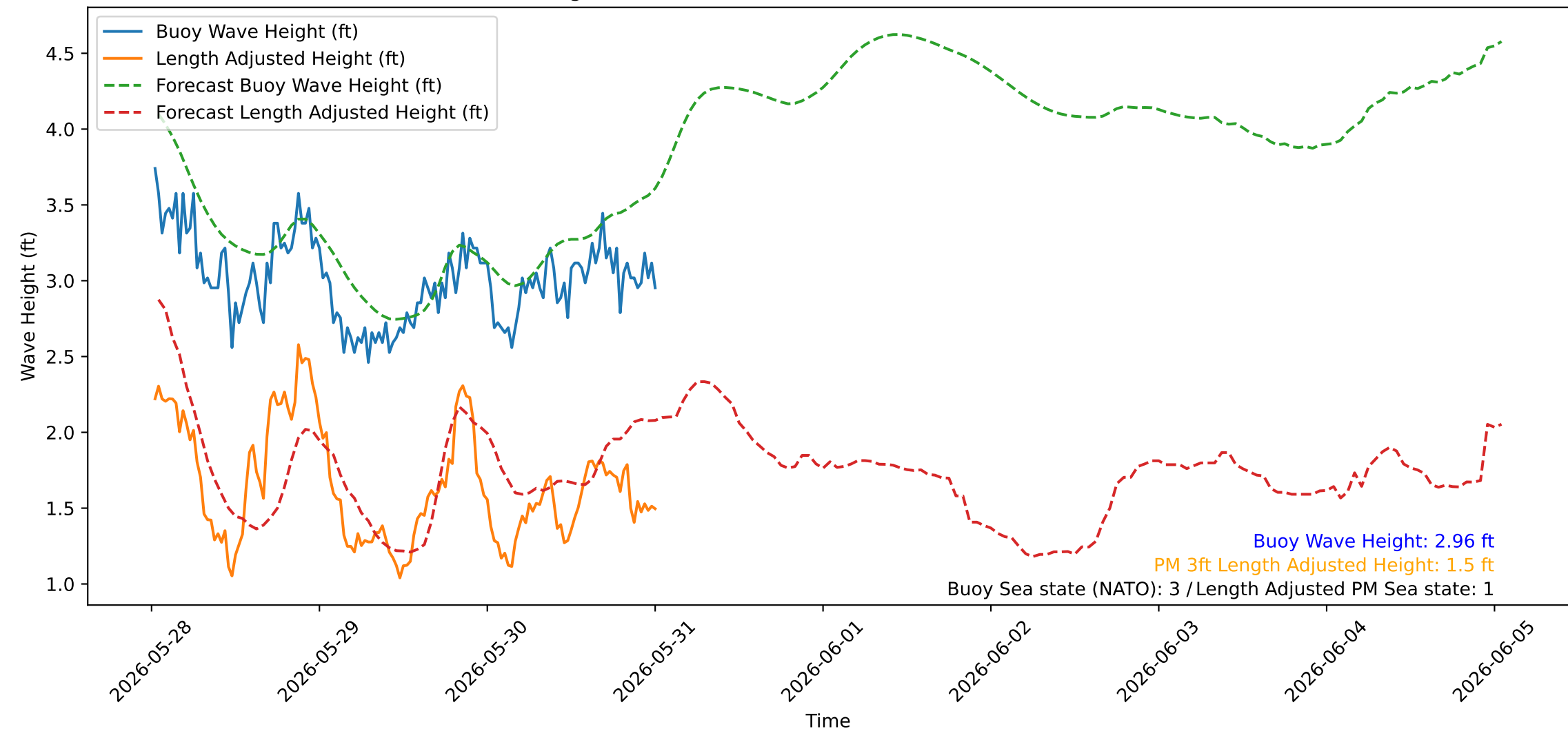
Wave Heights over Time for Green Beach at 2026-05-31 00:41:08
