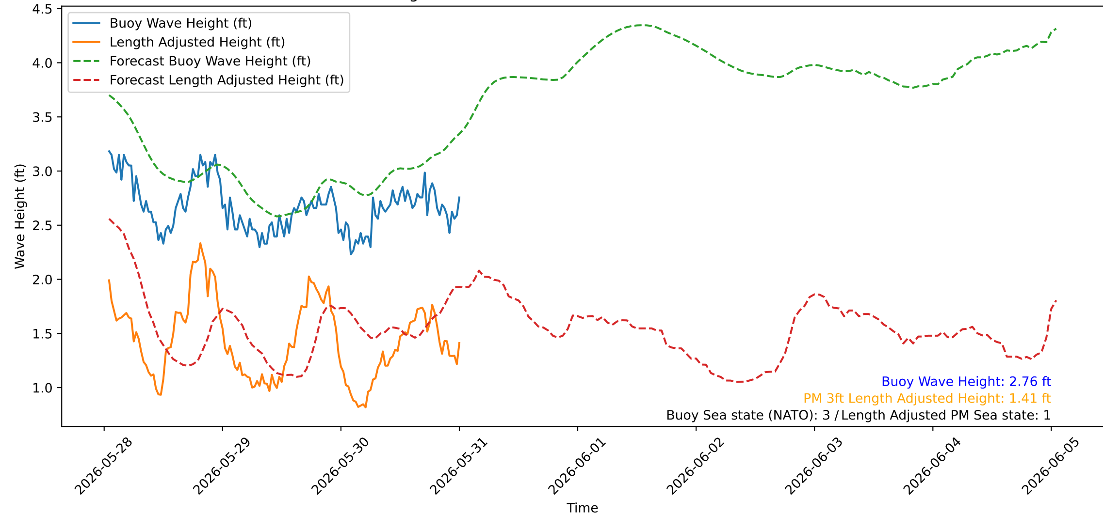
Wave Heights over Time for Red Beach at 2026-05-31 00:40:45
