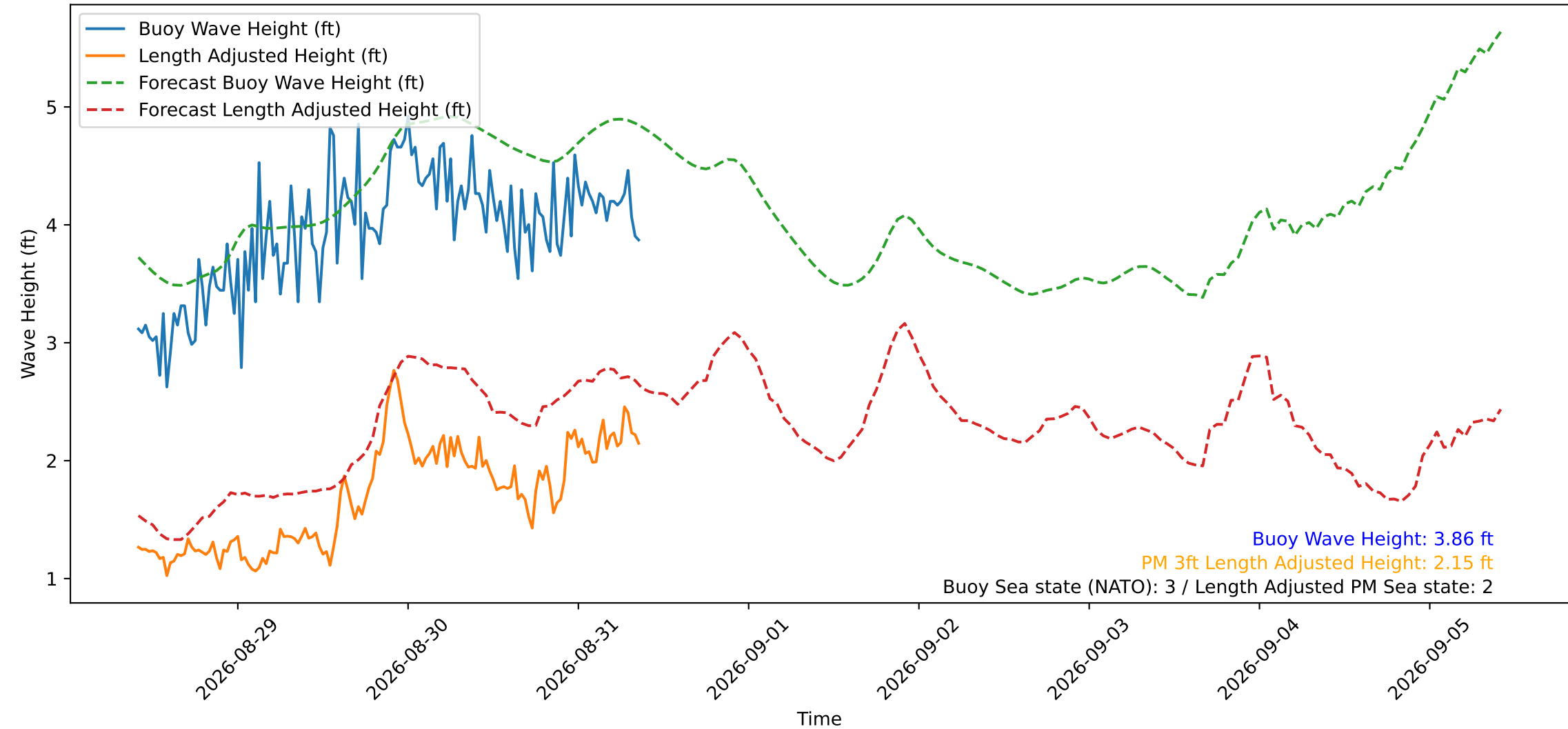
Wave Heights over Time for Green Beach at 2026-08-31 09:31:12
