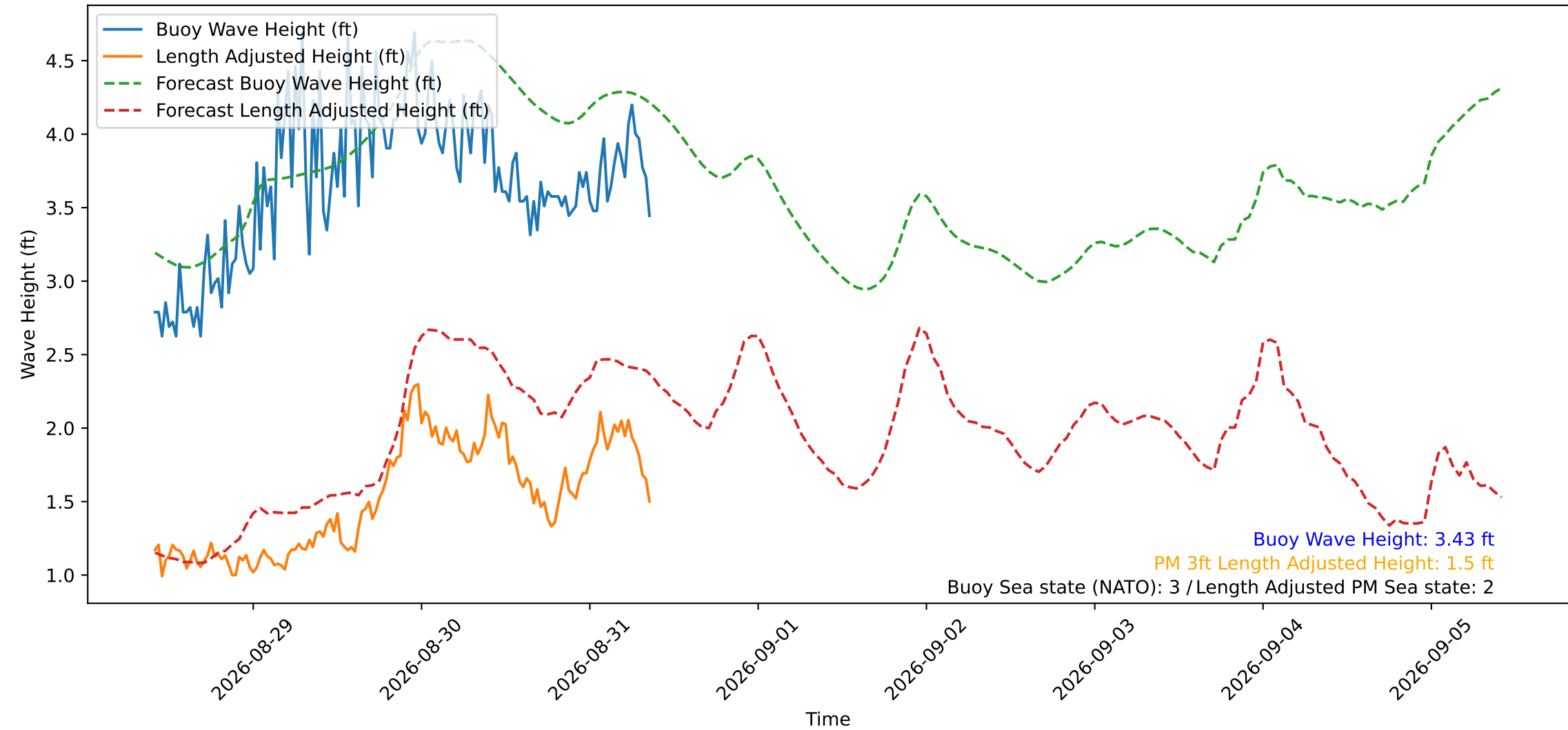
Wave Heights over Time for Red Beach at 2026-08-31 09:30:49
