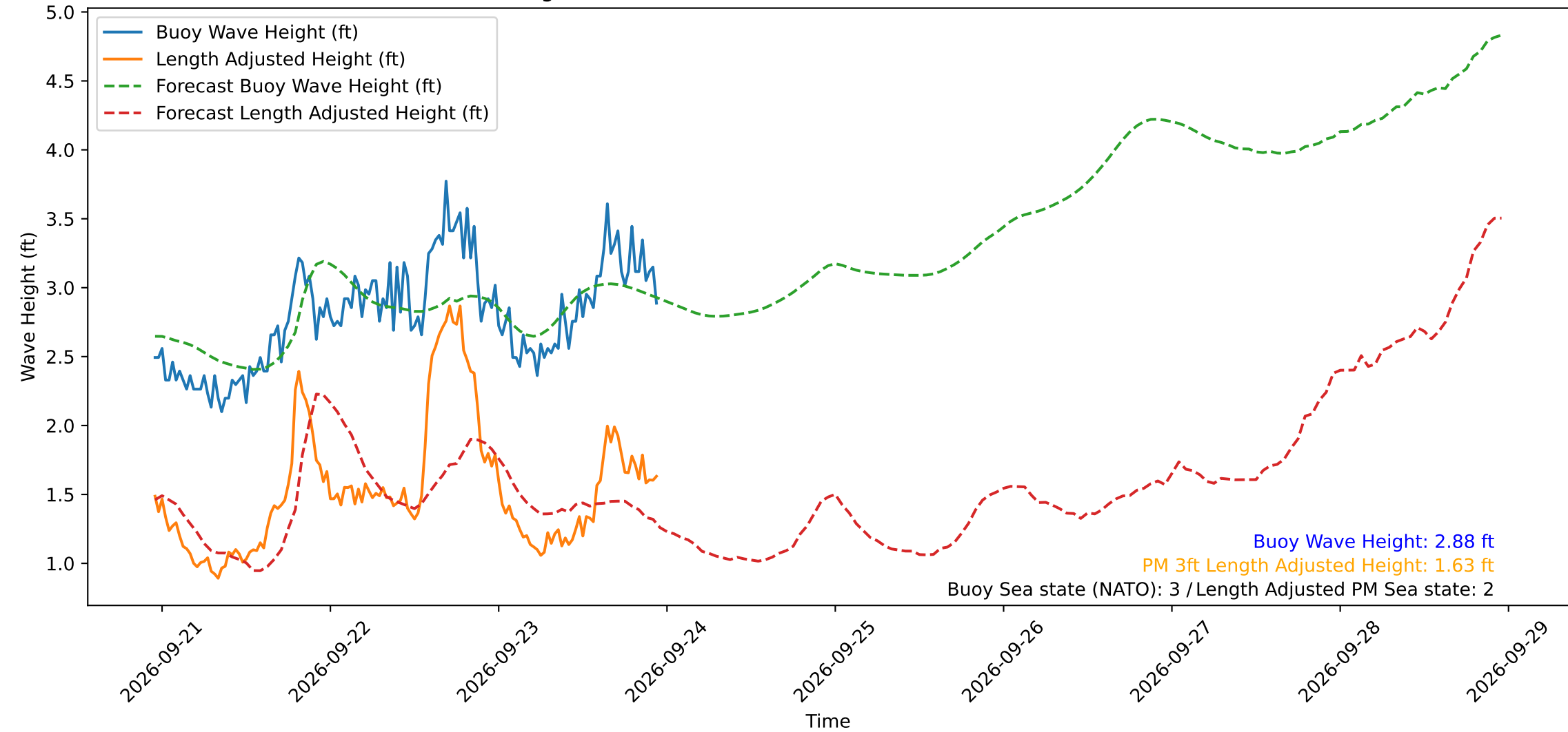
Wave Heights over Time for Oceanside Harbor at 2026-09-23 23:10:30
