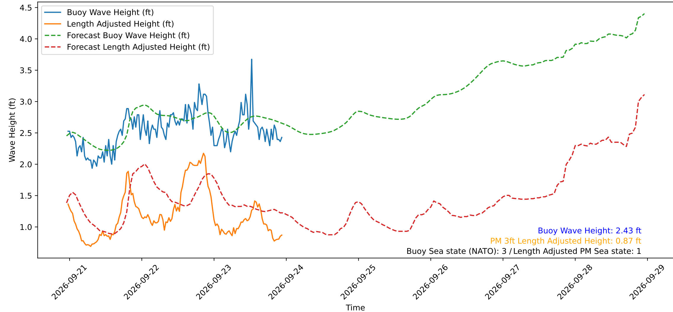
Wave Heights over Time for Red Beach at 2026-09-23 23:10:50
