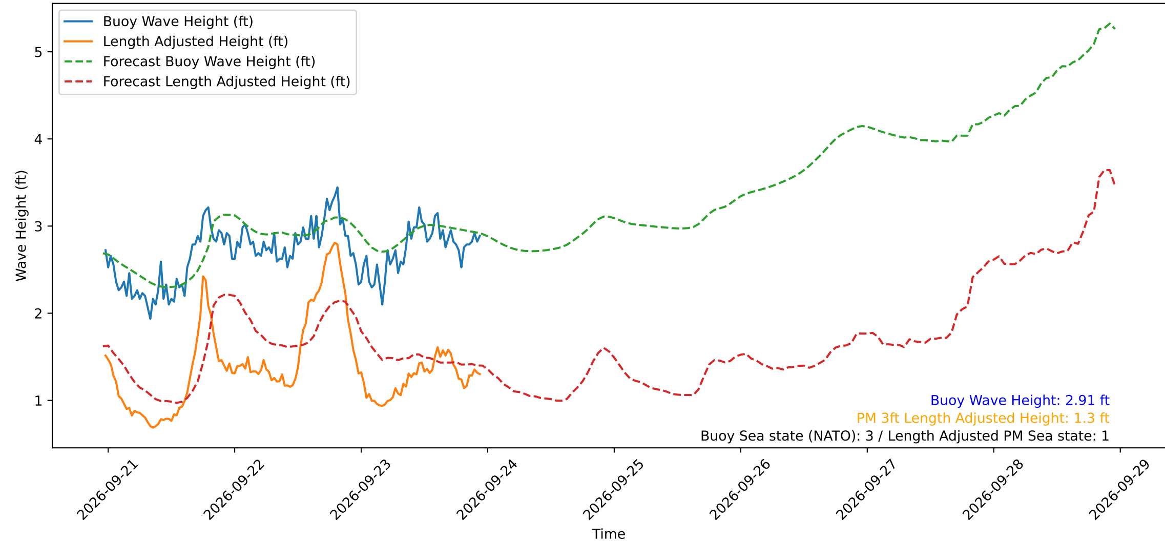
Wave Heights over Time for Green Beach at 2026-09-23 23:11:12
