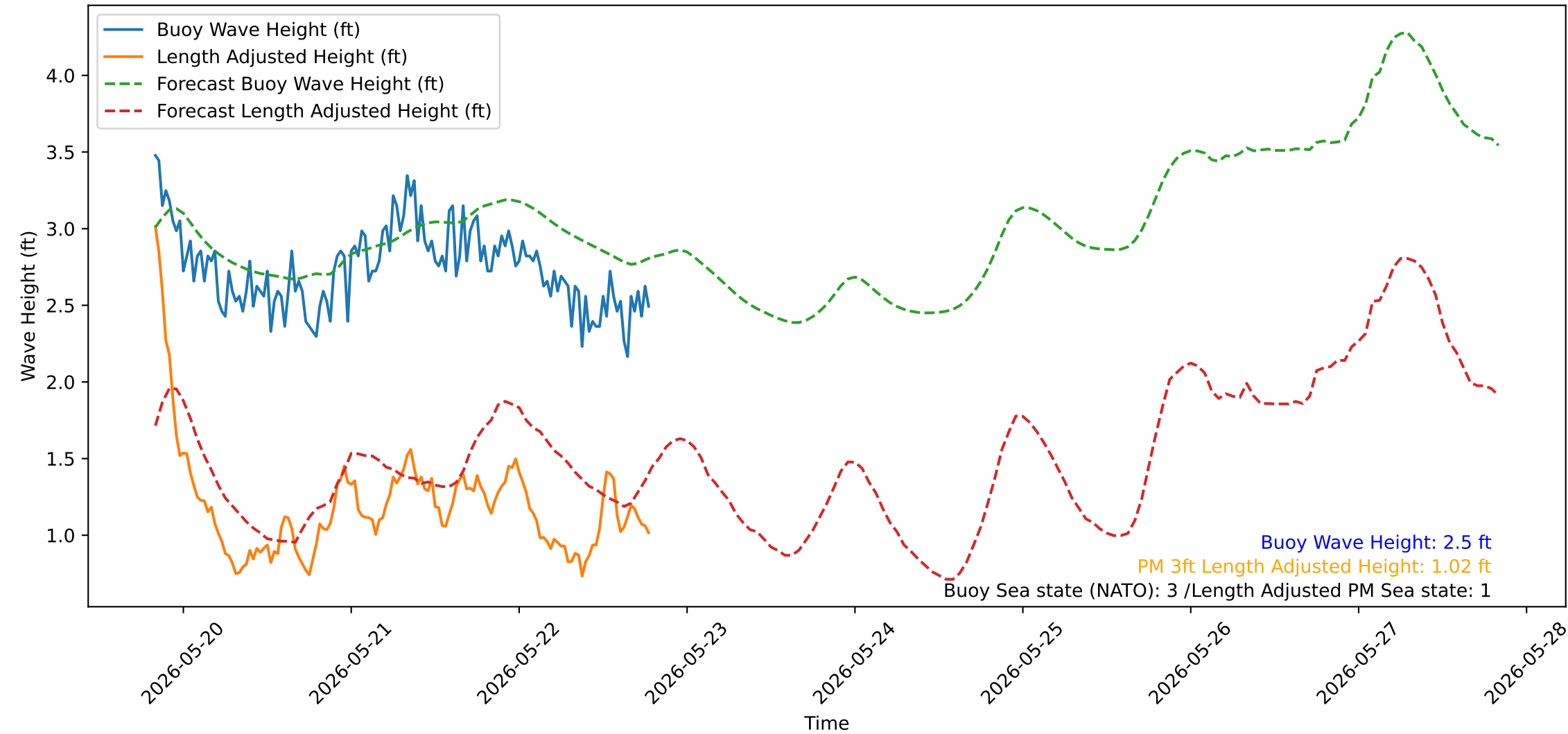
Wave Heights over Time for Red Beach at 2026-05-22 19:30:52
