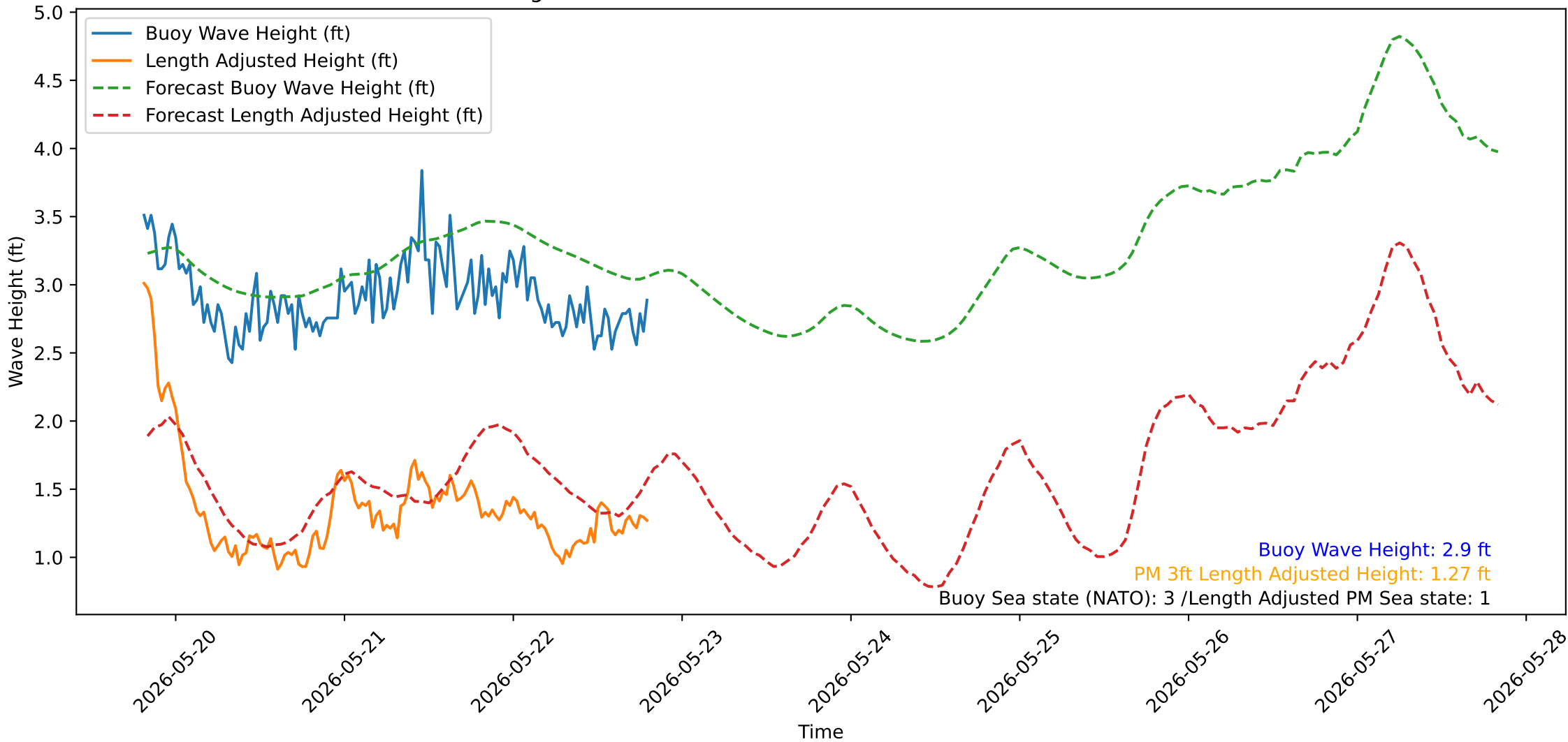
Wave Heights over Time for Oceanside Harbor at 2026-05-22 19:30:32
