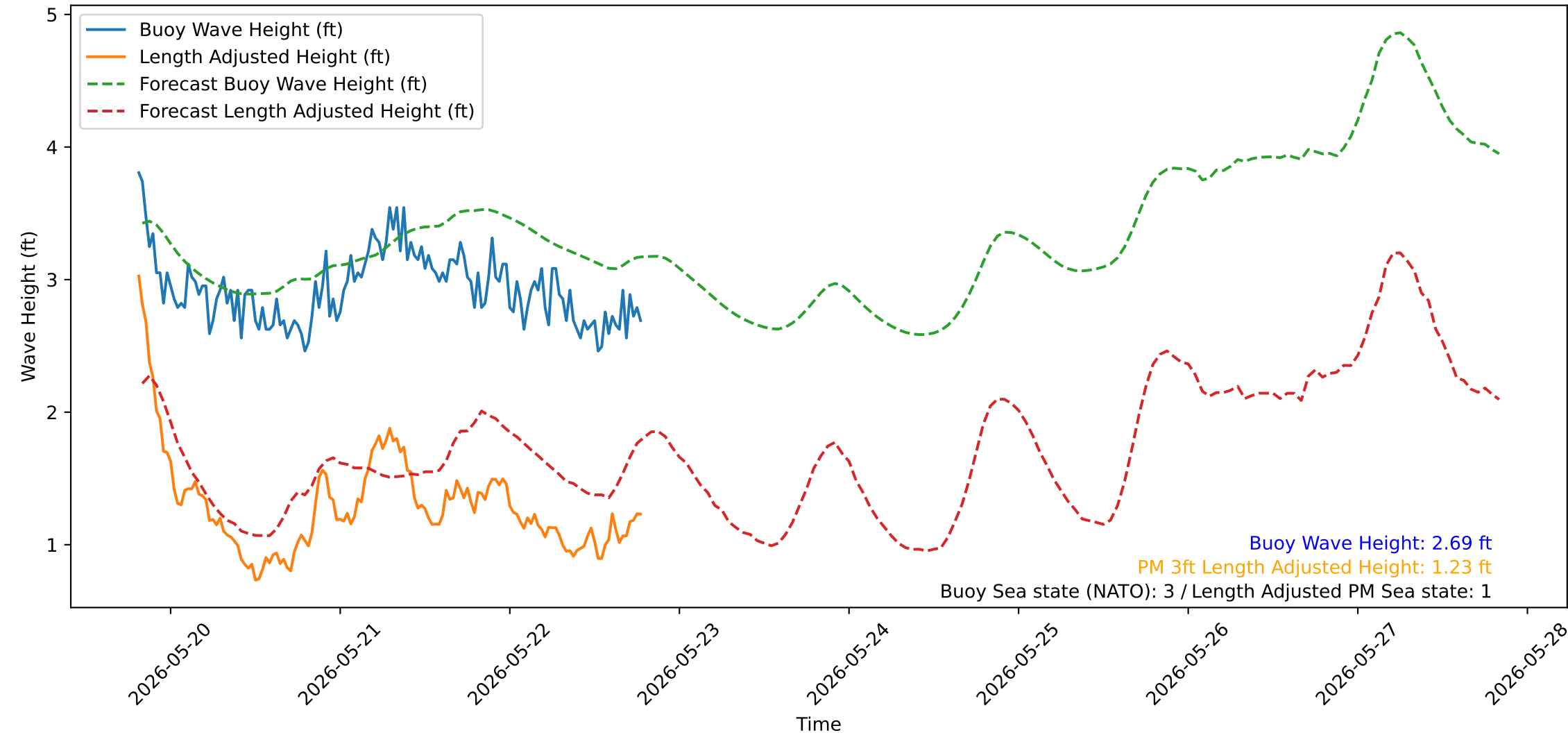
Wave Heights over Time for Green Beach at 2026-05-22 19:31:14
