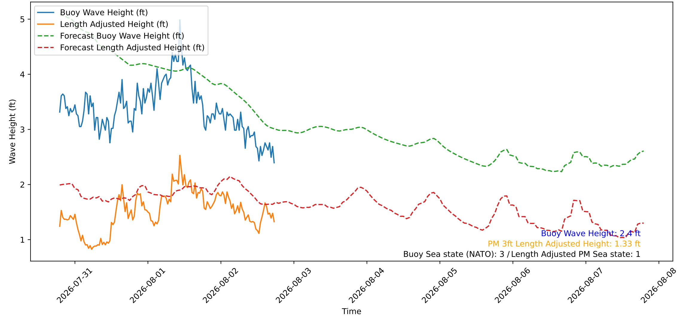
Wave Heights over Time for Green Beach at 2026-08-02 18:51:10
