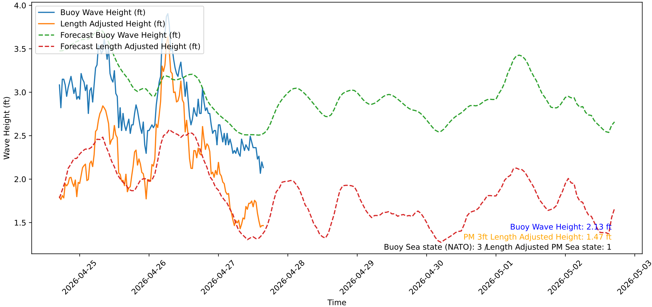
Wave Heights over Time for Oceanside Harbor at 2026-04-27 16:50:31
