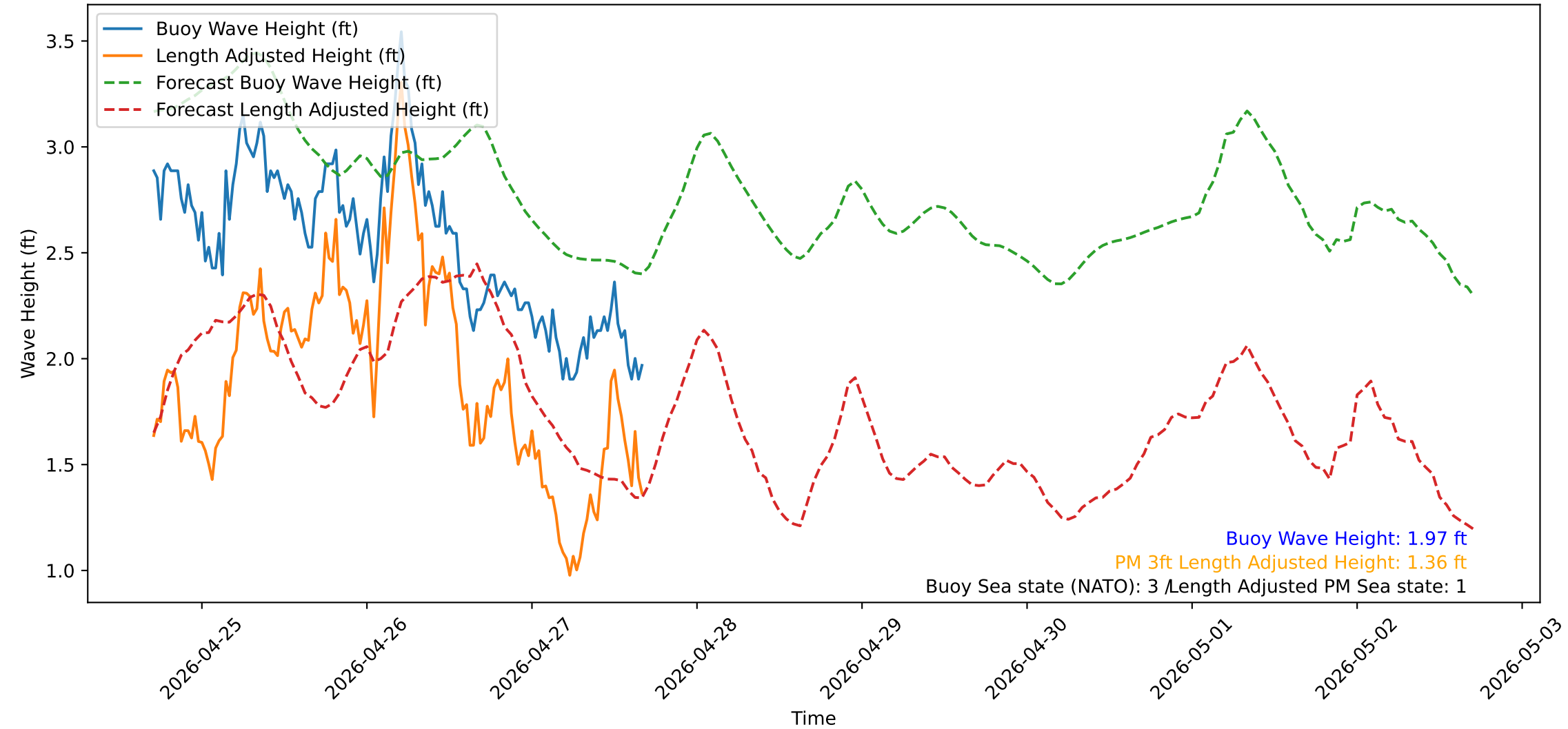
Wave Heights over Time for Red Beach at 2026-04-27 16:50:51
