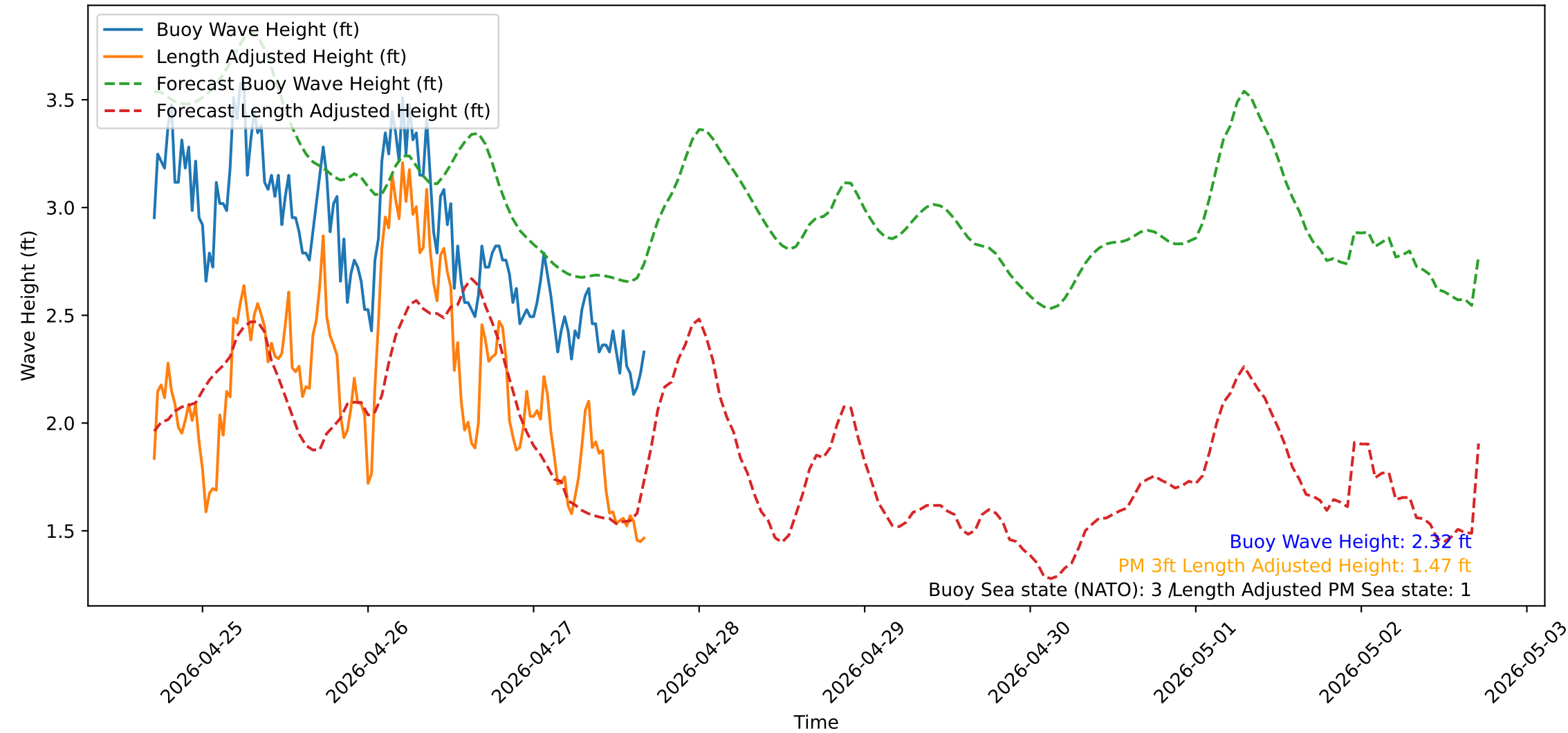
Wave Heights over Time for Green Beach at 2026-04-27 16:51:13
