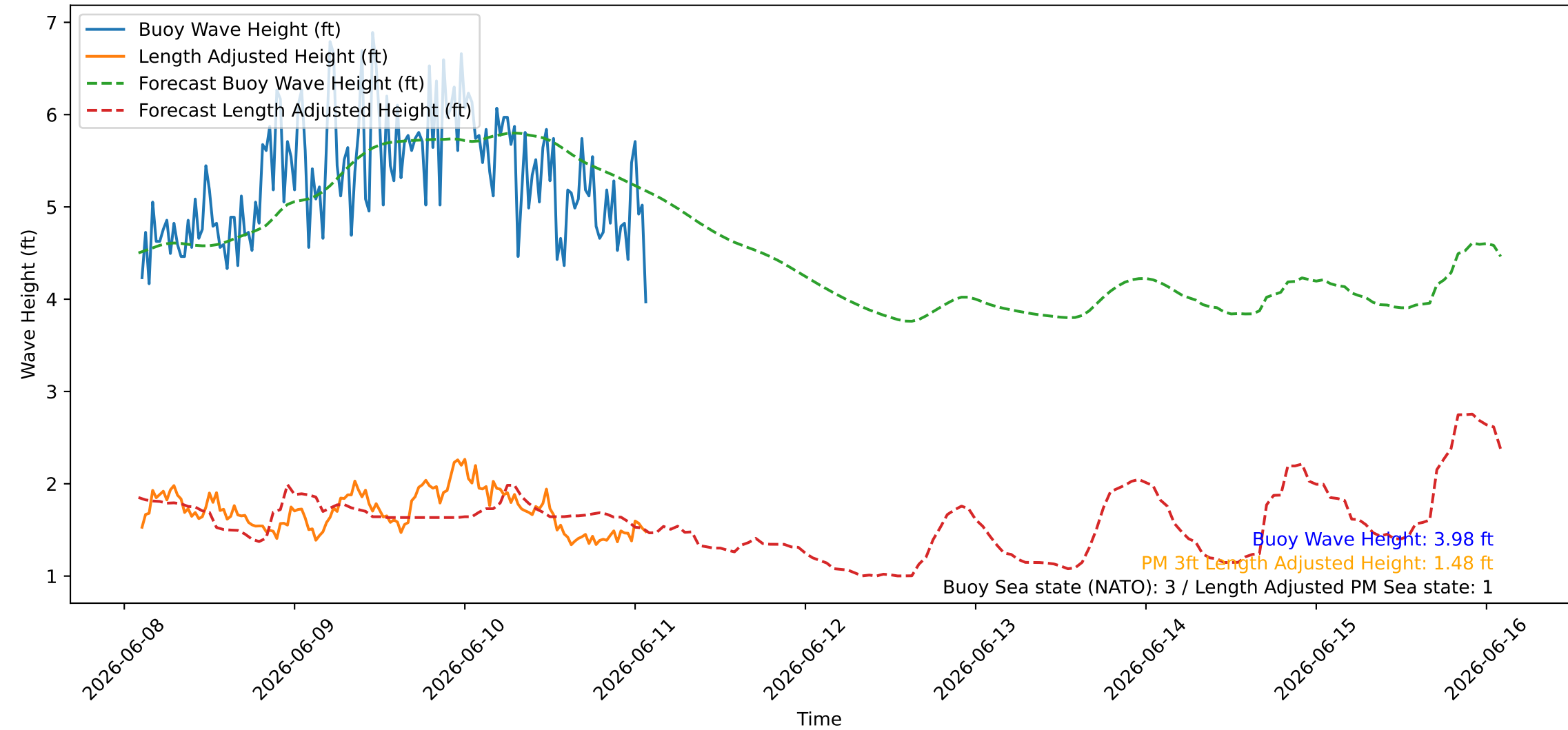
Wave Heights over Time for Green Beach at 2026-06-11 02:21:12
