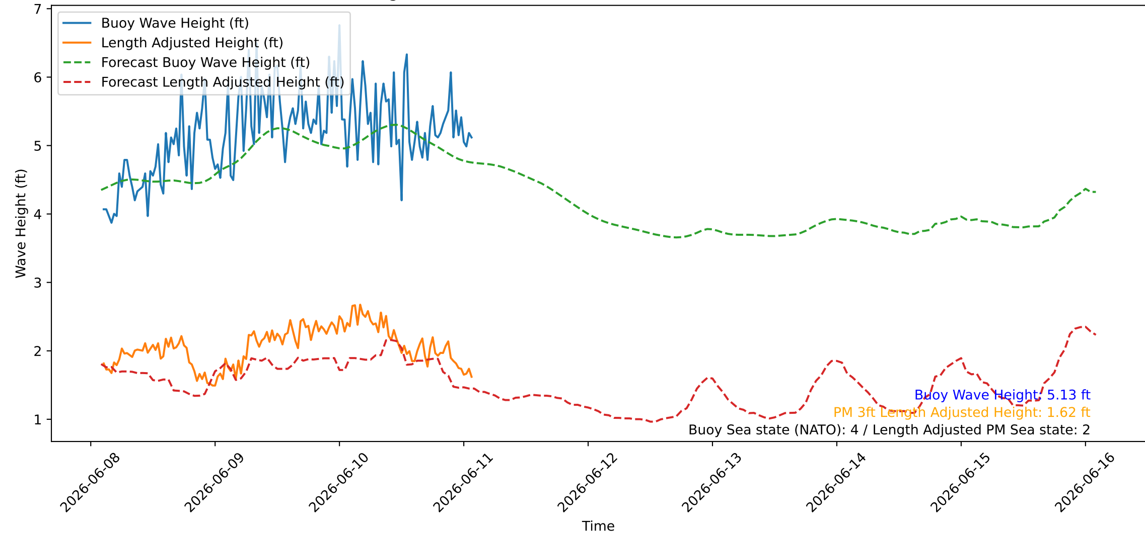
Wave Heights over Time for Oceanside Harbor at 2026-06-11 02:20:27
