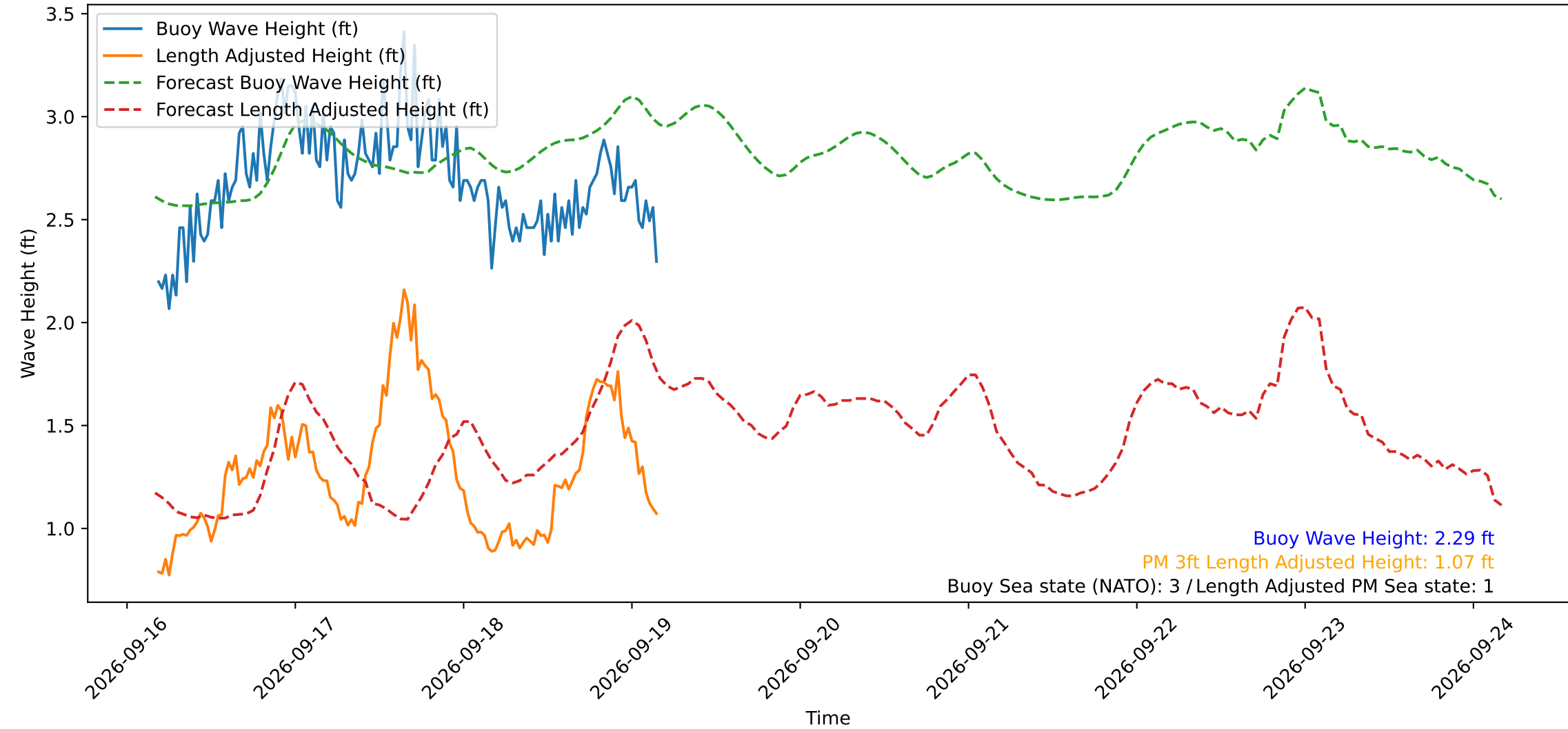
Wave Heights over Time for Red Beach at 2026-09-19 04:10:49
