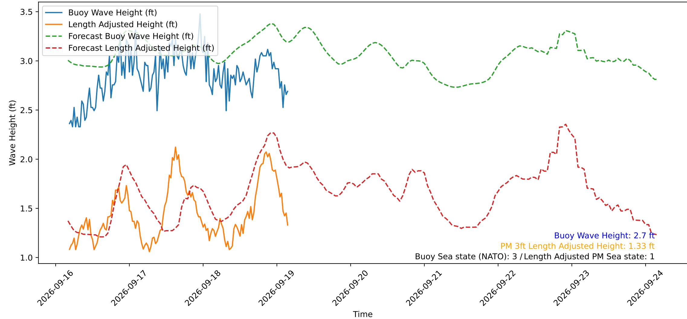
Wave Heights over Time for Green Beach at 2026-09-19 04:11:11
