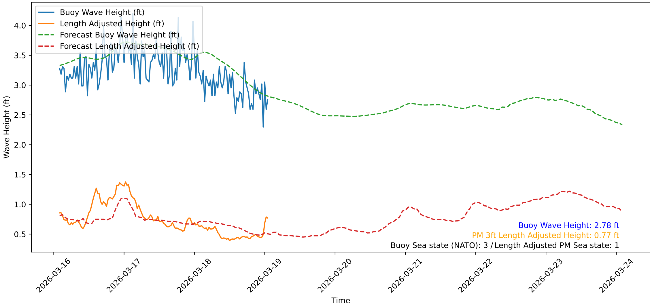
Wave Heights over Time for Green Beach at 2026-03-19 02:01:09
