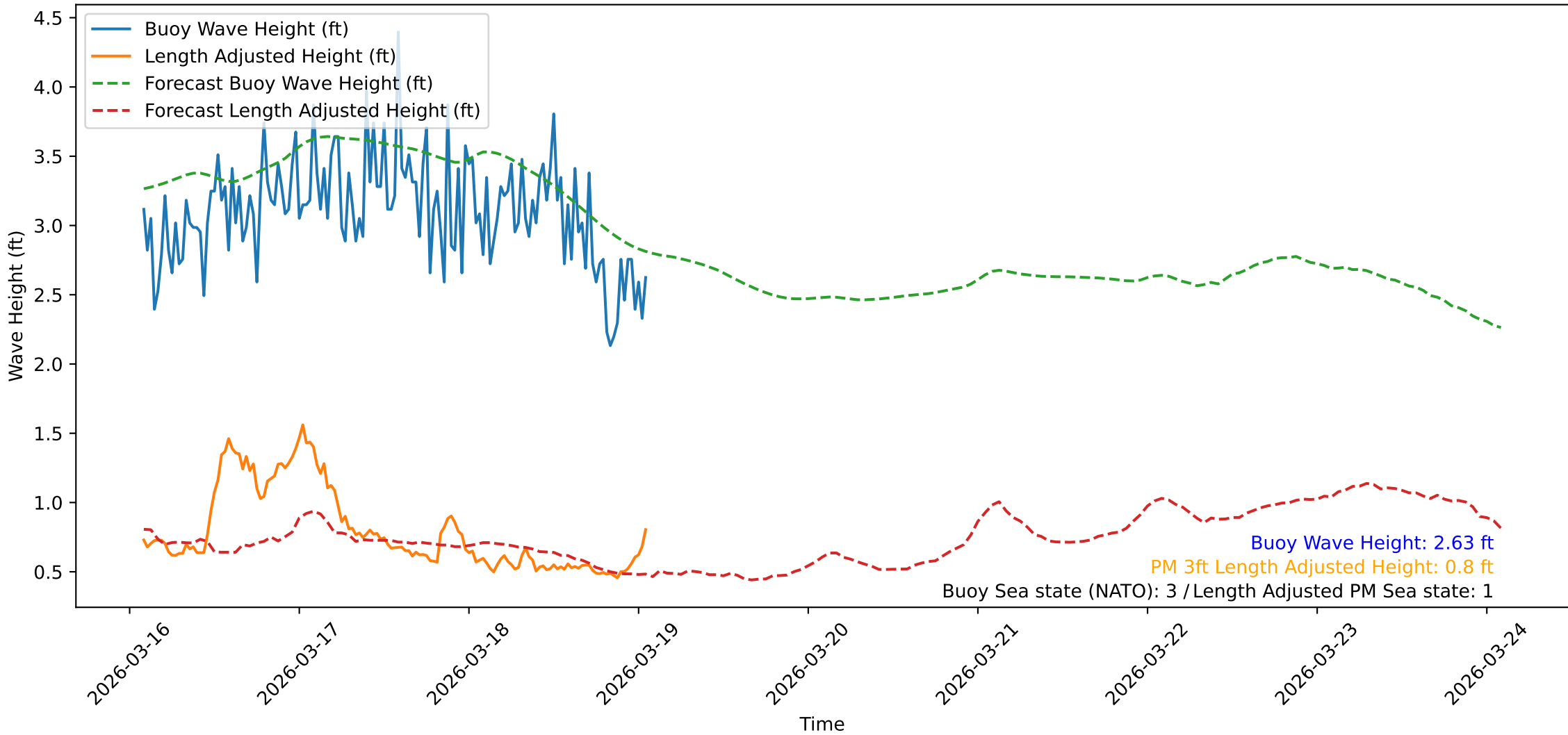
Wave Heights over Time for Oceanside Harbor at 2026-03-19 02:00:31
