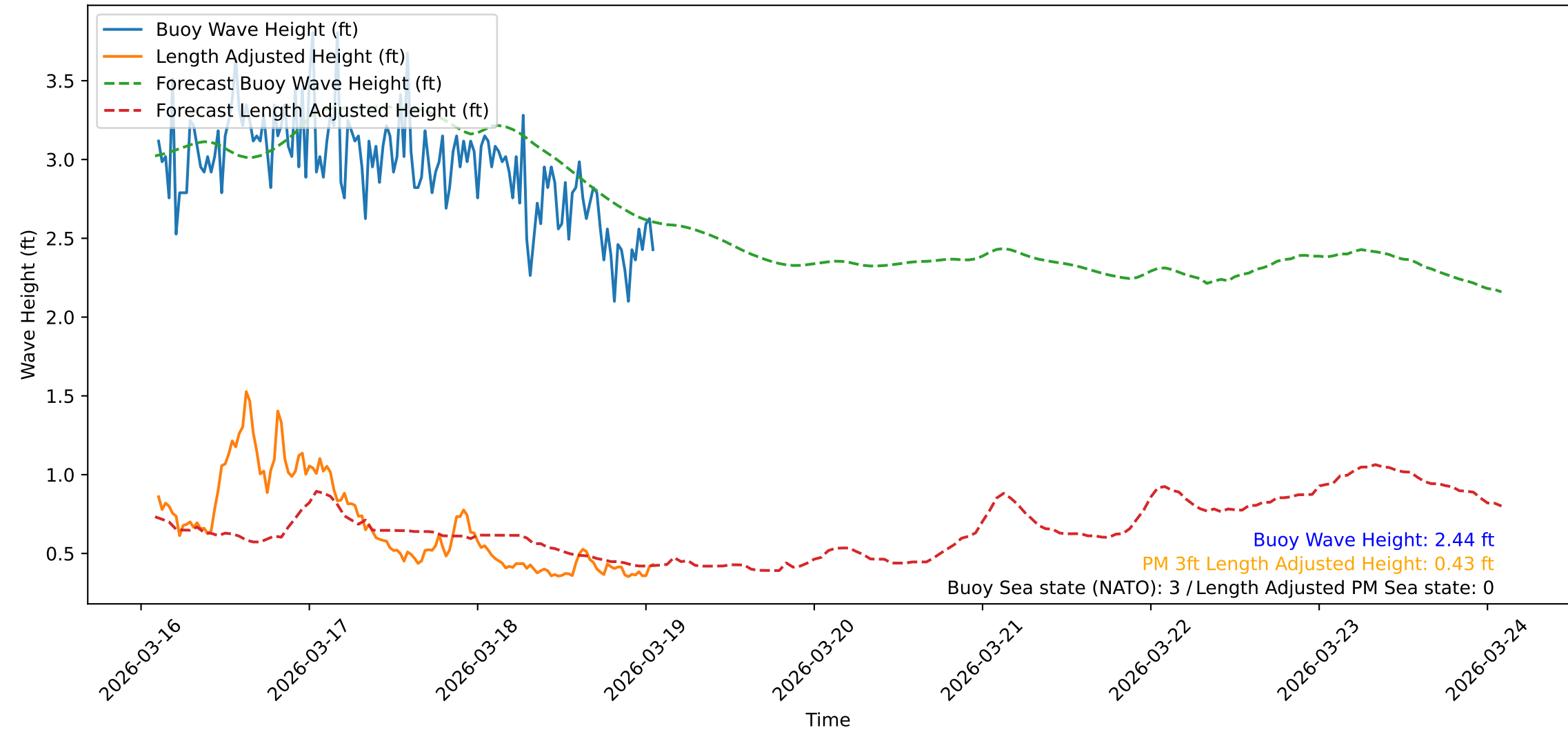
Wave Heights over Time for Red Beach at 2026-03-19 02:00:47
