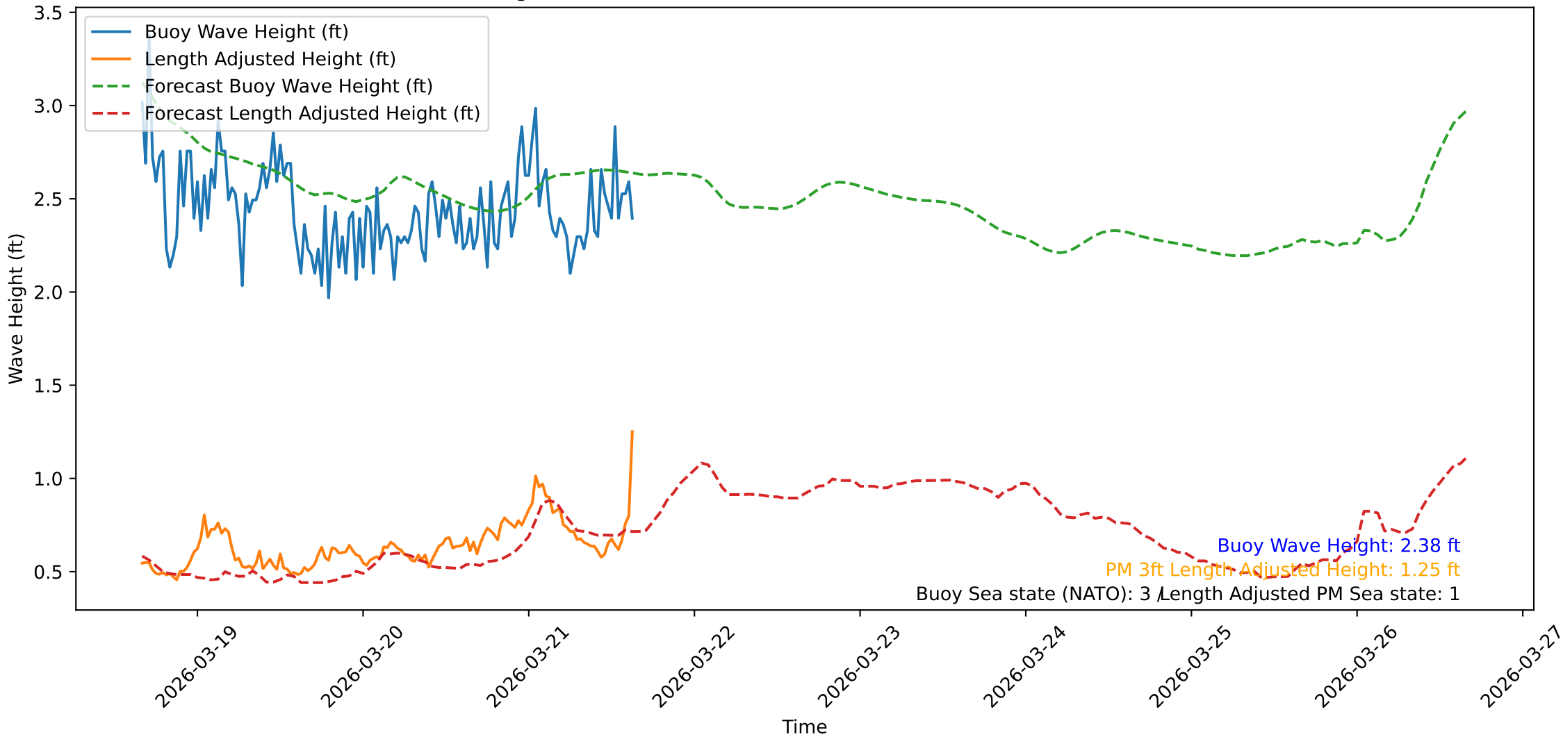
Wave Heights over Time for Oceanside Harbor at 2026-03-21 15:50:31
