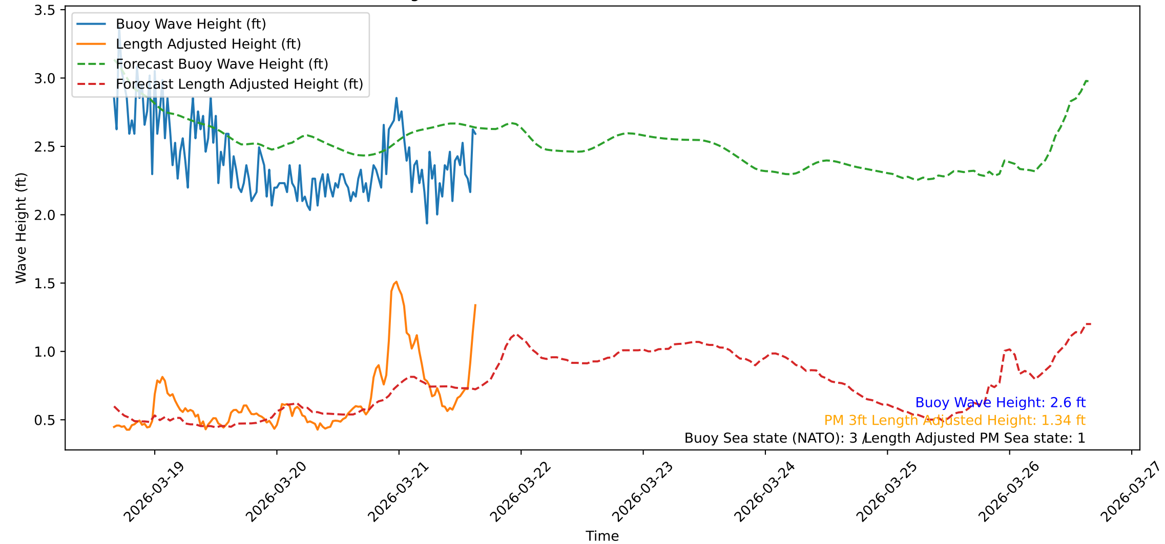
Wave Heights over Time for Green Beach at 2026-03-21 15:51:09
