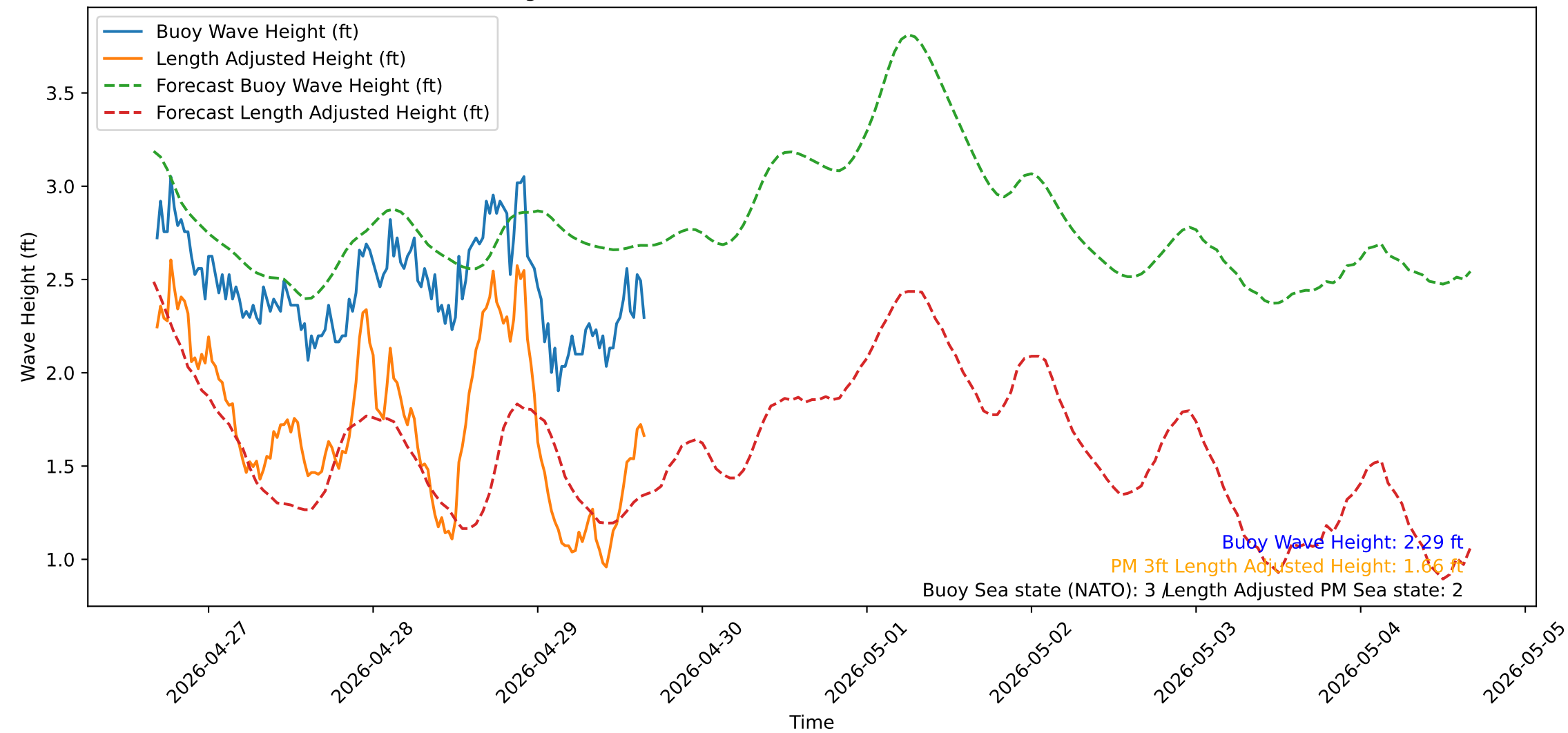
Wave Heights over Time for Oceanside Harbor at 2026-04-29 16:20:32
