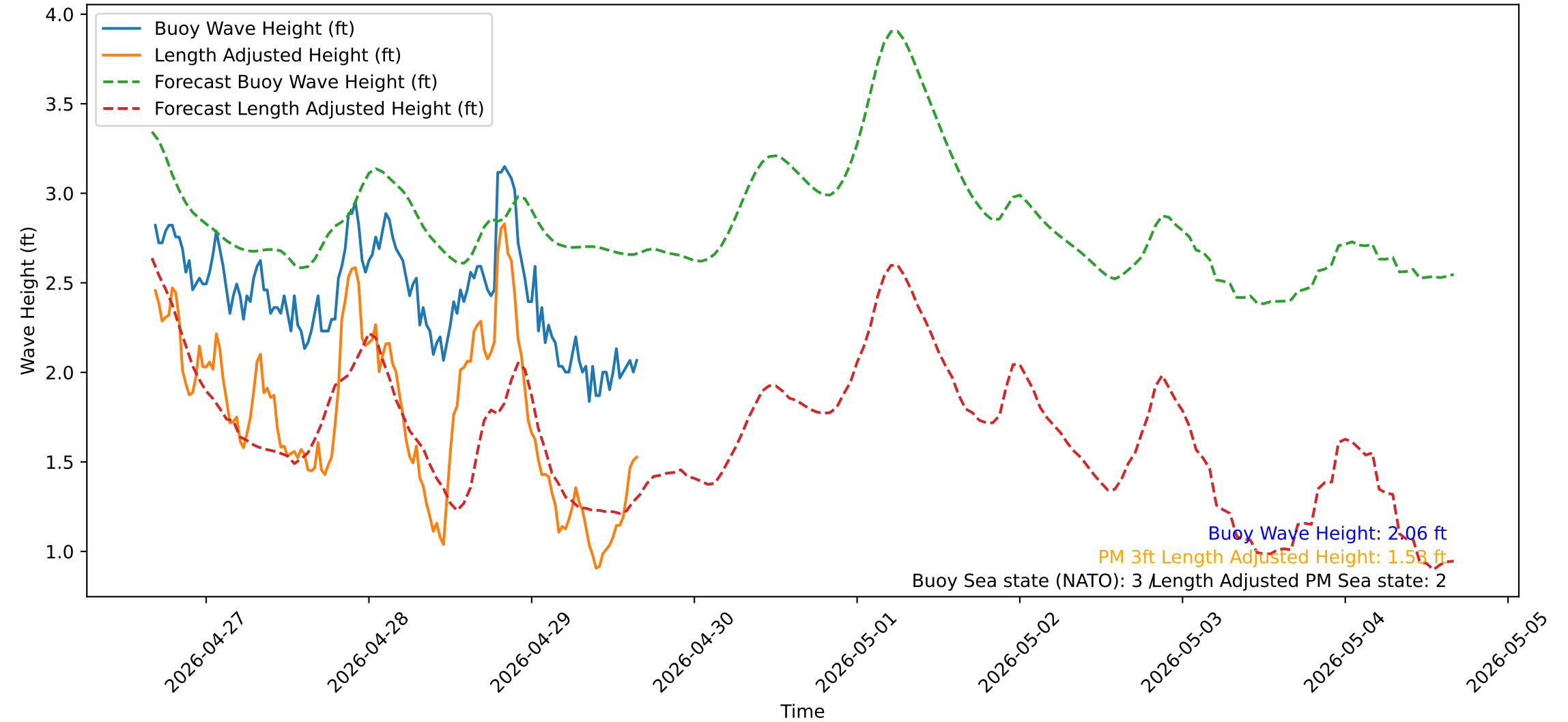
Wave Heights over Time for Green Beach at 2026-04-29 16:21:14
