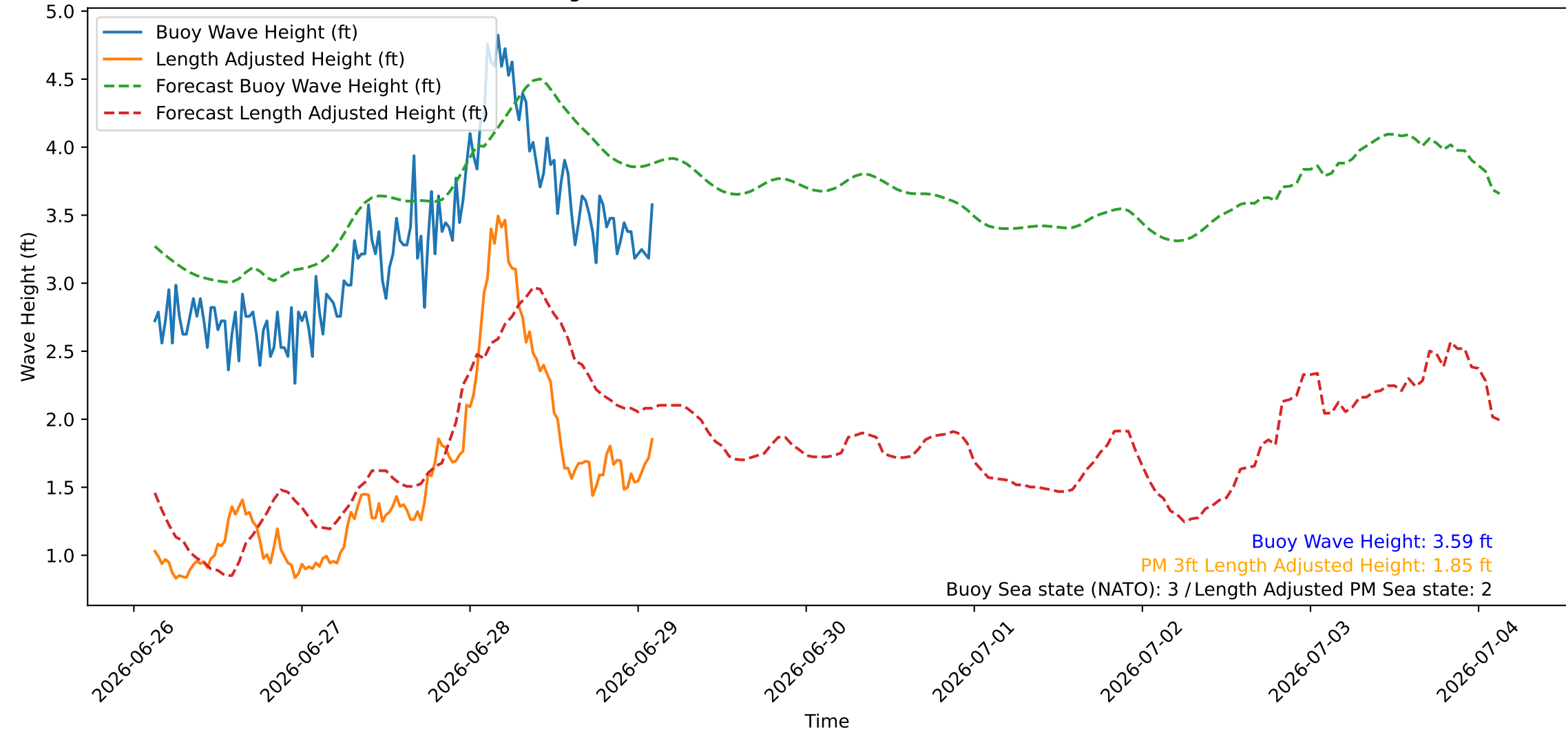
Wave Heights over Time for Green Beach at 2026-06-29 02:51:08
