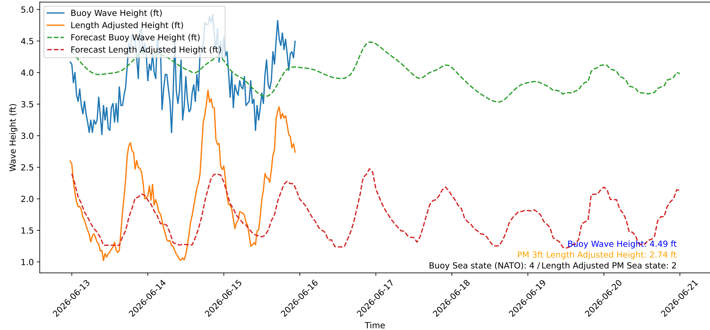
Wave Heights over Time for Green Beach at 2026-06-15 23:31:07
