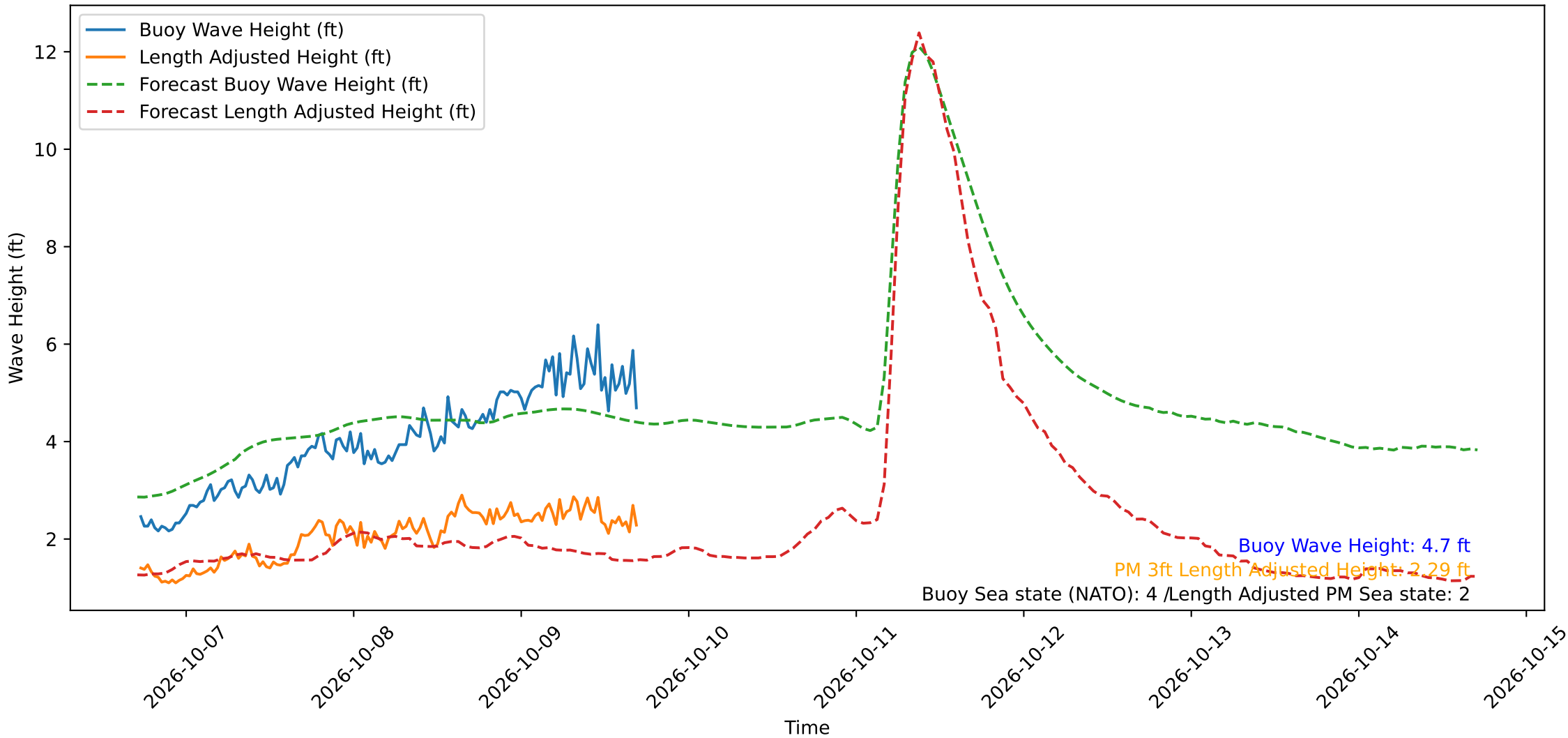
Wave Heights over Time for Oceanside Harbor at 2026-10-09 17:20:29
