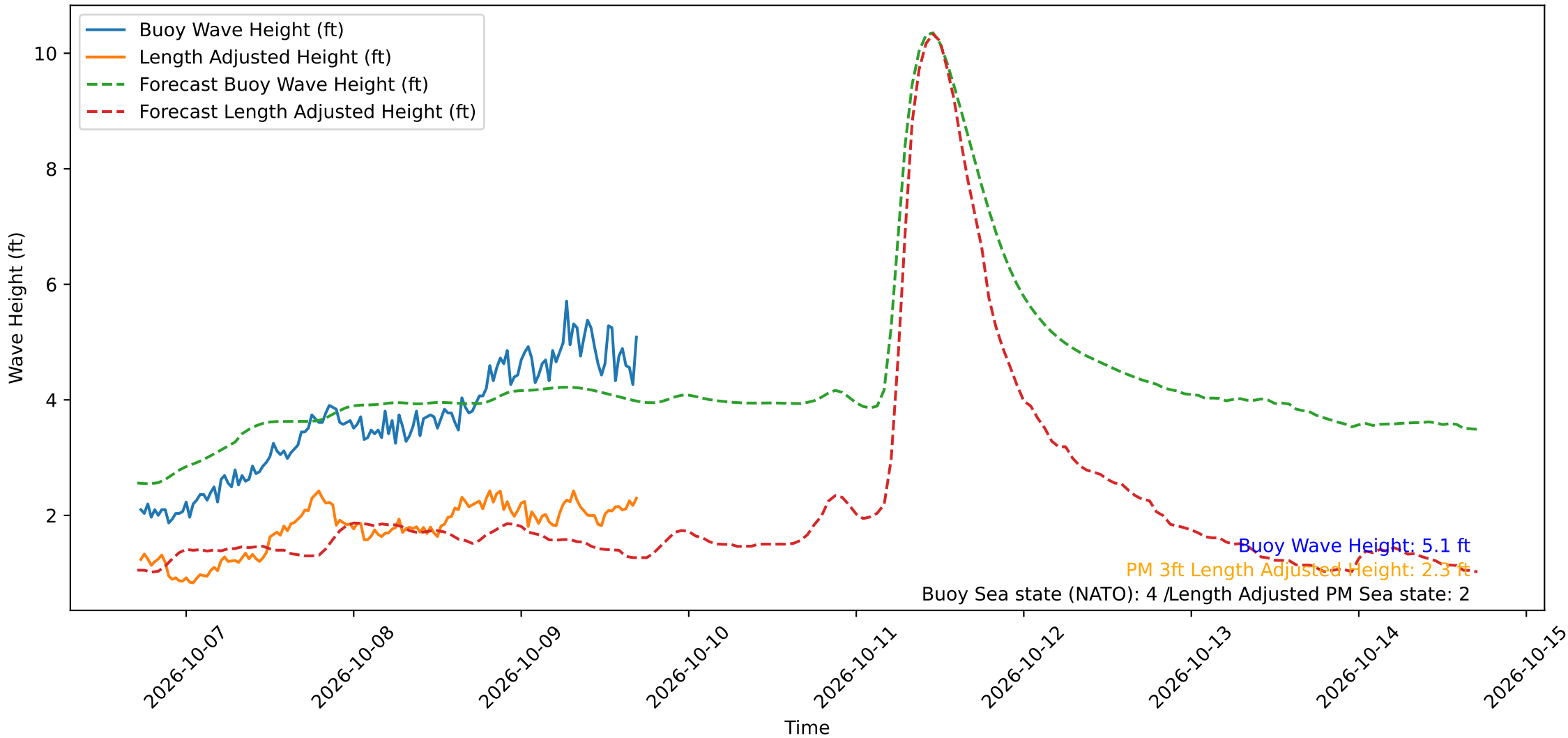
Wave Heights over Time for Red Beach at 2026-10-09 17:20:50
