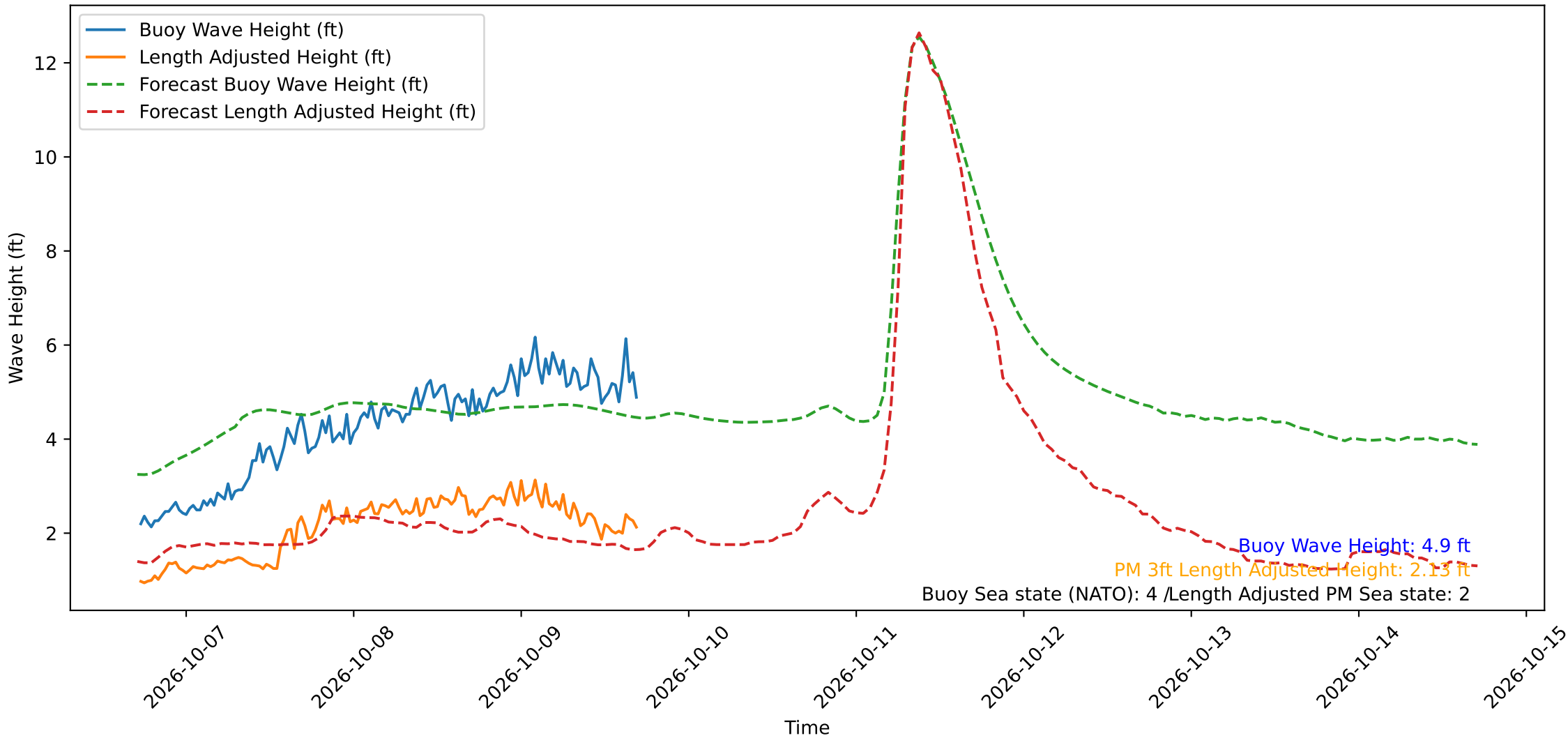
Wave Heights over Time for Green Beach at 2026-10-09 17:21:14
