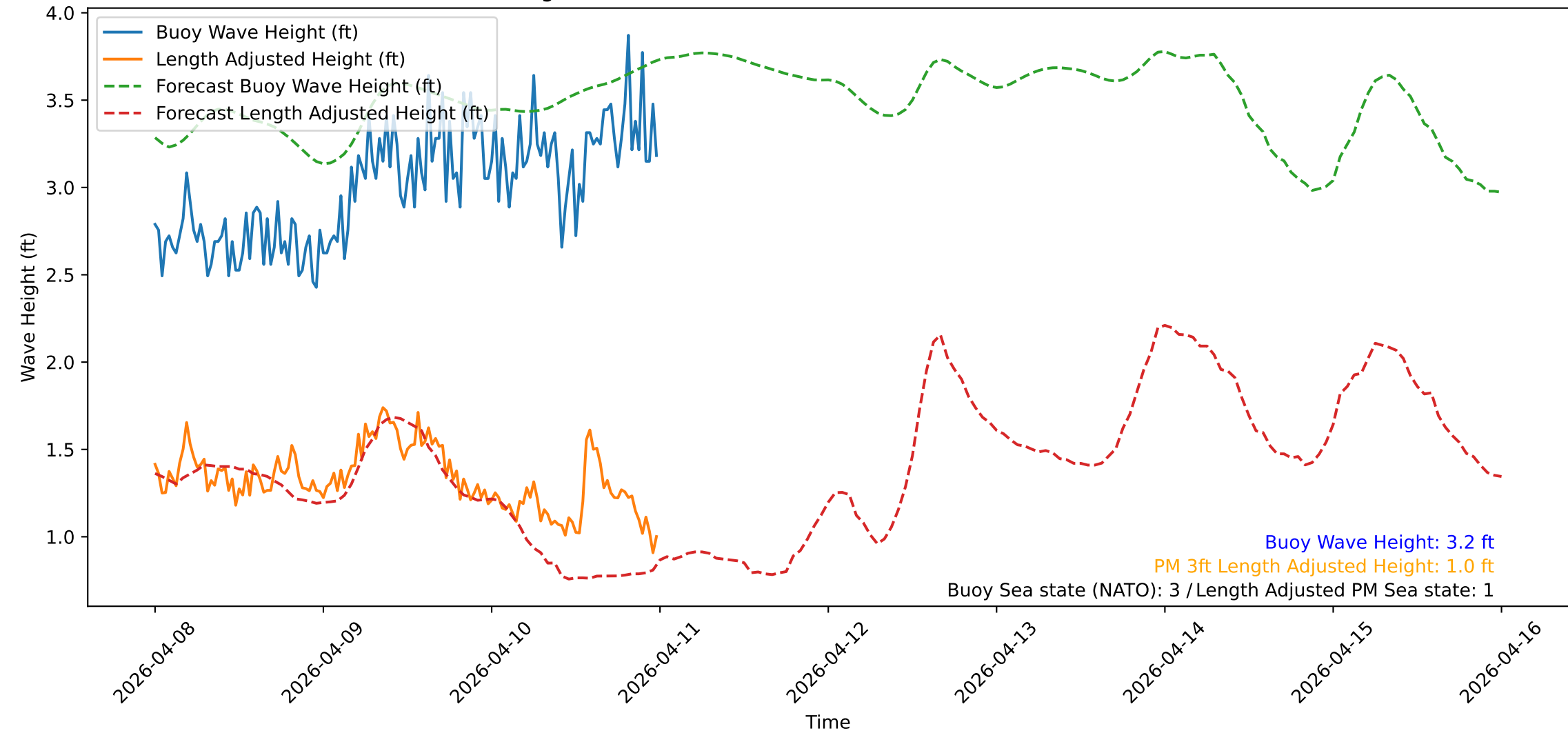
Wave Heights over Time for Oceanside Harbor at 2026-04-11 00:00:31
