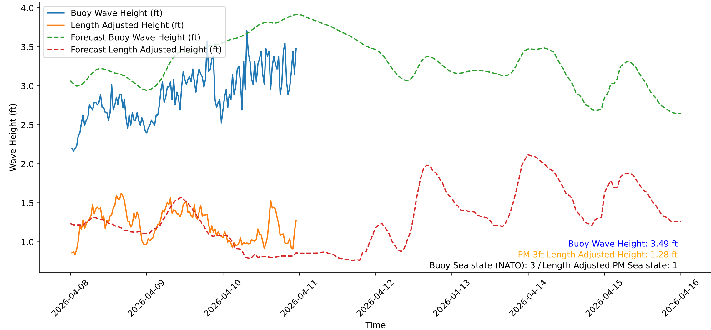
Wave Heights over Time for Red Beach at 2026-04-11 00:00:51
