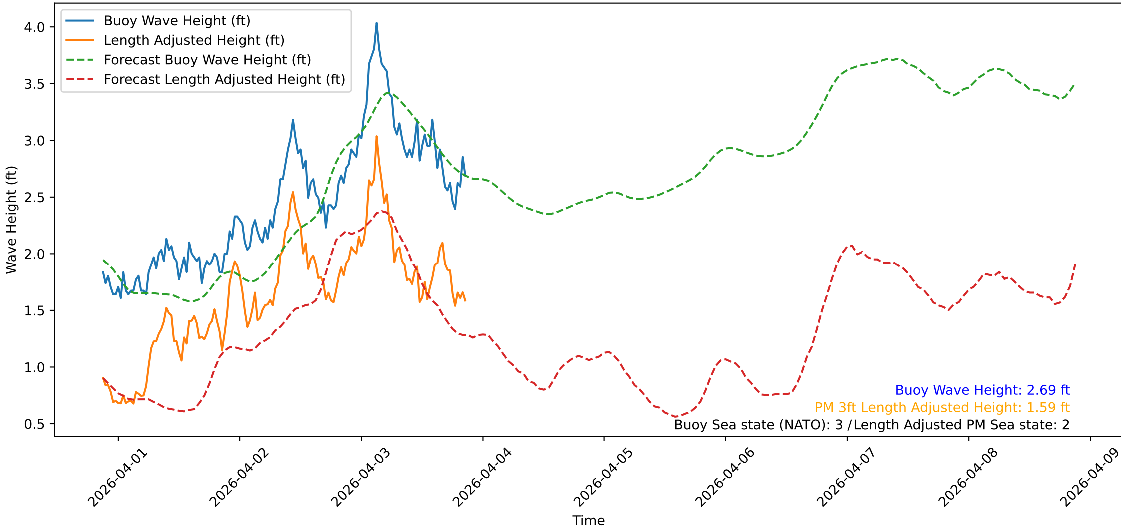
Wave Heights over Time for Oceanside Harbor at 2026-04-03 21:10:37
