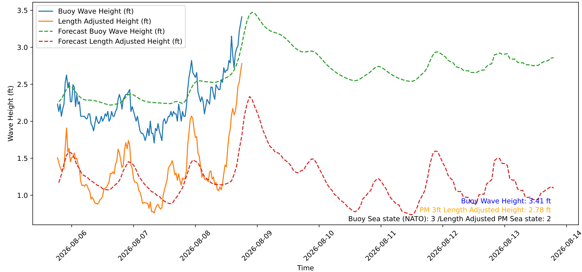
Wave Heights over Time for Green Beach at 2026-08-08 18:41:08
