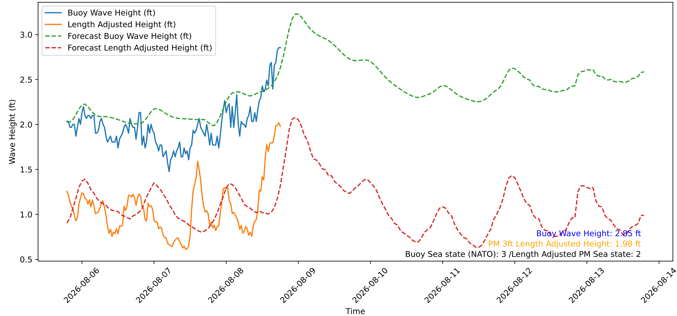
Wave Heights over Time for Red Beach at 2026-08-08 18:40:46
