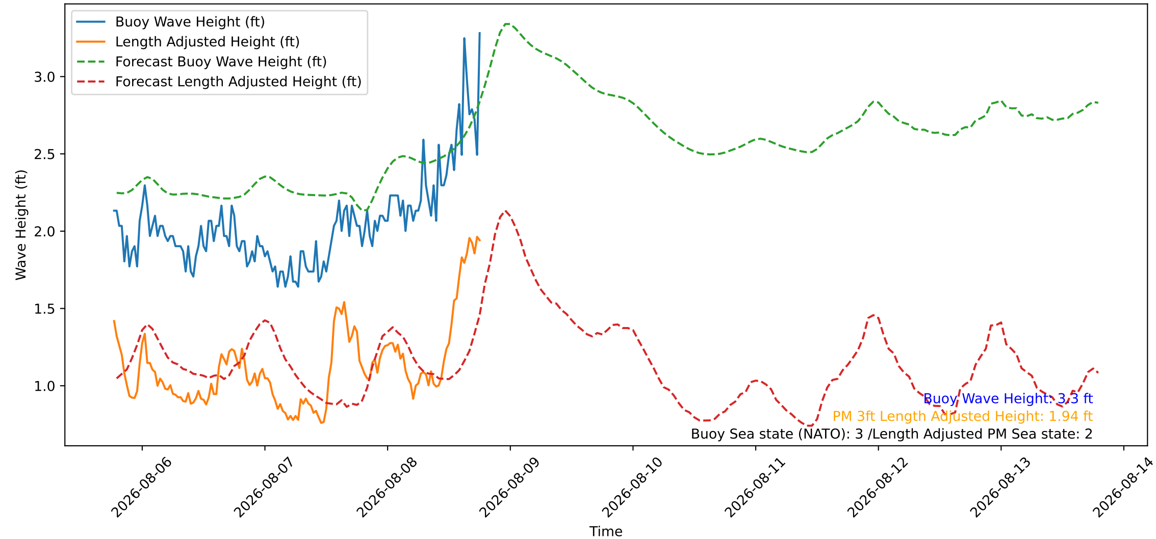
Wave Heights over Time for Oceanside Harbor at 2026-08-08 18:40:26
