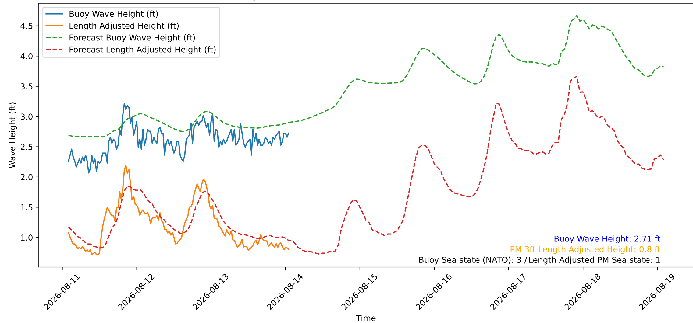
Wave Heights over Time for Green Beach at 2026-08-14 01:51:09
