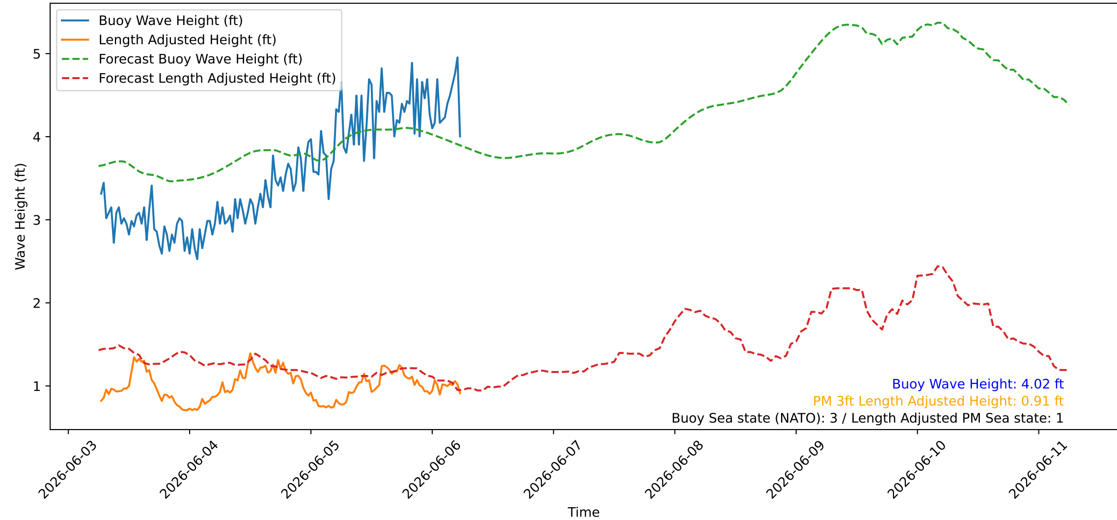
Wave Heights over Time for Red Beach at 2026-06-06 06:10:45
