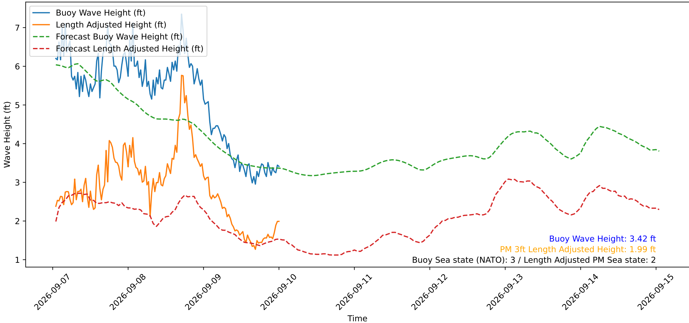
Wave Heights over Time for Oceanside Harbor at 2026-09-10 00:50:29
