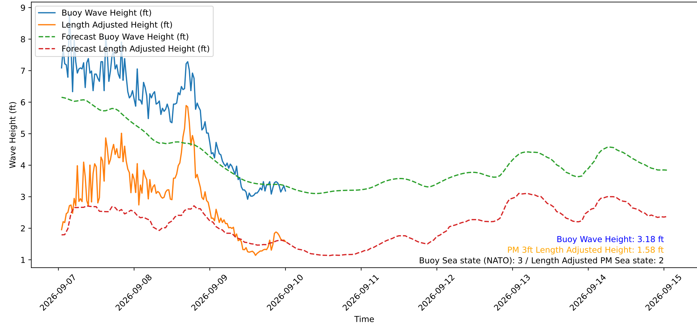
Wave Heights over Time for Green Beach at 2026-09-10 00:51:13
