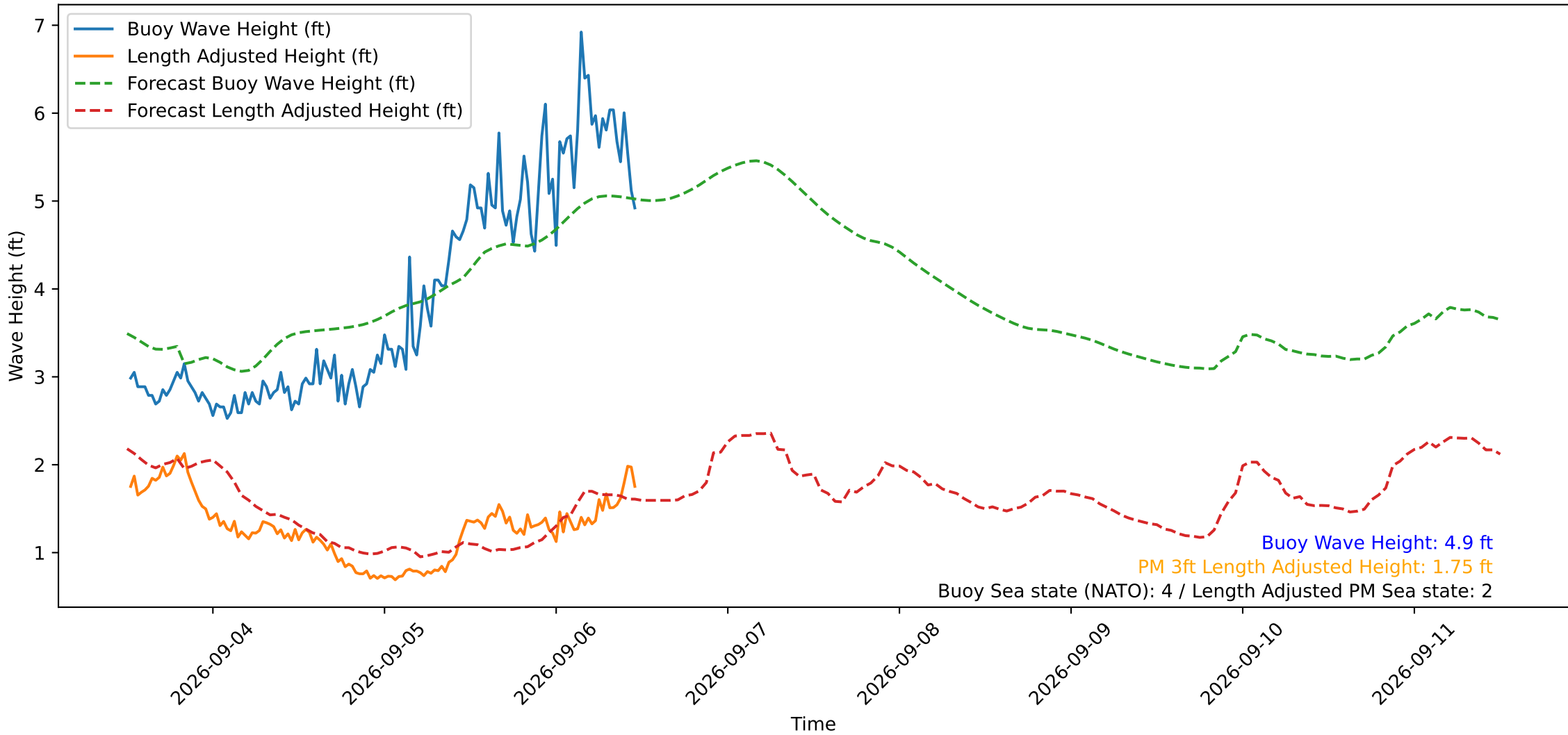
Wave Heights over Time for Red Beach at 2026-09-06 12:00:50
