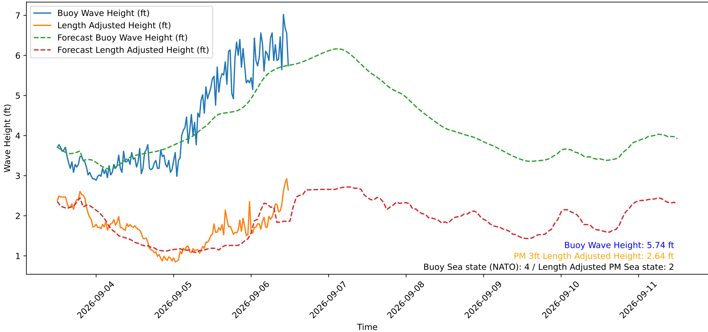
Wave Heights over Time for Oceanside Harbor at 2026-09-06 12:00:30
