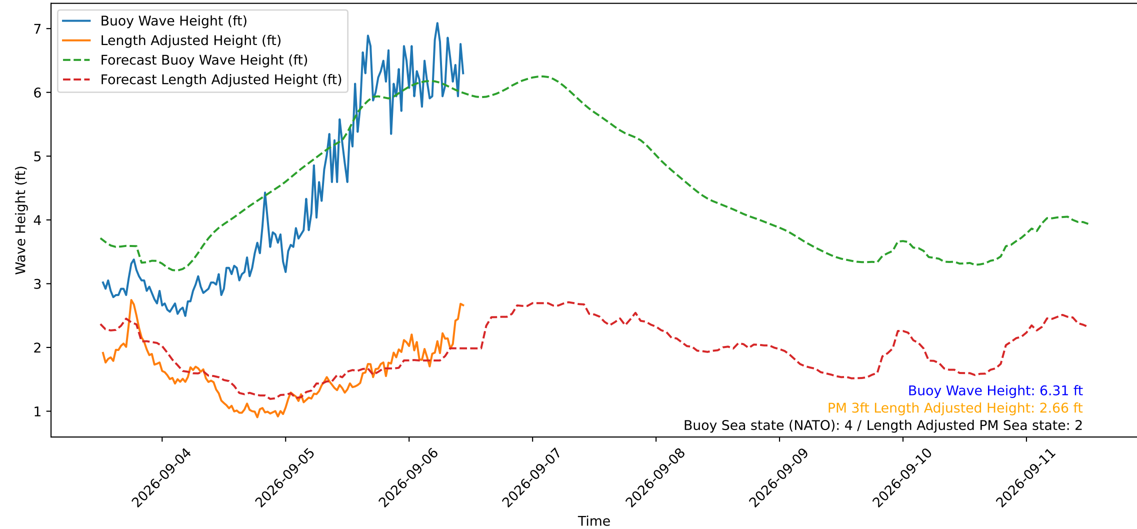
Wave Heights over Time for Green Beach at 2026-09-06 12:01:12
