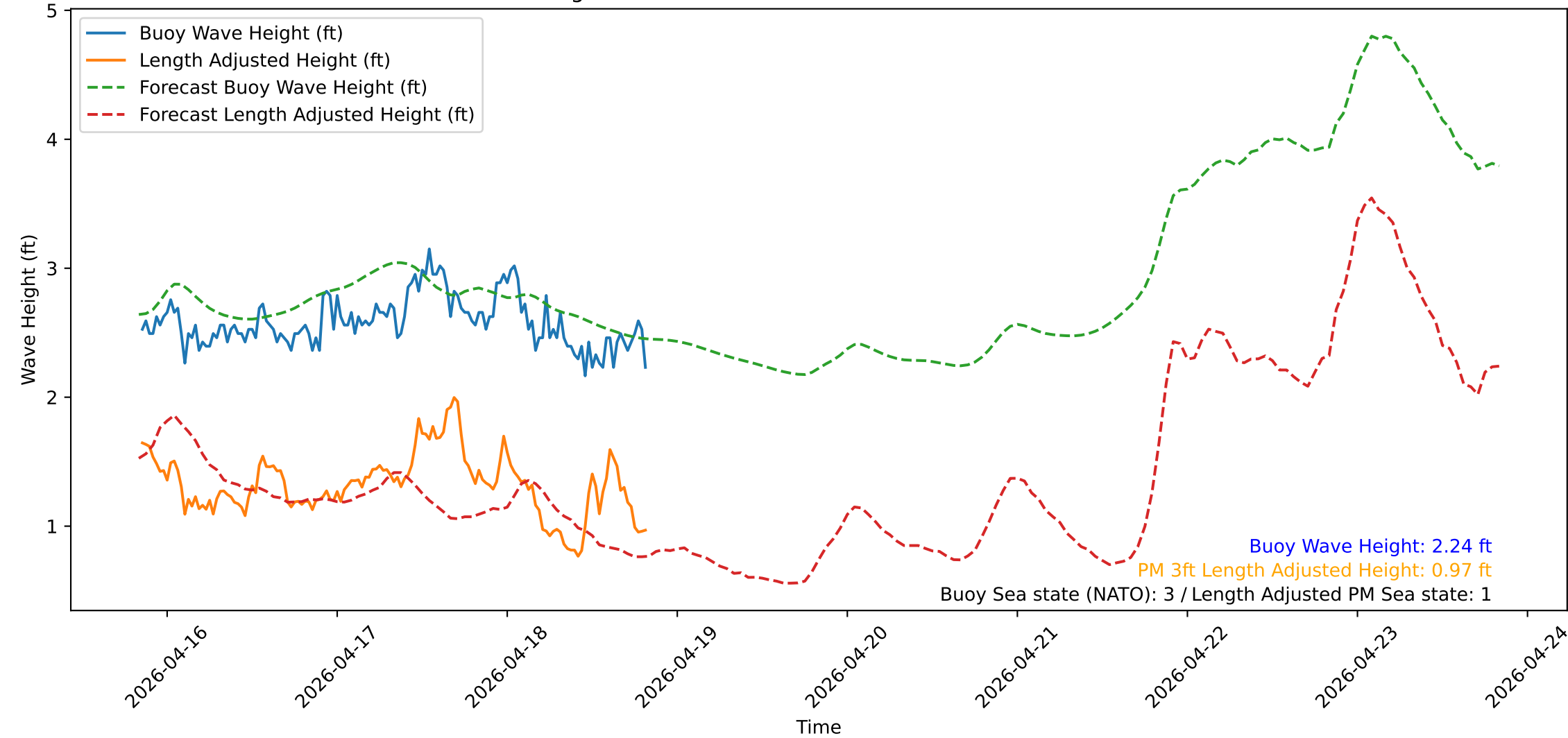
Wave Heights over Time for Red Beach at 2026-04-18 20:10:50
