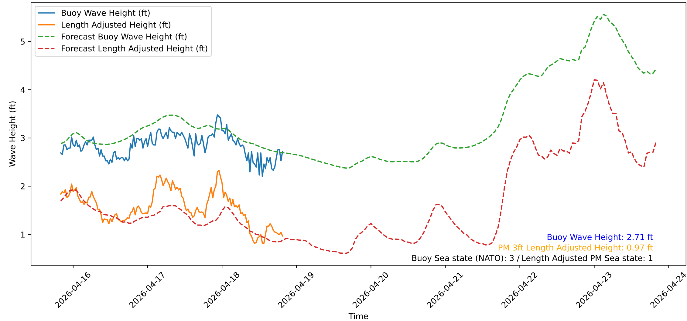
Wave Heights over Time for Green Beach at 2026-04-18 20:11:13
