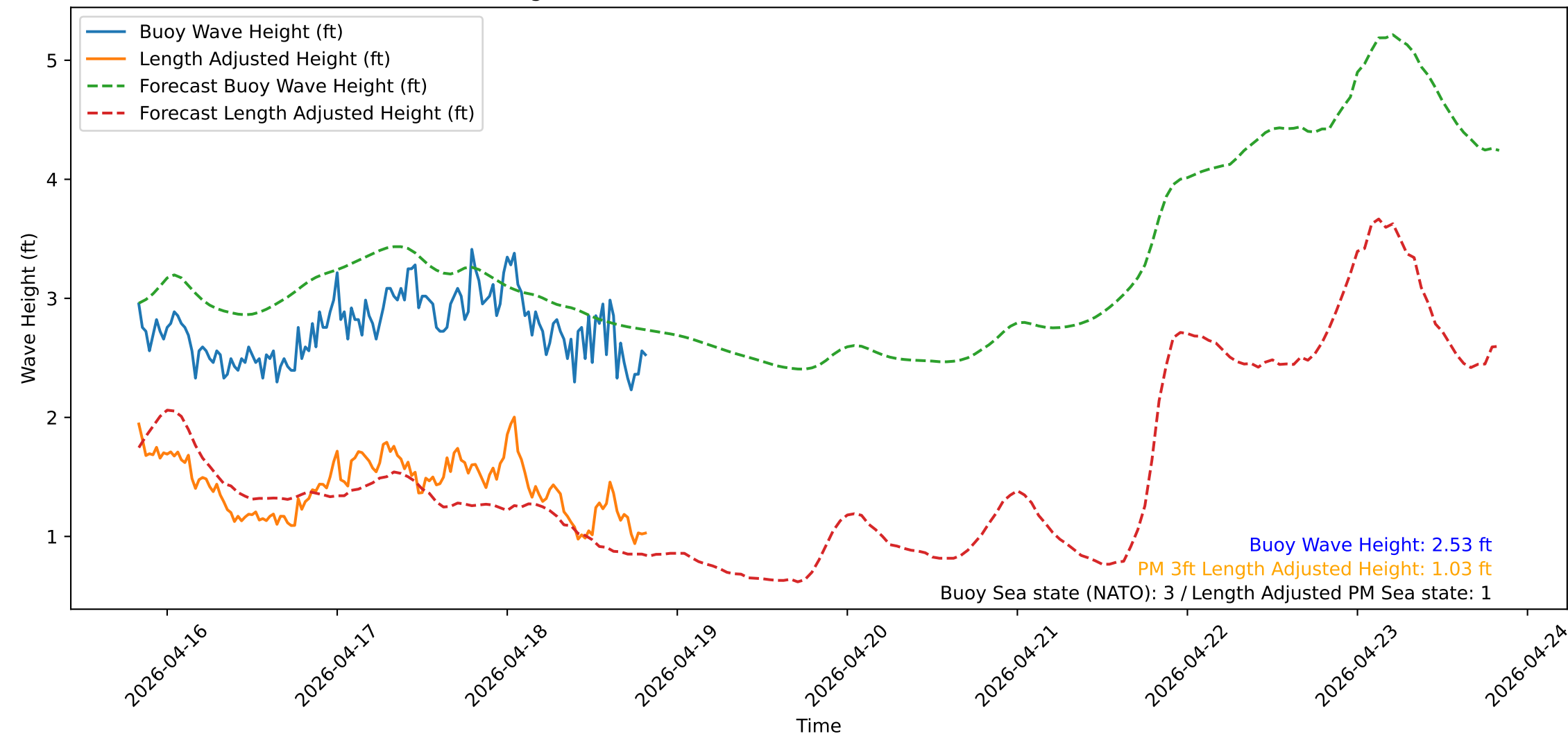
Wave Heights over Time for Oceanside Harbor at 2026-04-18 20:10:31
