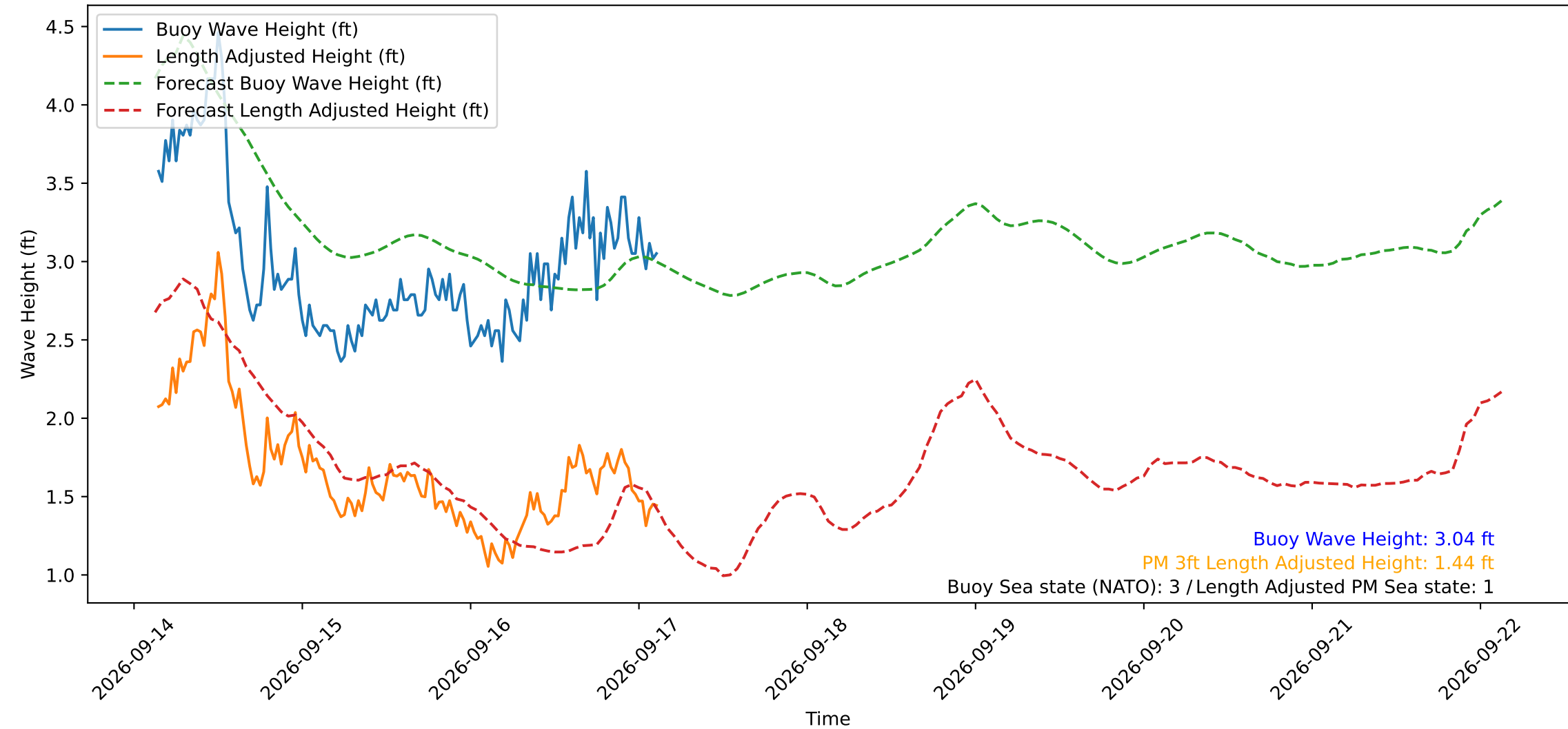
Wave Heights over Time for Oceanside Harbor at 2026-09-17 03:20:29
