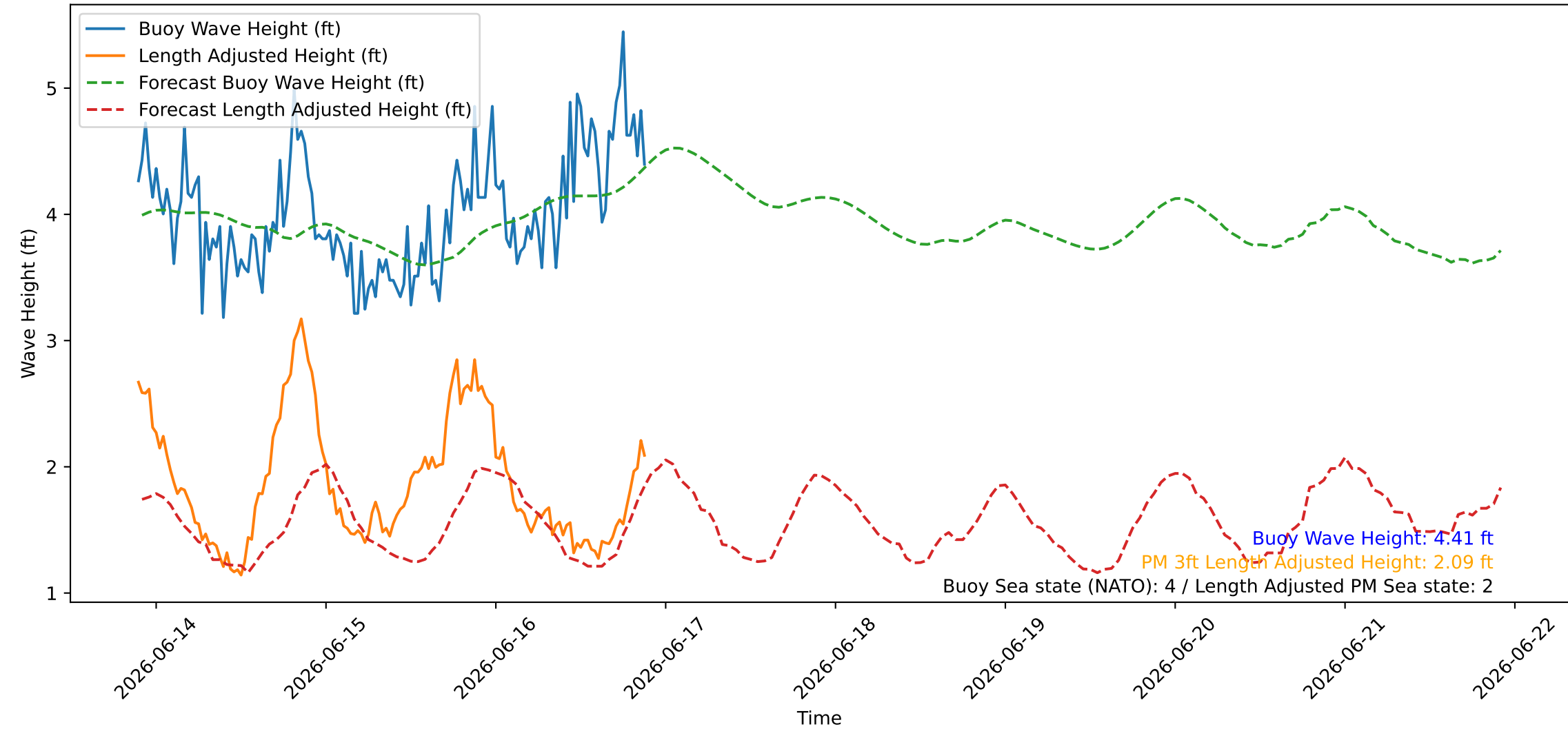
Wave Heights over Time for Oceanside Harbor at 2026-06-16 21:30:27
