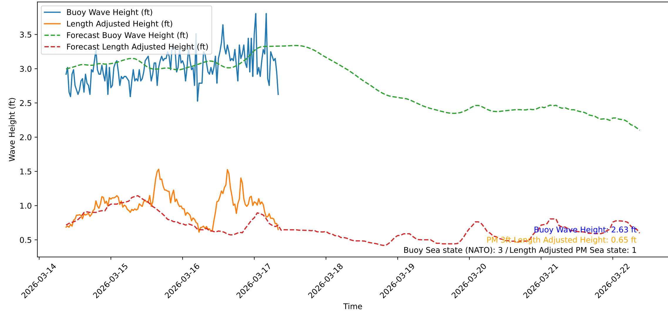
Wave Heights over Time for Red Beach at 2026-03-17 08:51:09
